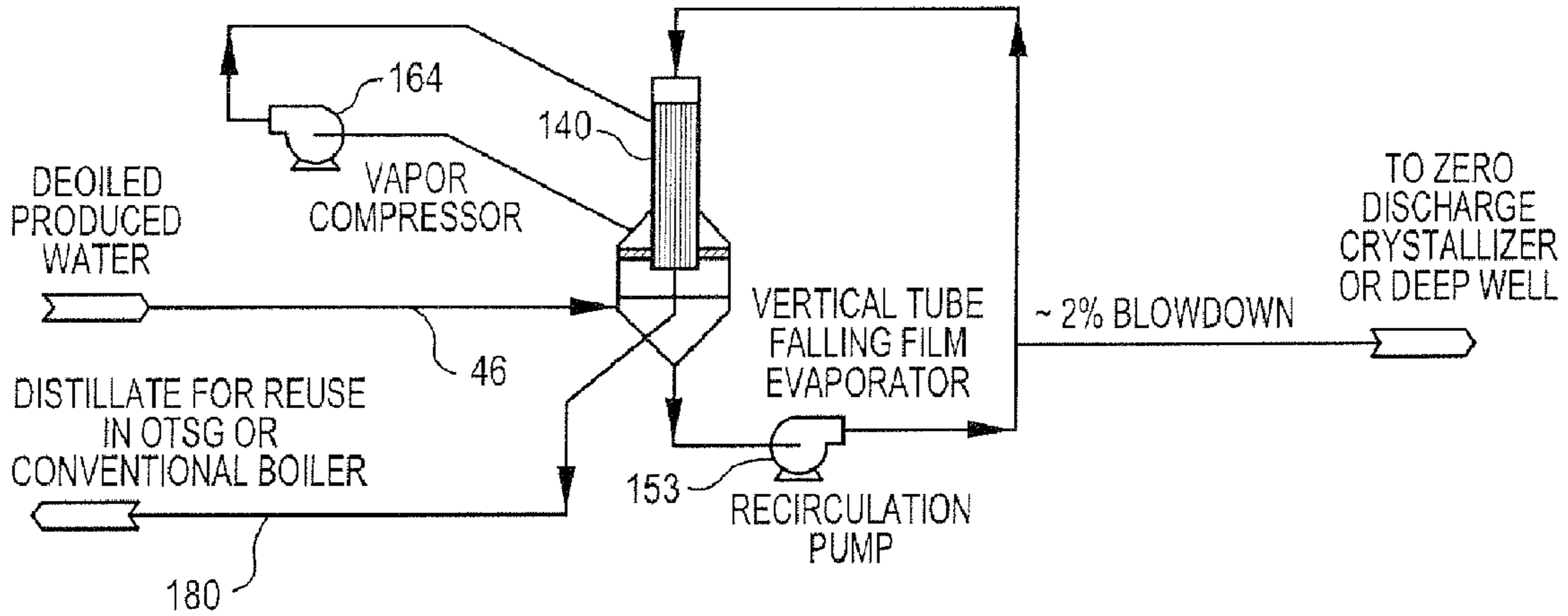
SIMPLIFIED VAPOR COMPRESSION FALLING FILM EVAPORATOR SYSTEM
