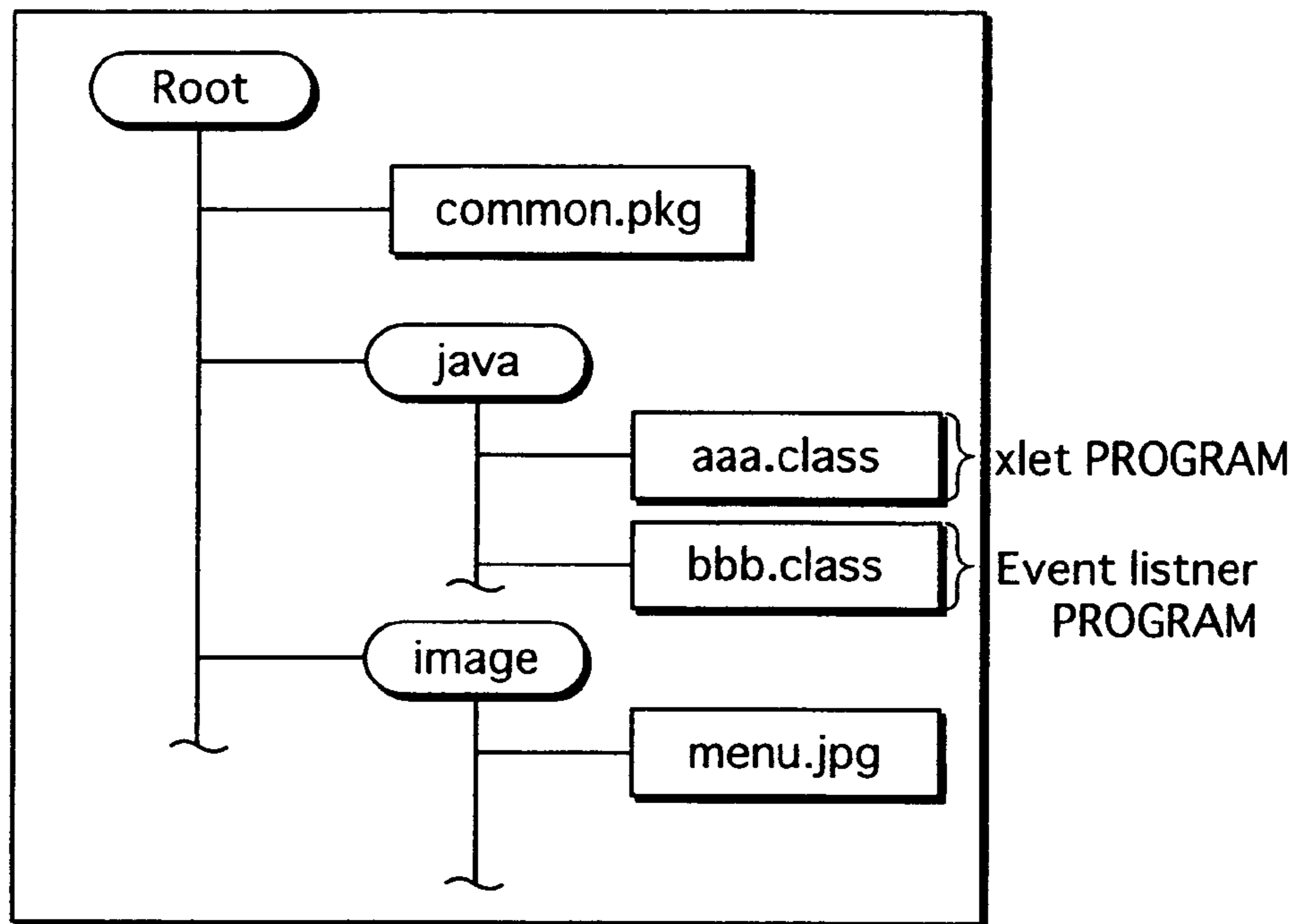
JAR FILE
