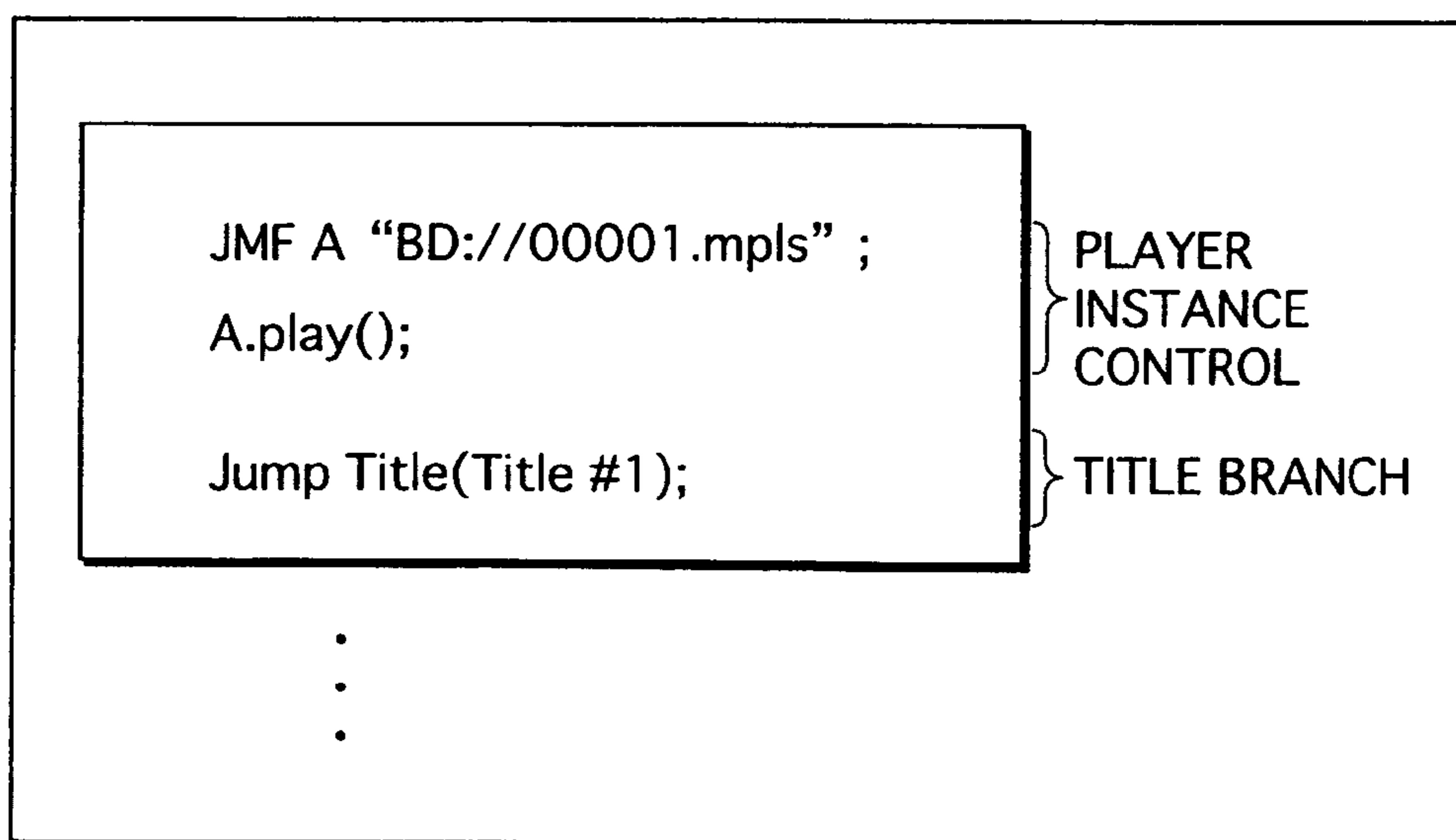
xlet PROGRAM
