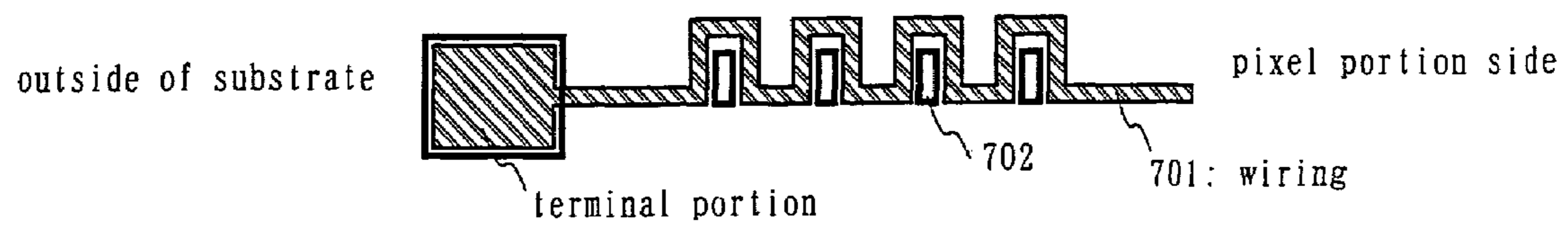
(A) top view
