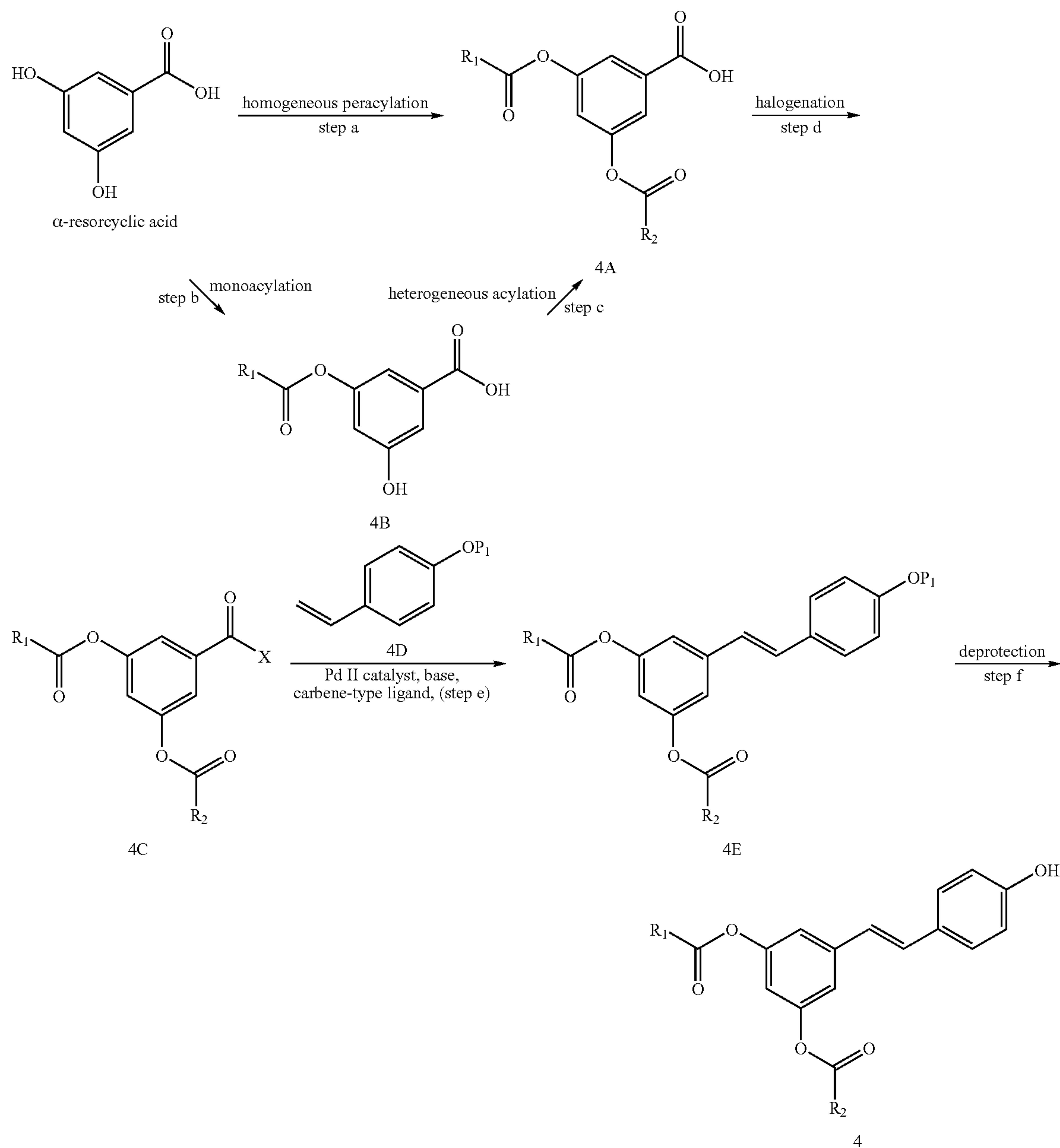
Scheme 5.
