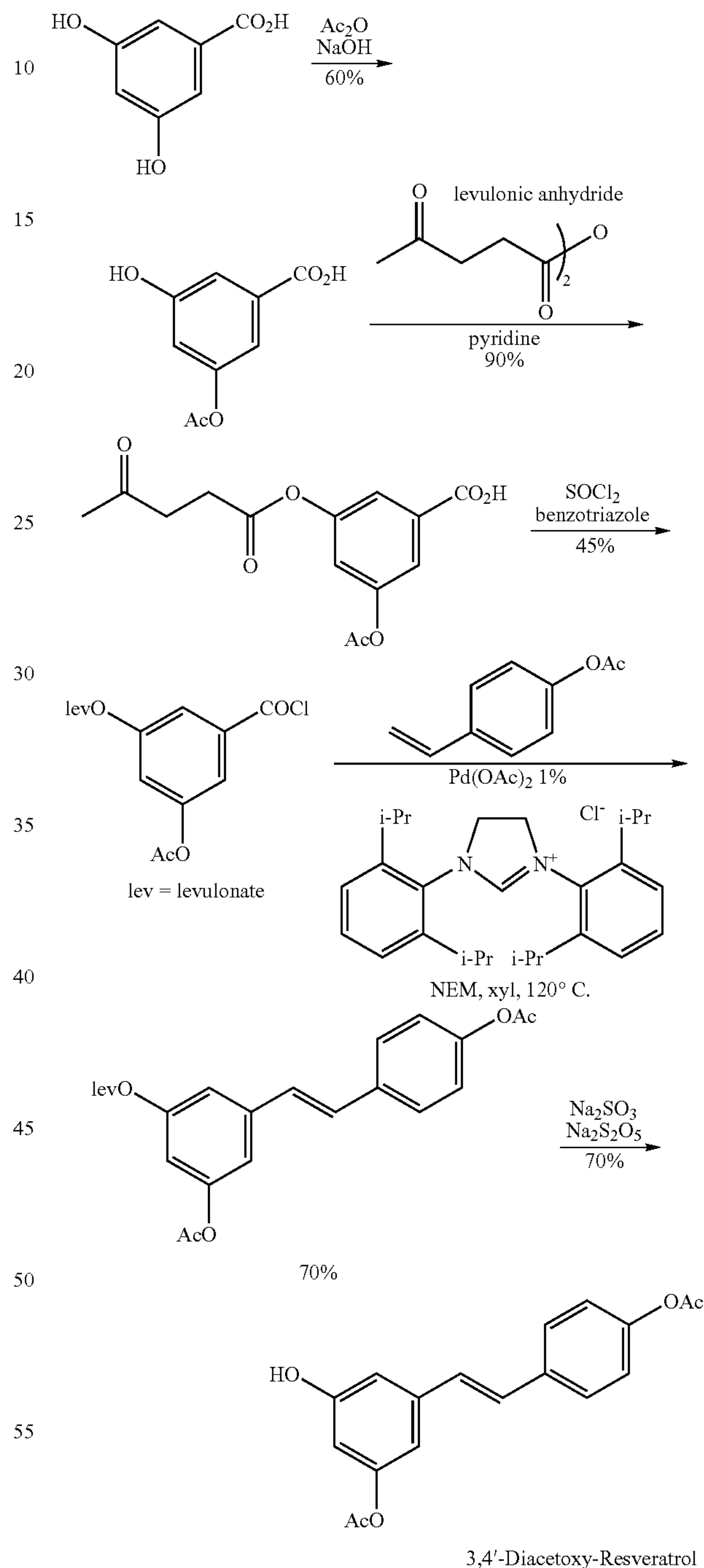
Scheme 13.
