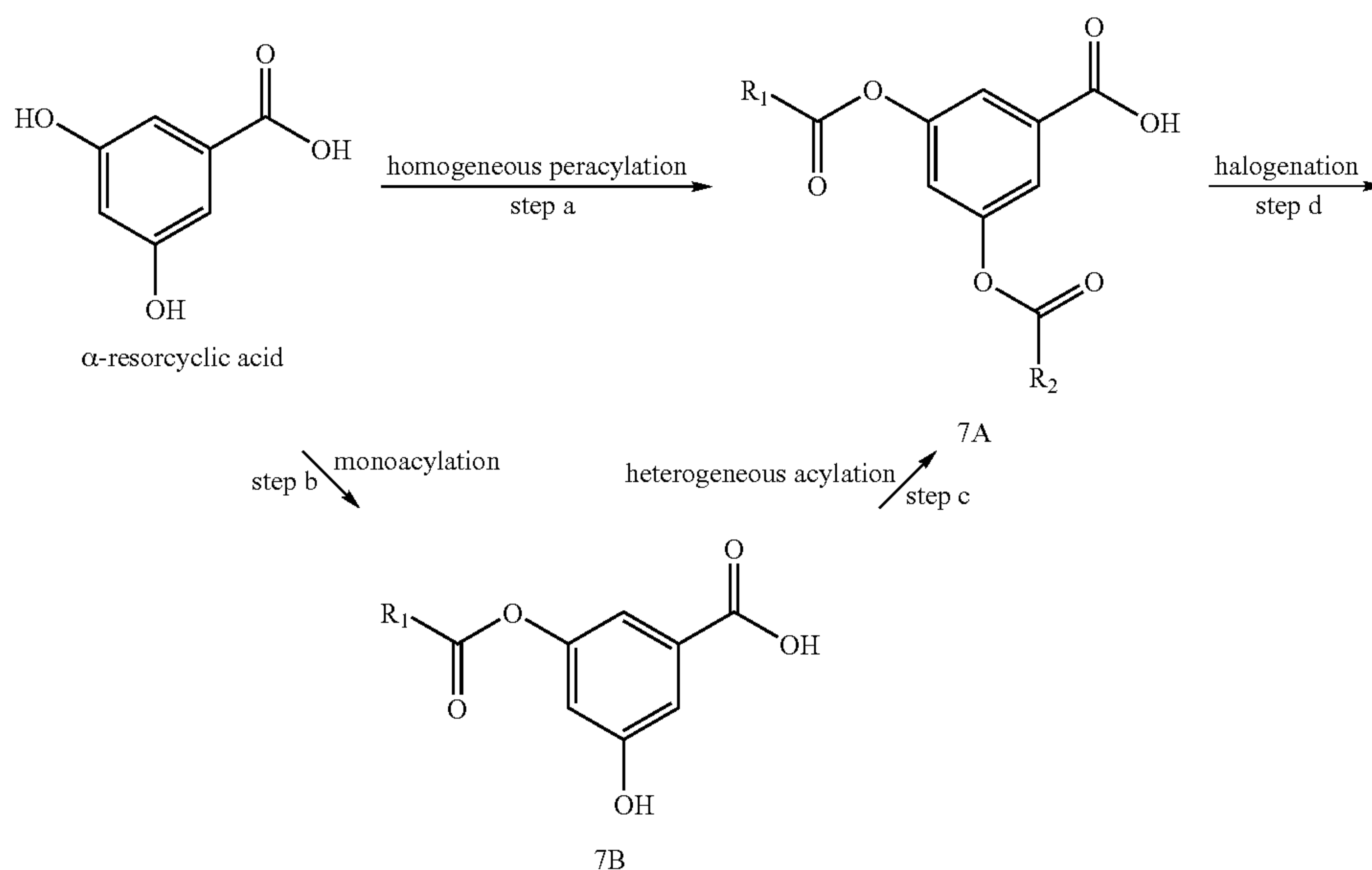
Scheme 8.
