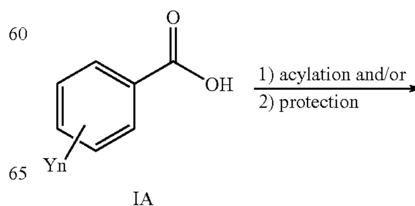
Scheme 9.
