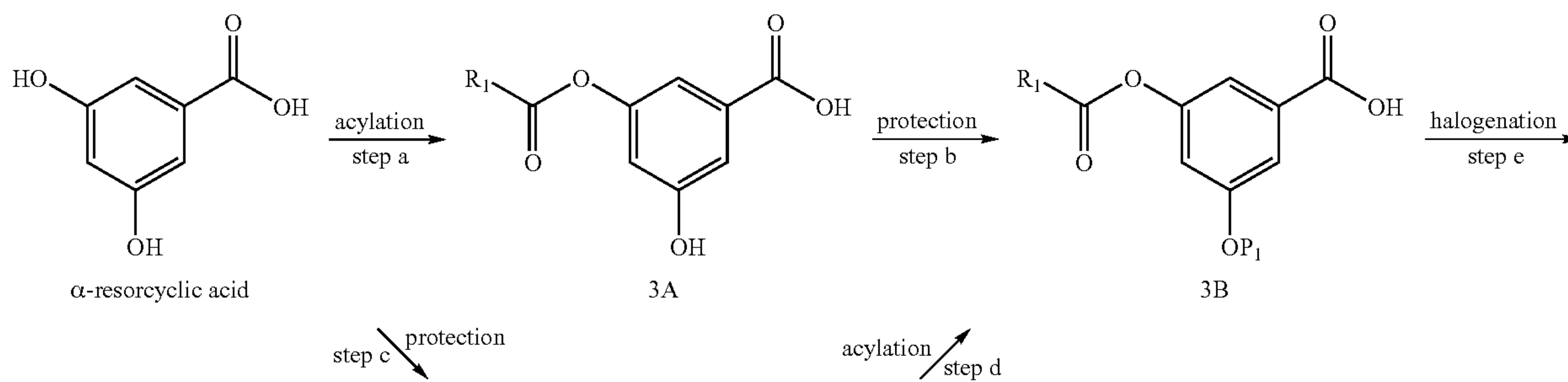
Scheme 4.
