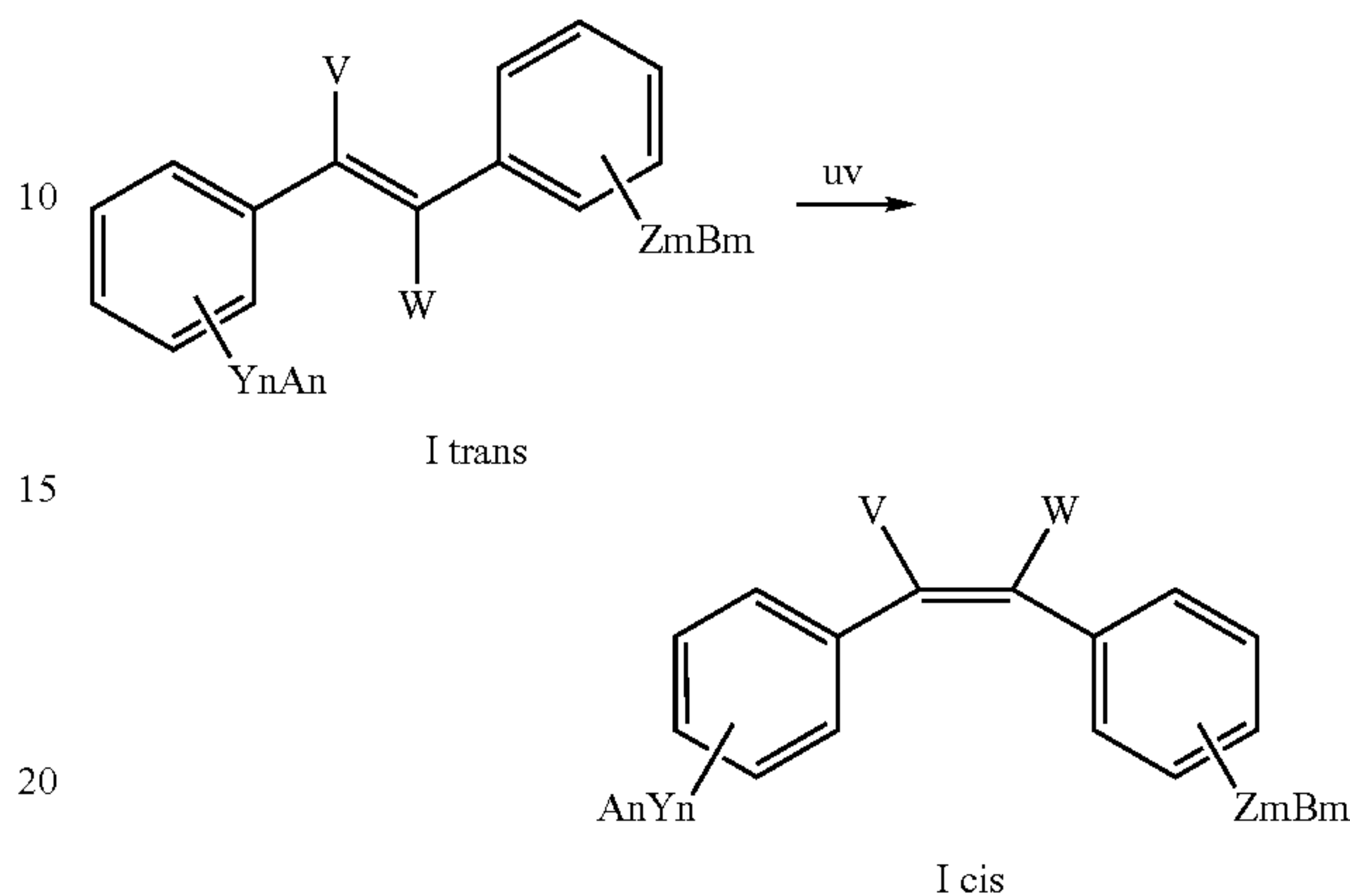
Scheme 10.
