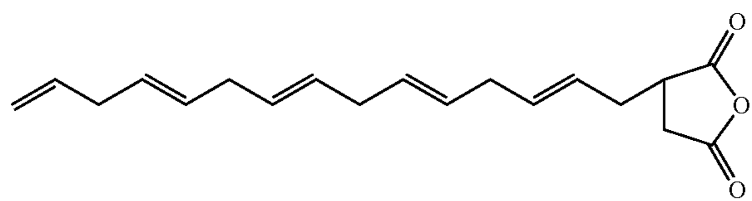
Pentapropenyl succinic anhydride
