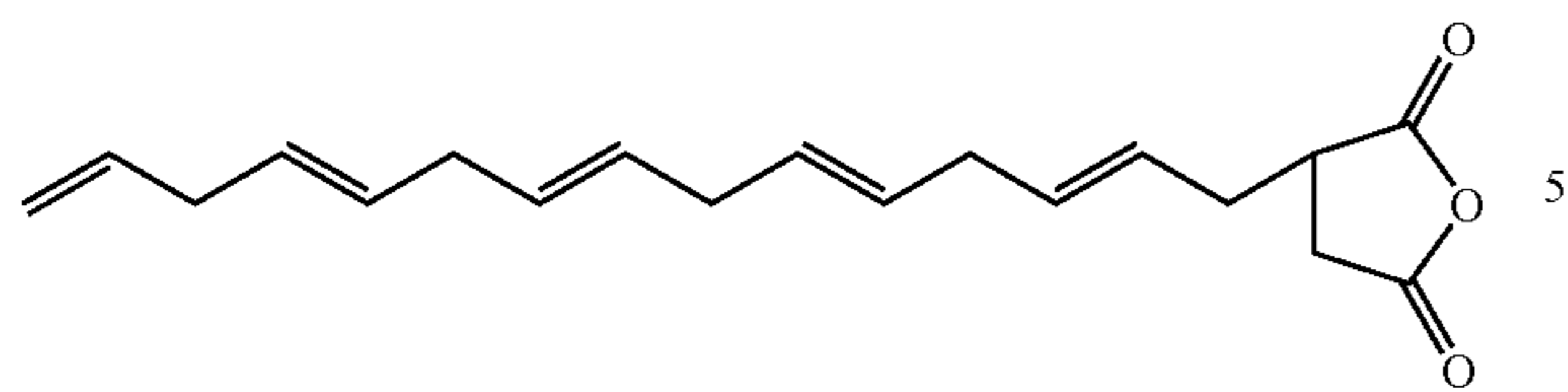
Pentapropenyl succinic anhydride
