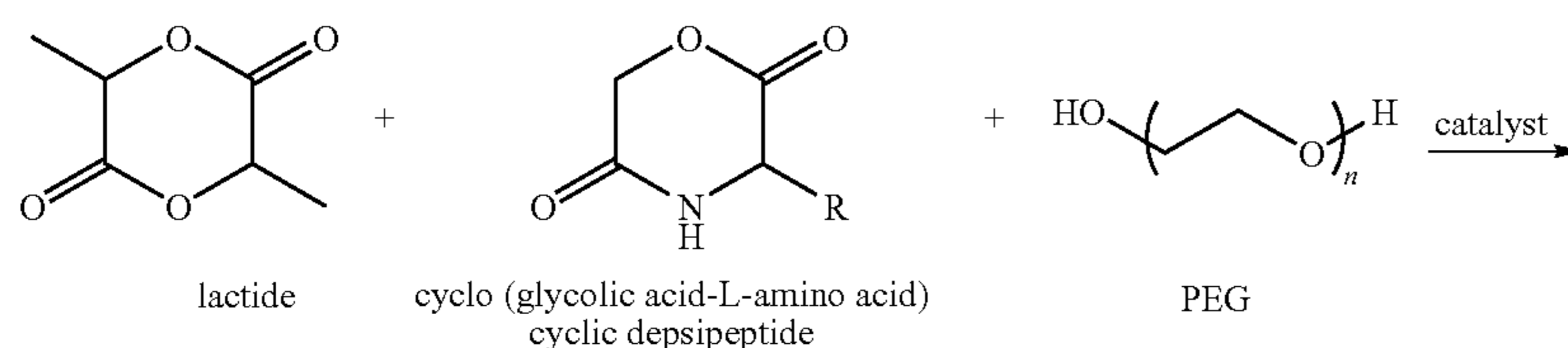
Formula (2): Synthesis of poly[lactide-r-(glycolic acid-amino acid)]-PEG-poly[lactide-r-(glycolic acid-amino acid)] triblock copolymer
