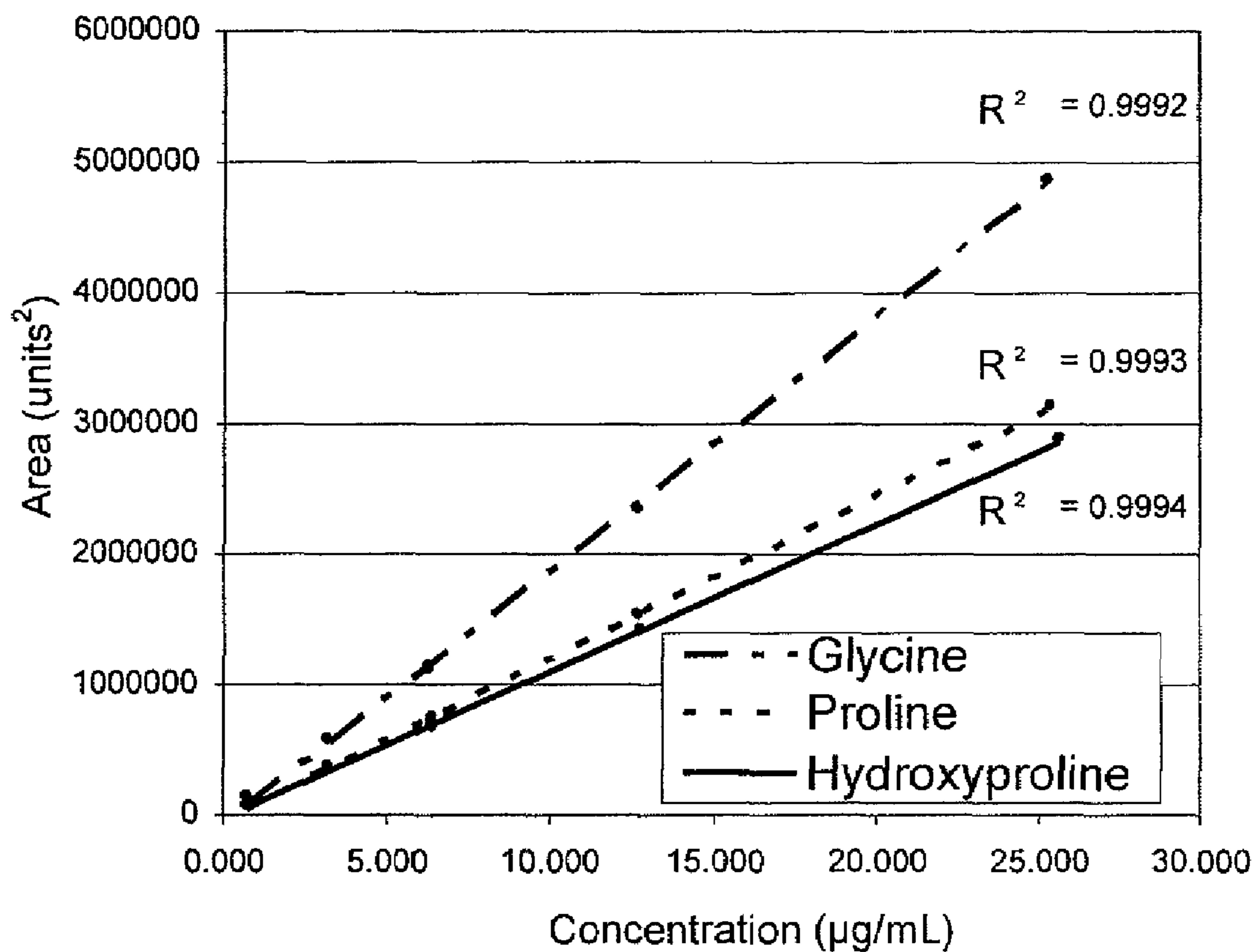
Linearity Plot for Hydroxyproline, Glycine, and Proline
