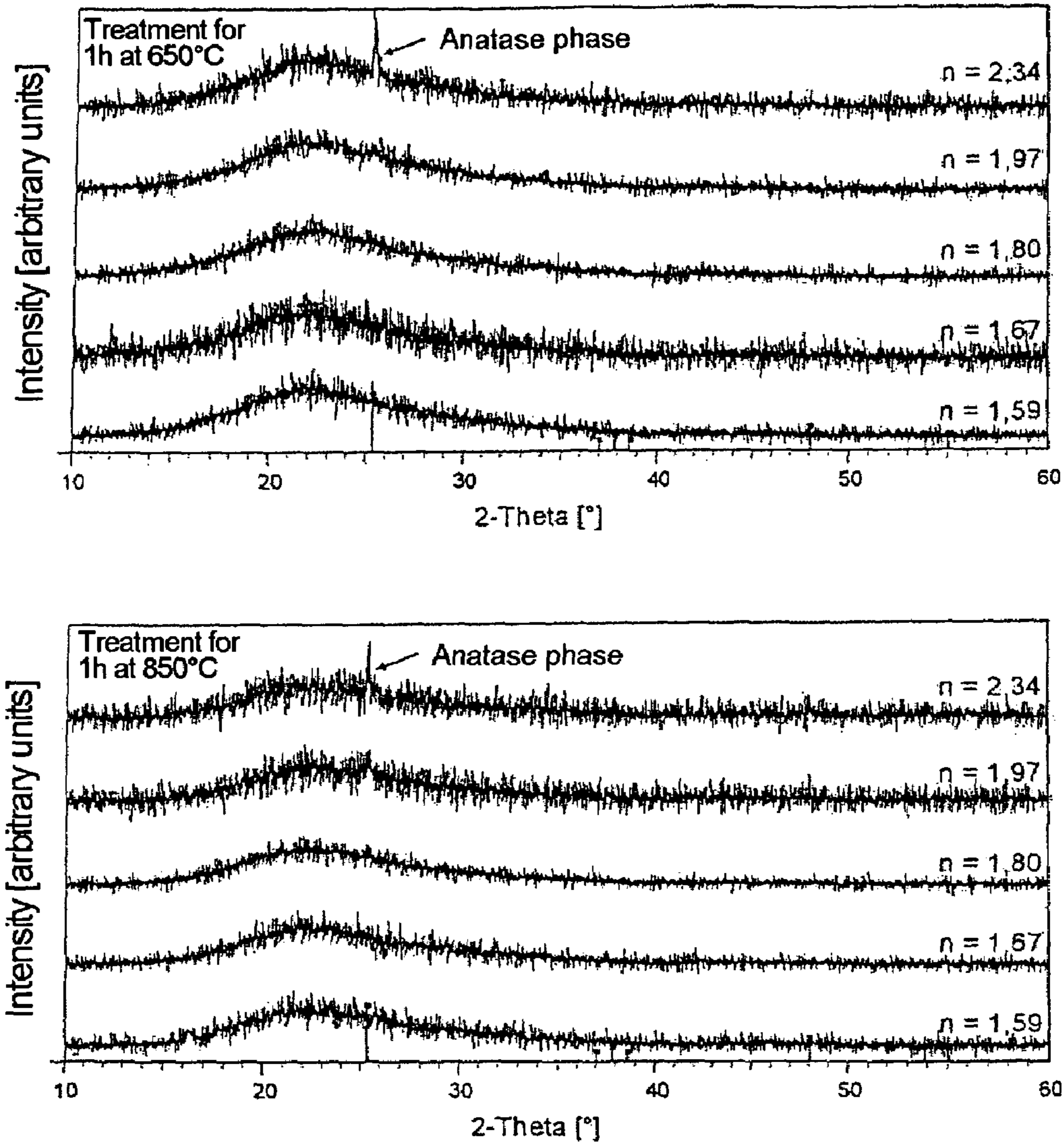
Fig. 3 Diffractograms of titanium aluminum oxide layers
