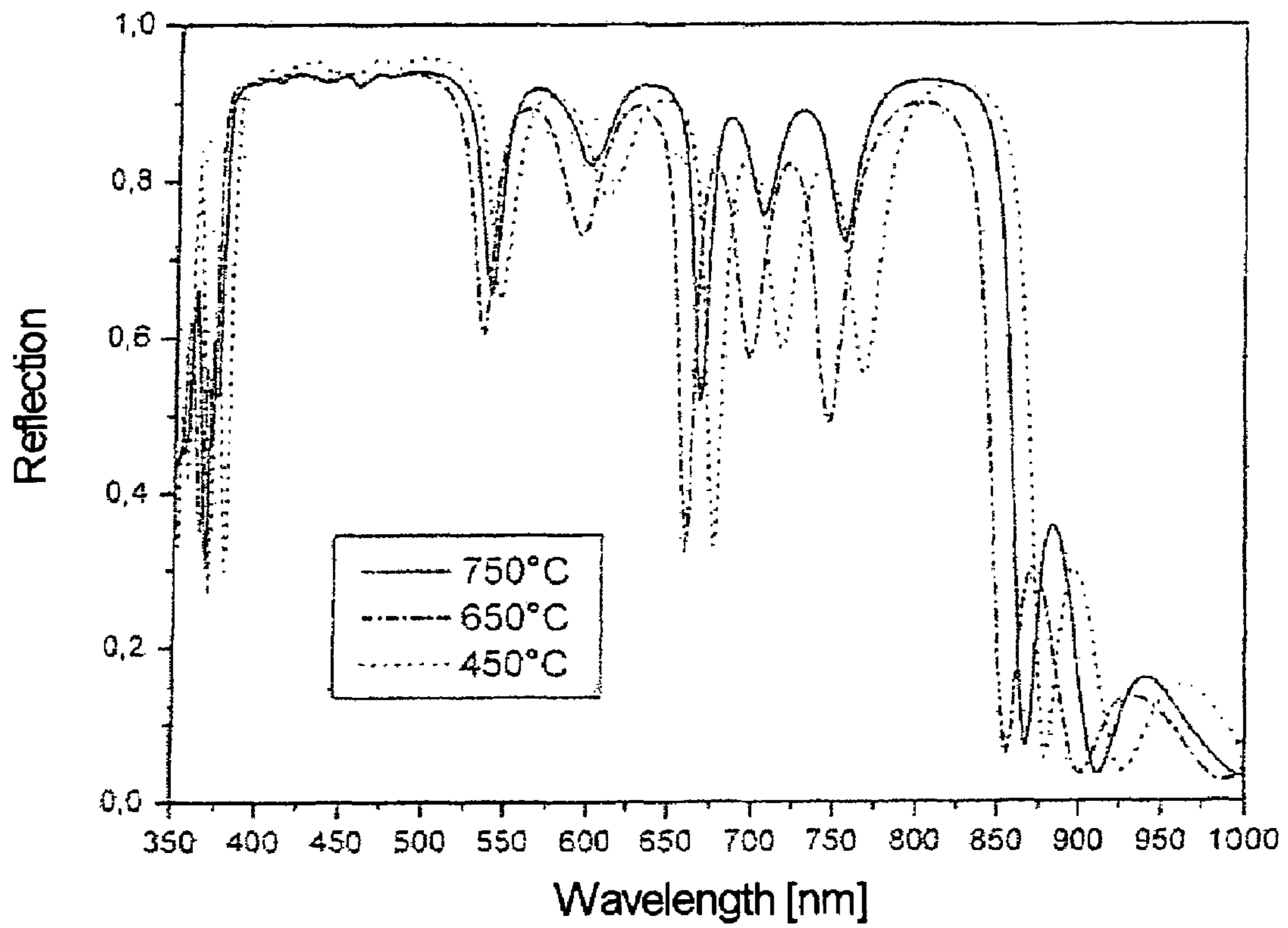
Fig. 2 Reflection properties of the reflector
