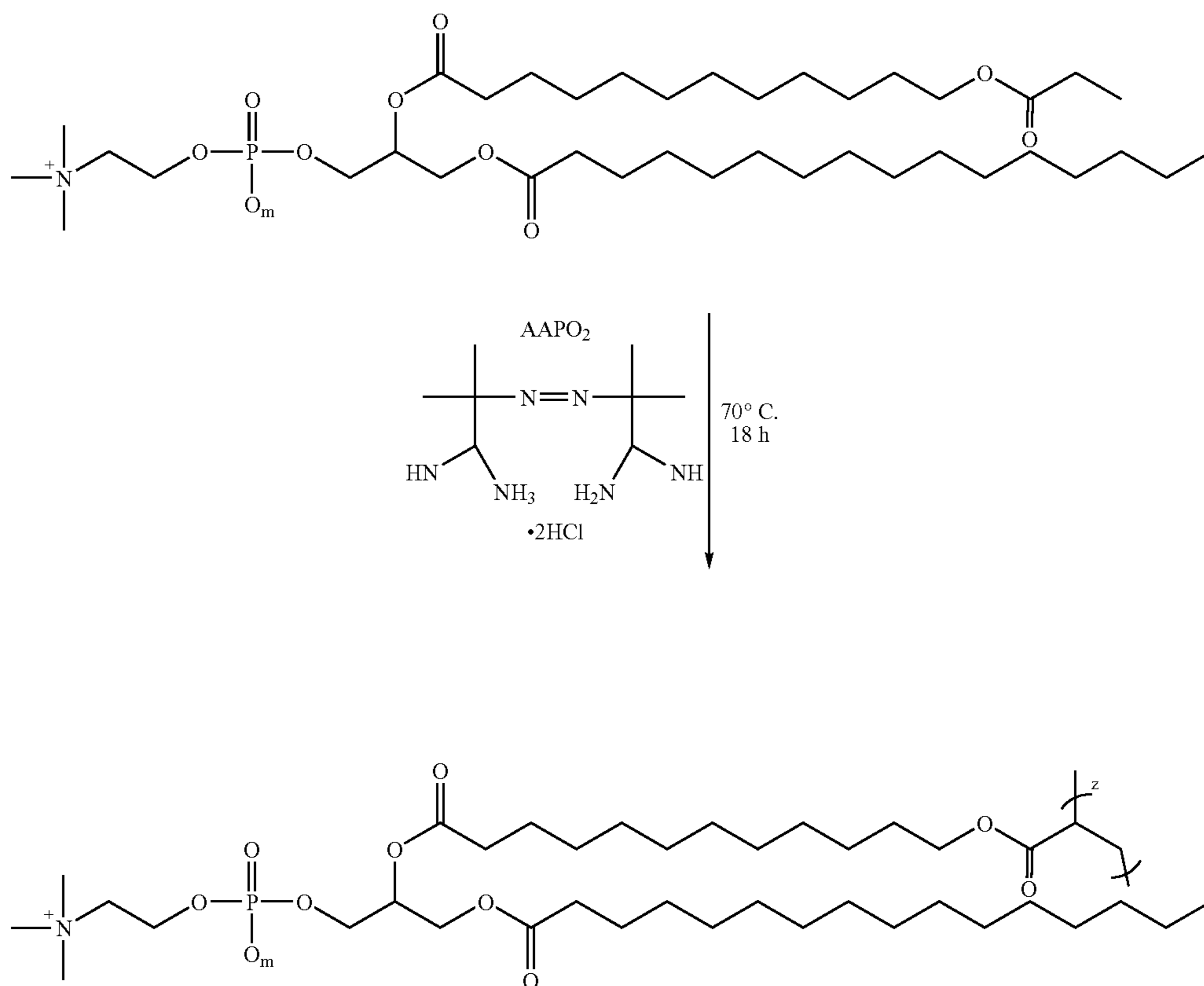
Scheme 2. Polymerization reaction of mono-acryl PC.
