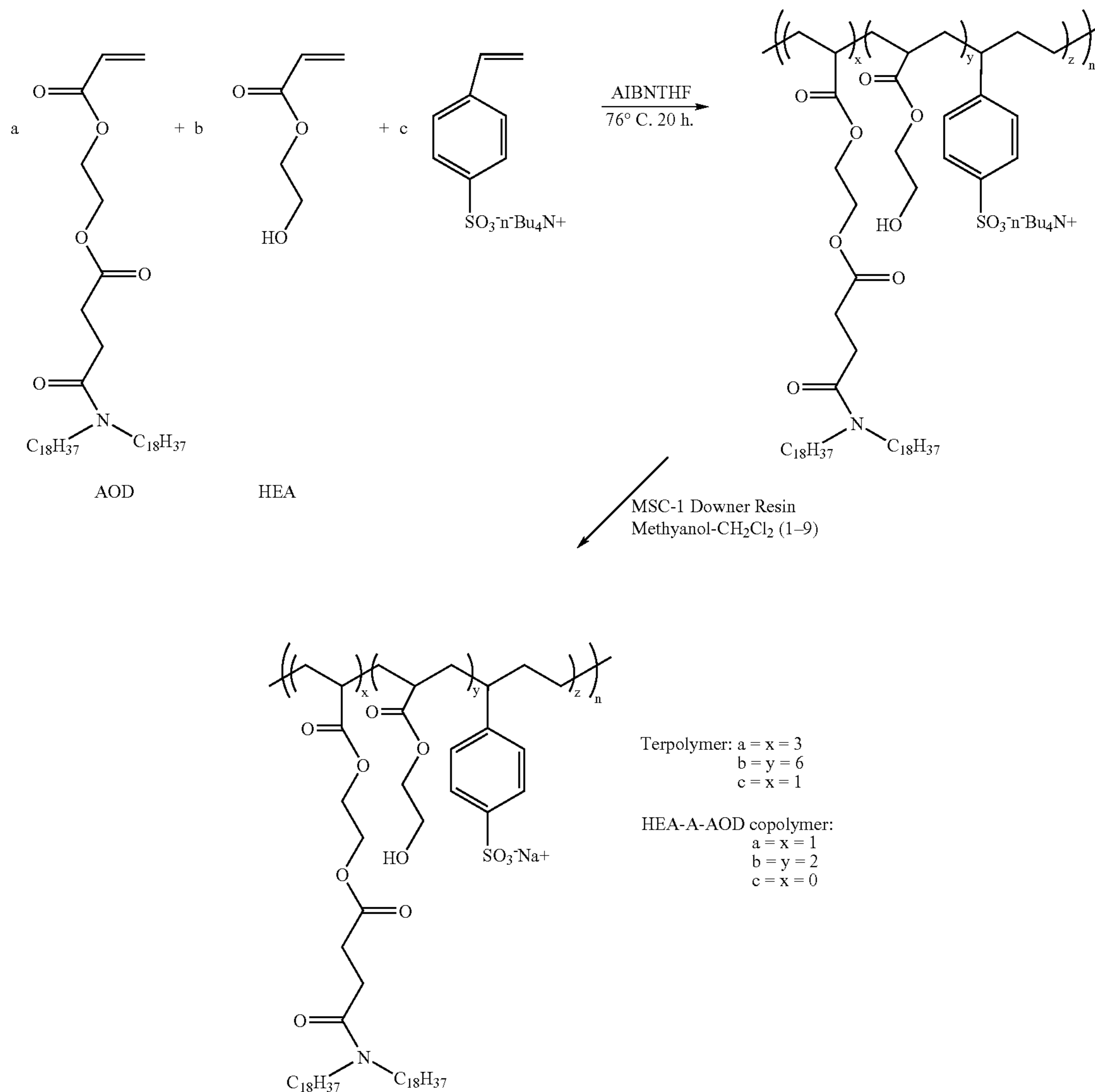
Scheme 3. Synthesis of HEA:AOD (2:1) and HEA:AOD:styrene sulfonate (6:3:1).
