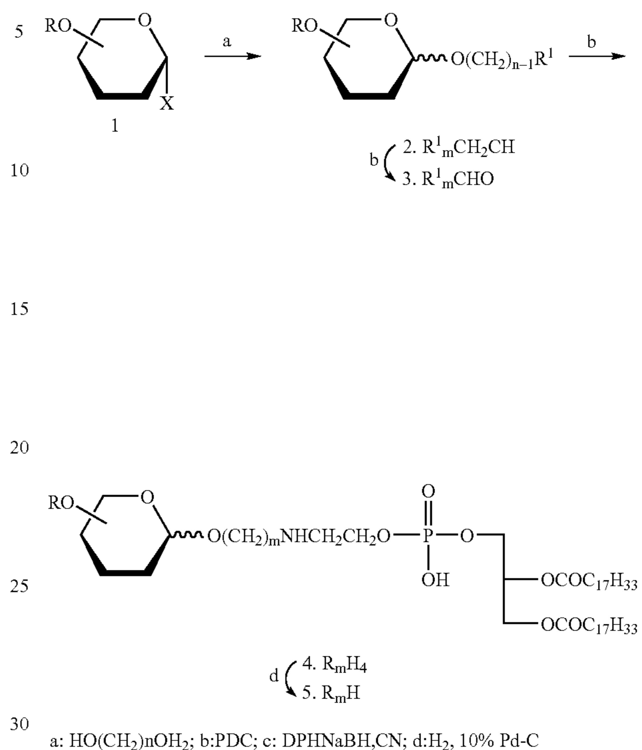
Scheme 1. Synthesis of neoglycophospholipid conjugates
