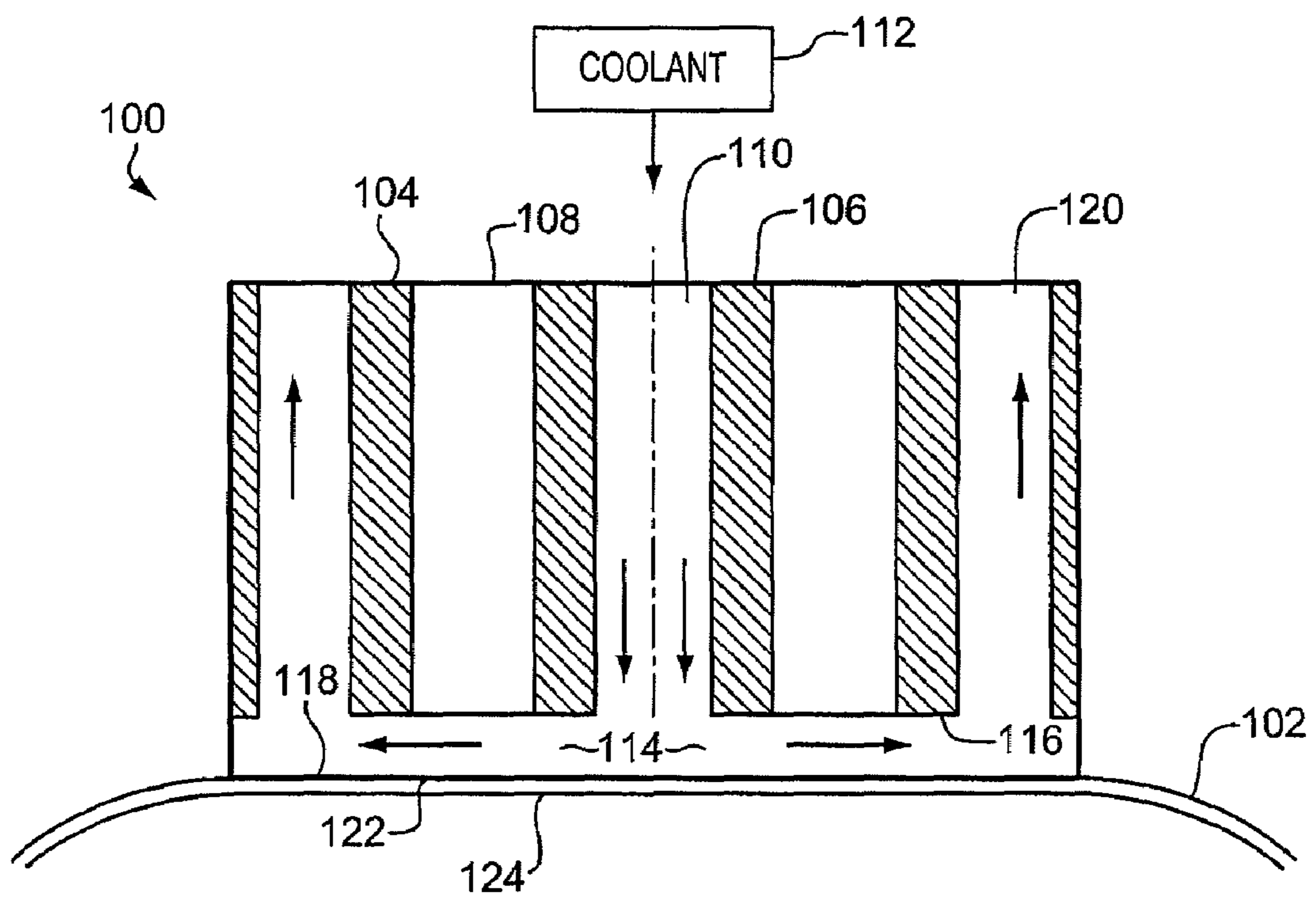
FIG. 1 PRIOR ART
