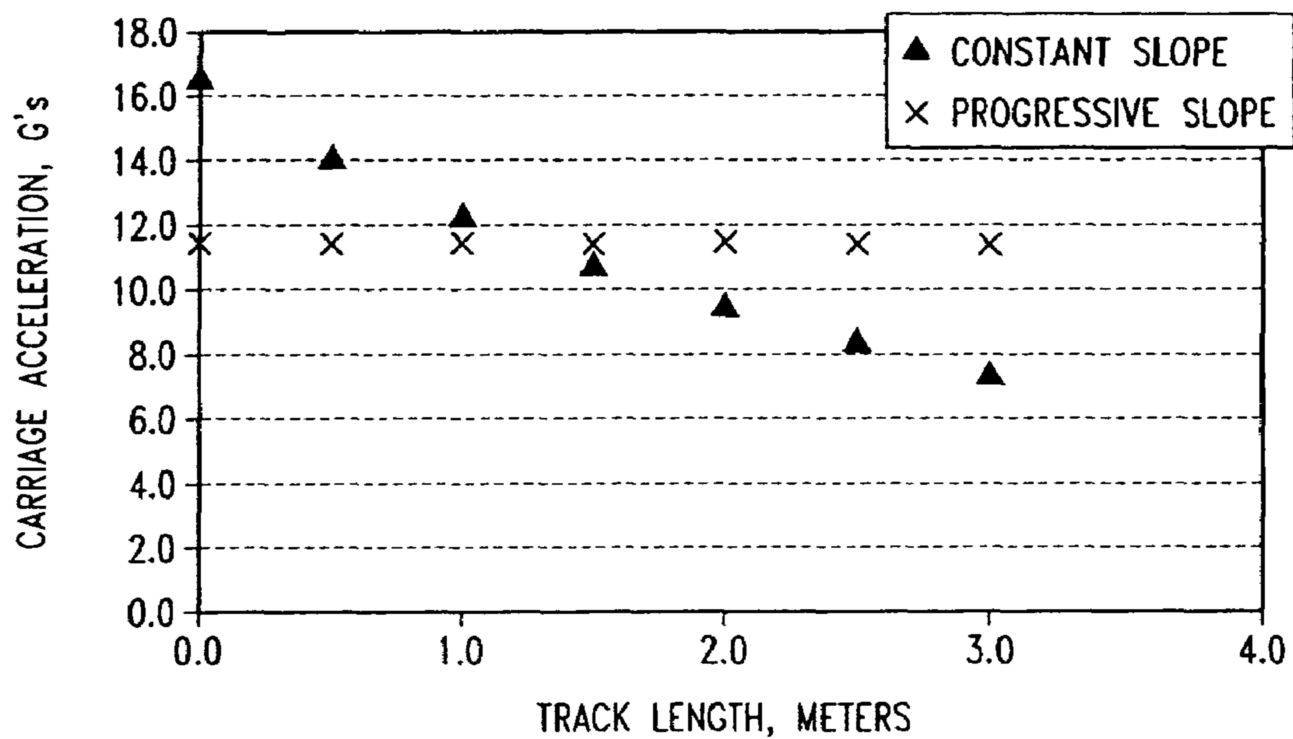
PREDICTED ACCELERATION PROFILES FOR DIFFERENT TRACK SHAPES, SAME ENERGY, SAME END SPEED
