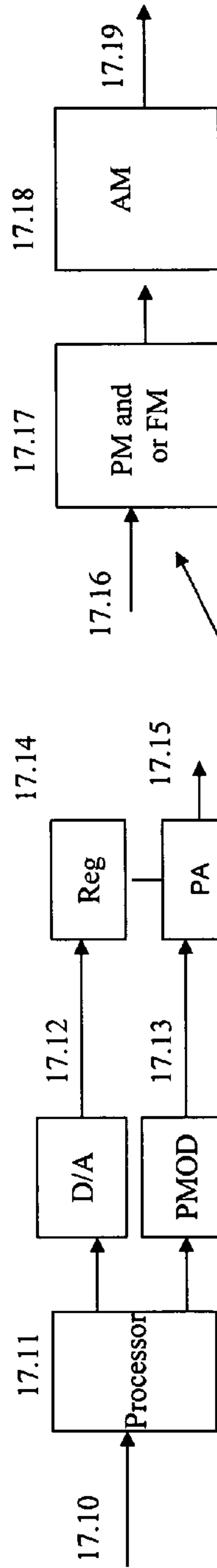
Fig. 17b A prior art Non Quadrature -Polar Modulator
