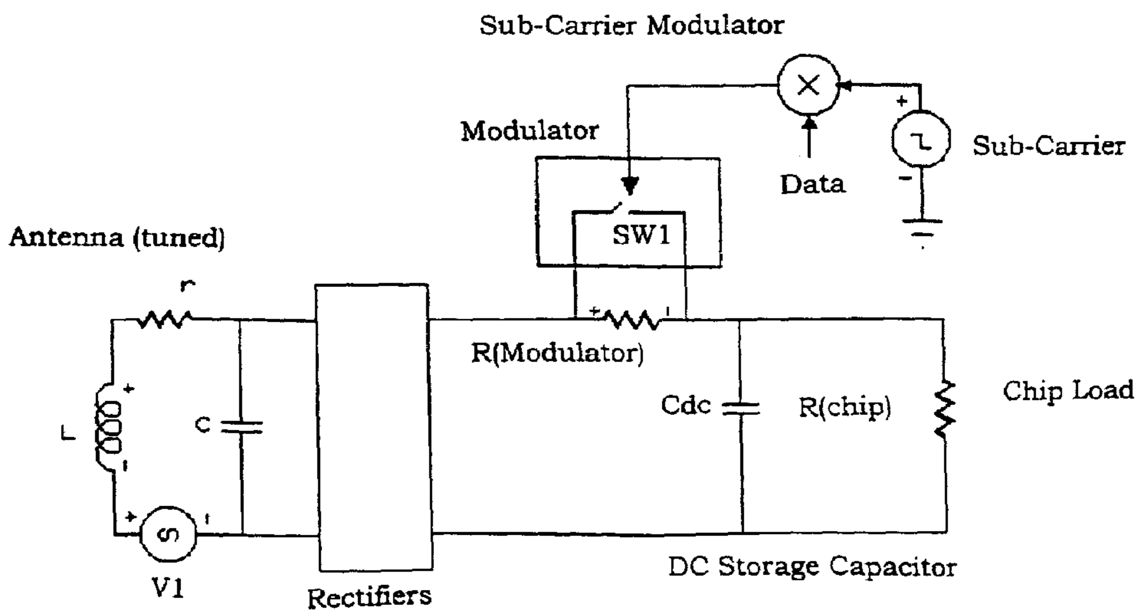
Figure 9(b): Invention with Data Modulated onto Sub-Carrier with Modulator in DC Circuit
