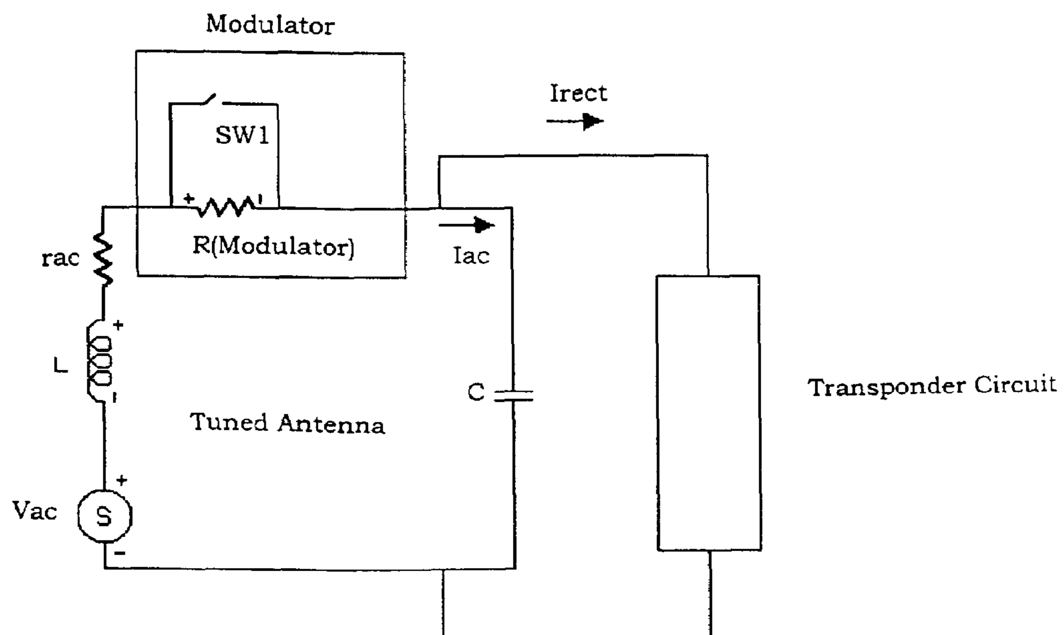
Figure 15(b): Invention with Transponder connected across Tuning Capacitor
