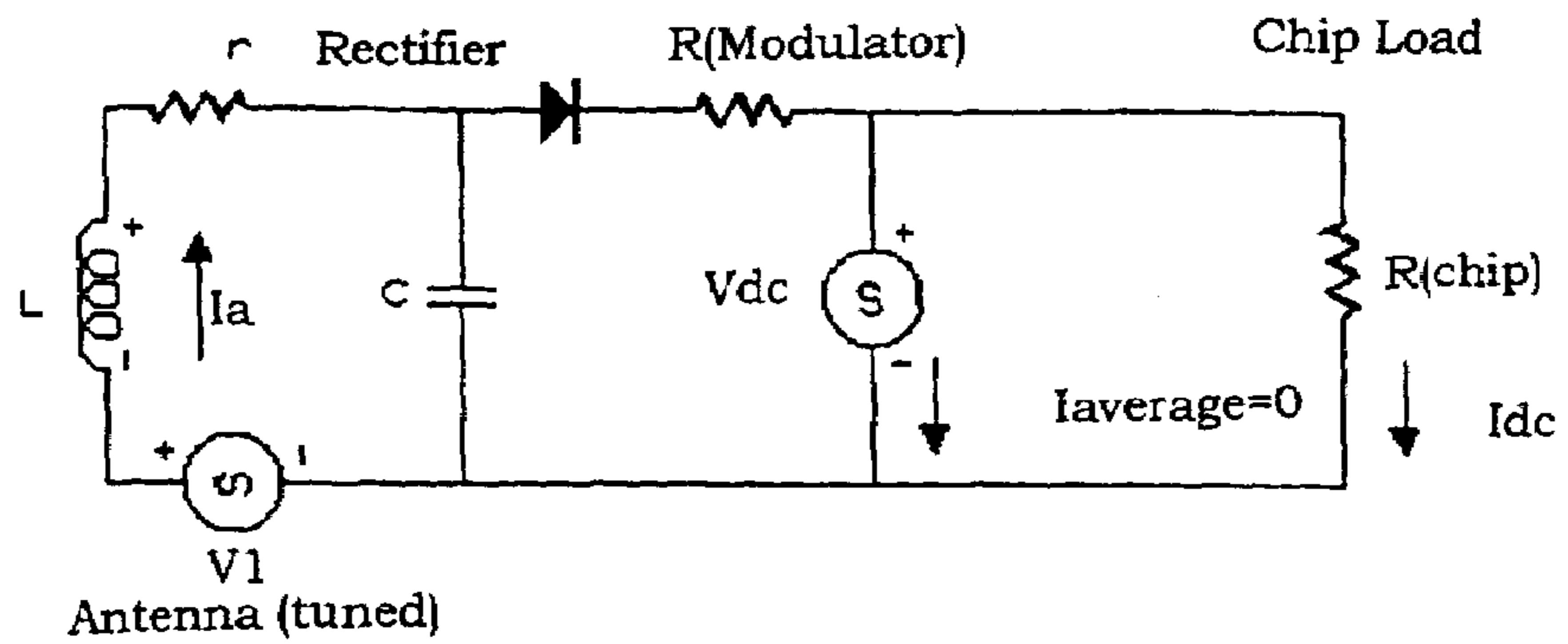
Figure 7(a): Electrical Model for Invention with SW1 Open
