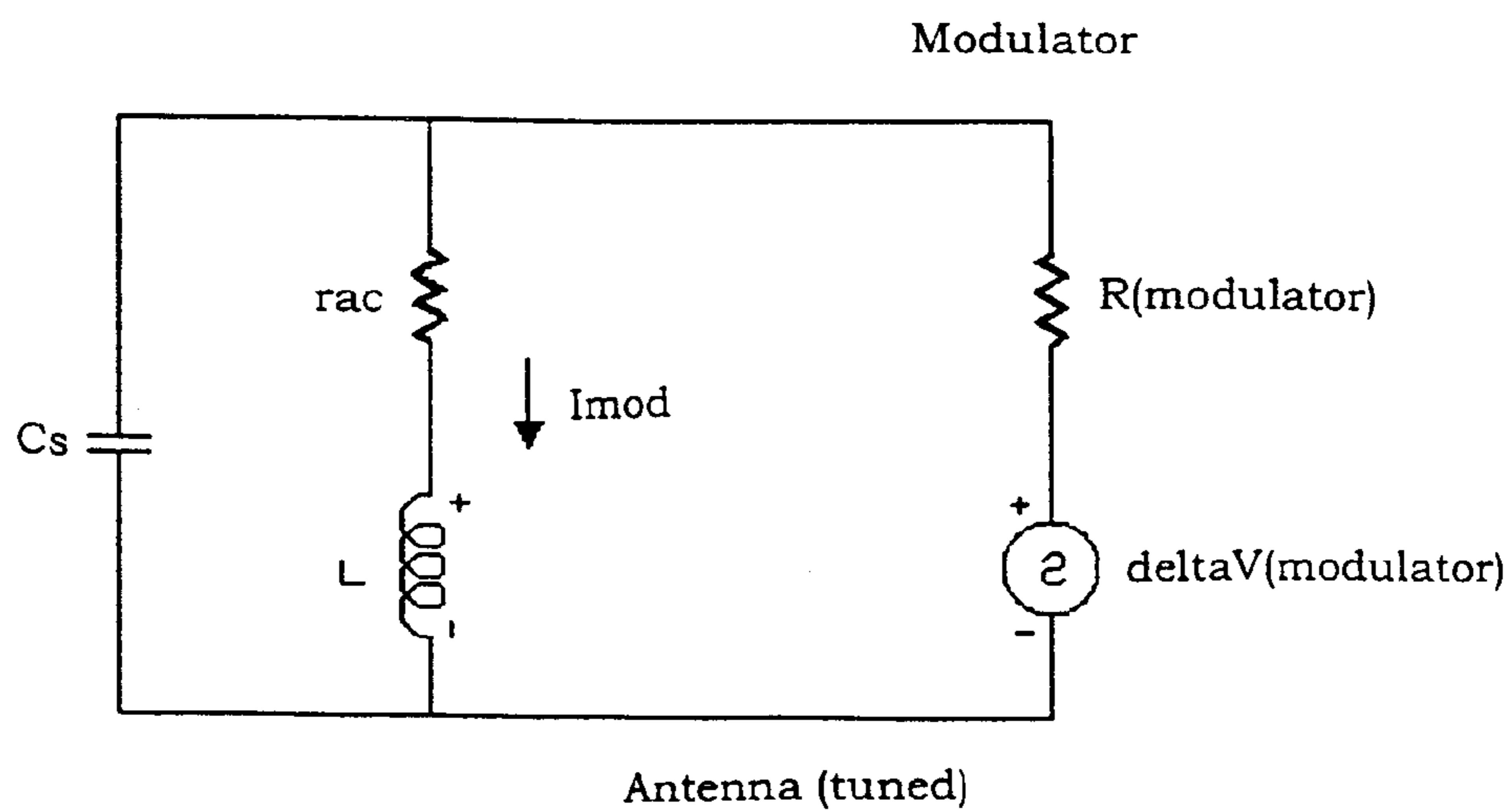
Figure 17(b): Electrical Model of the Invention at Radio Frequency
