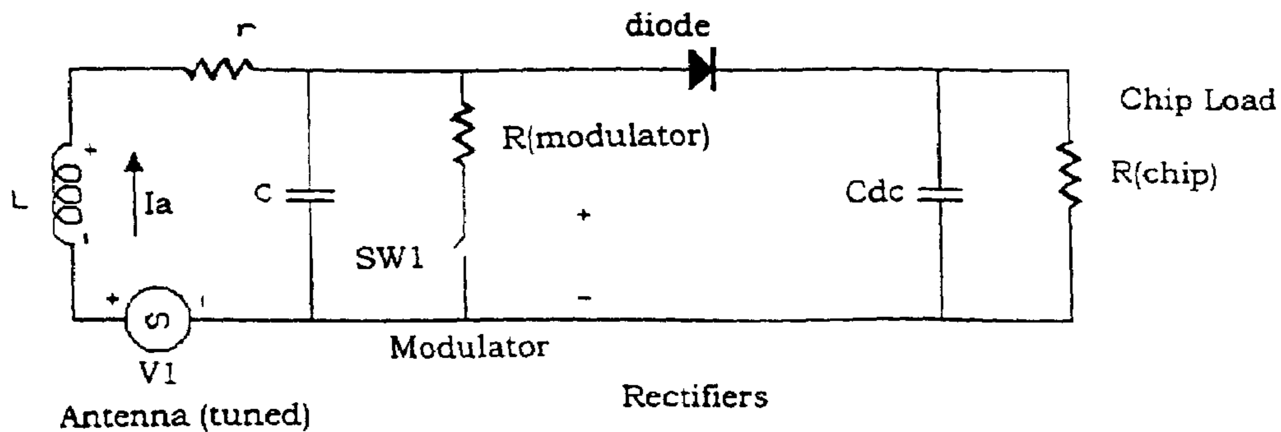
Figure 3: Electrical Model for Prior Art Circuit
