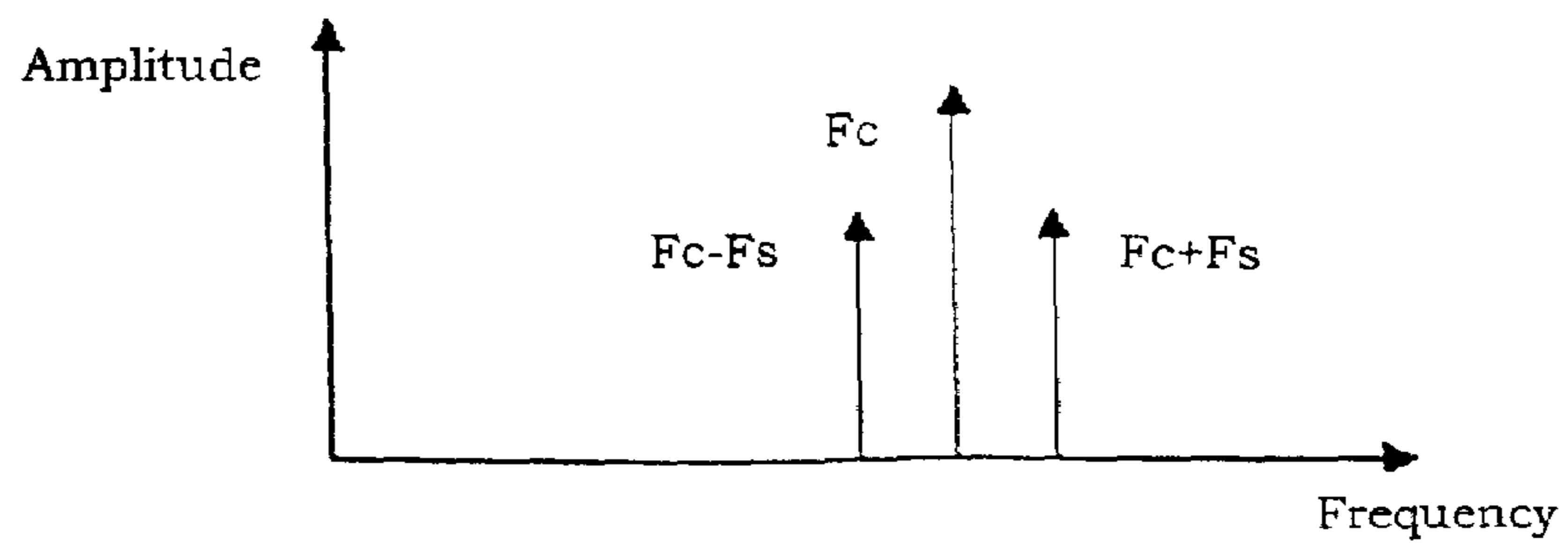
Figure 10(d): Sub-Carrier Amplitude Modulation Sidebands
