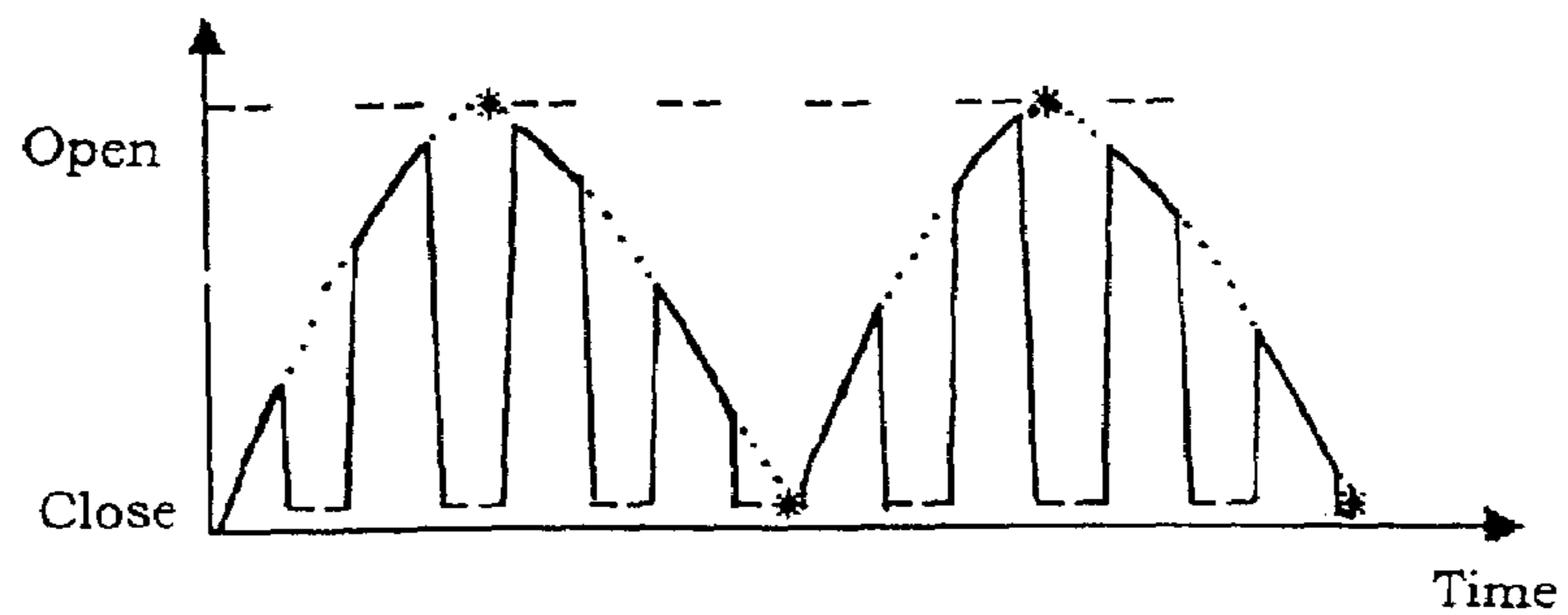
Figure 18(c): Magnitude of V(\text{modulator})
