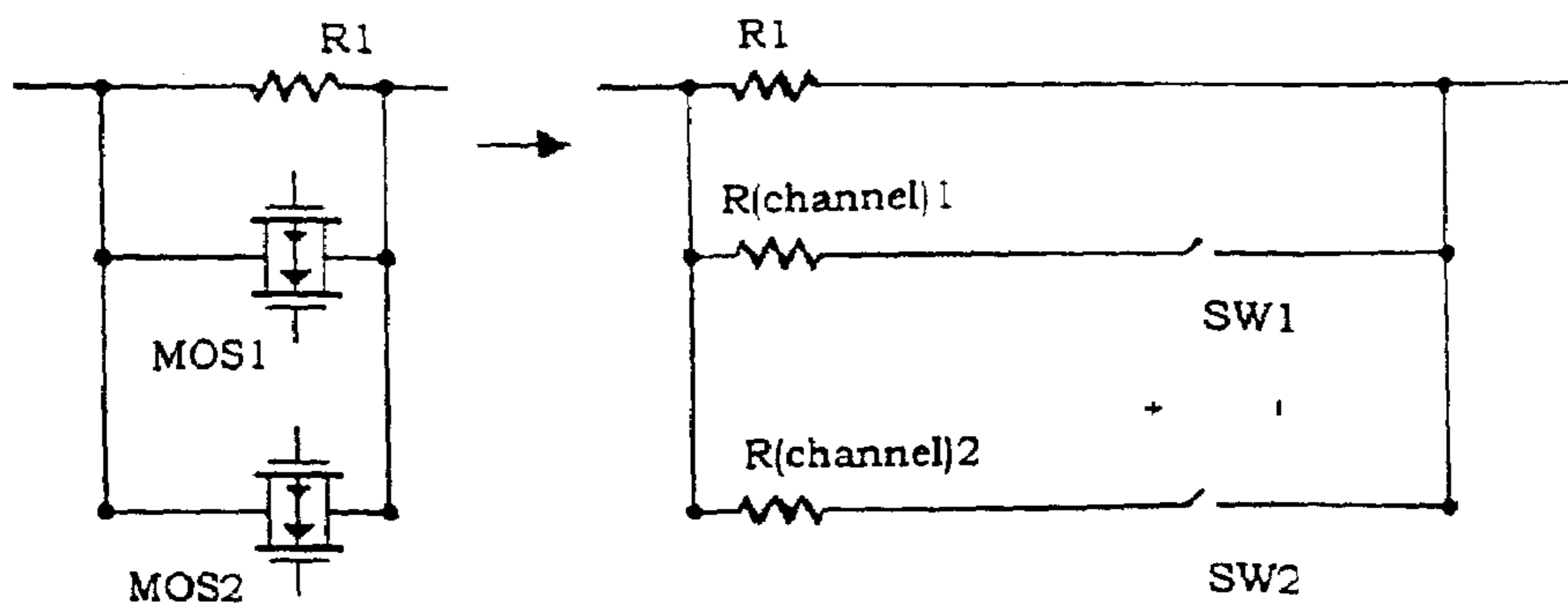
Figure 20(d): Resistance varied between several values
