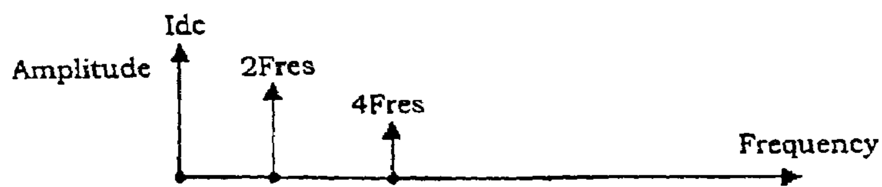
Figure 19(a): Spectrum of I_{ac} Fullwave Rectified
