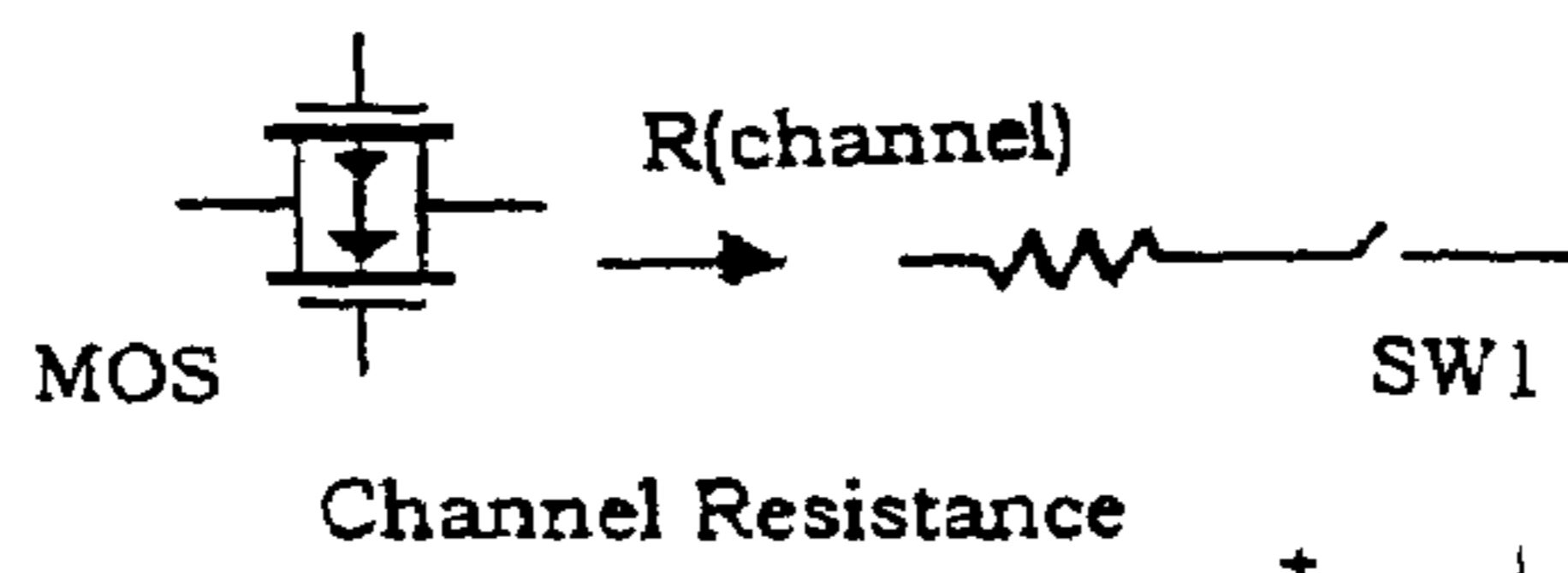
Figure 20(c): Use of Channel Resistance to make Switchable Resistances
