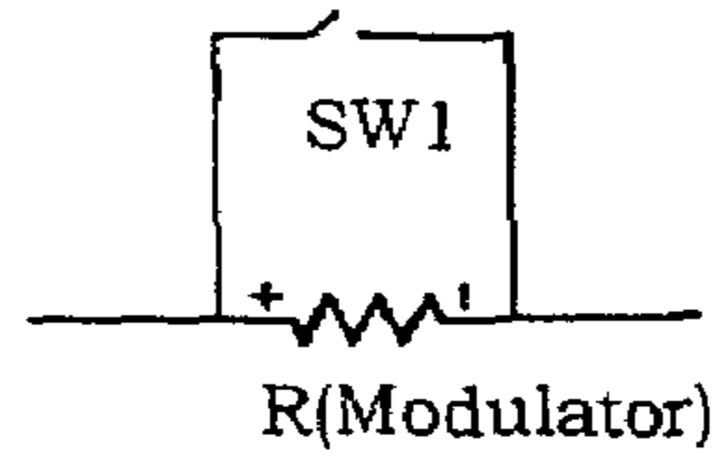
Figure 12(a) Simple Switch Modulator
