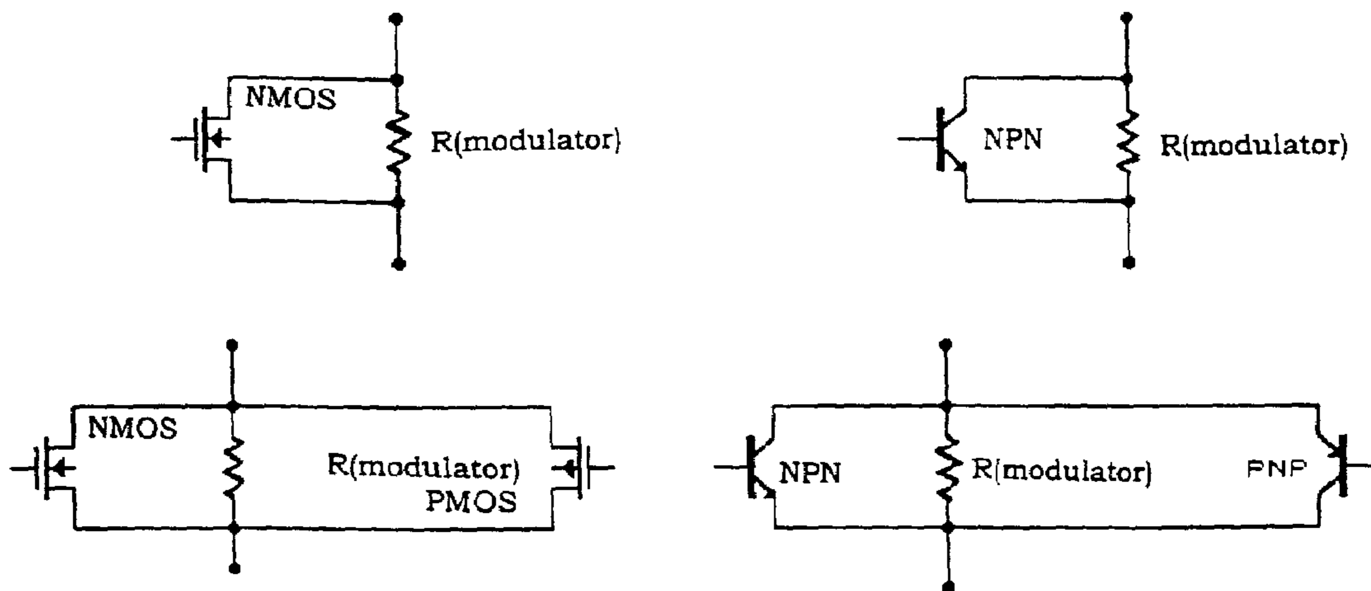
Figure 20(b): Examples of Modulation Switches
