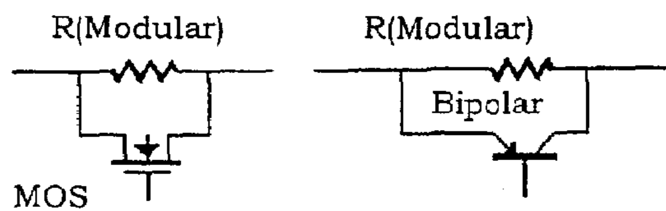
Figure 12(b): Examples of Modulation Switches
