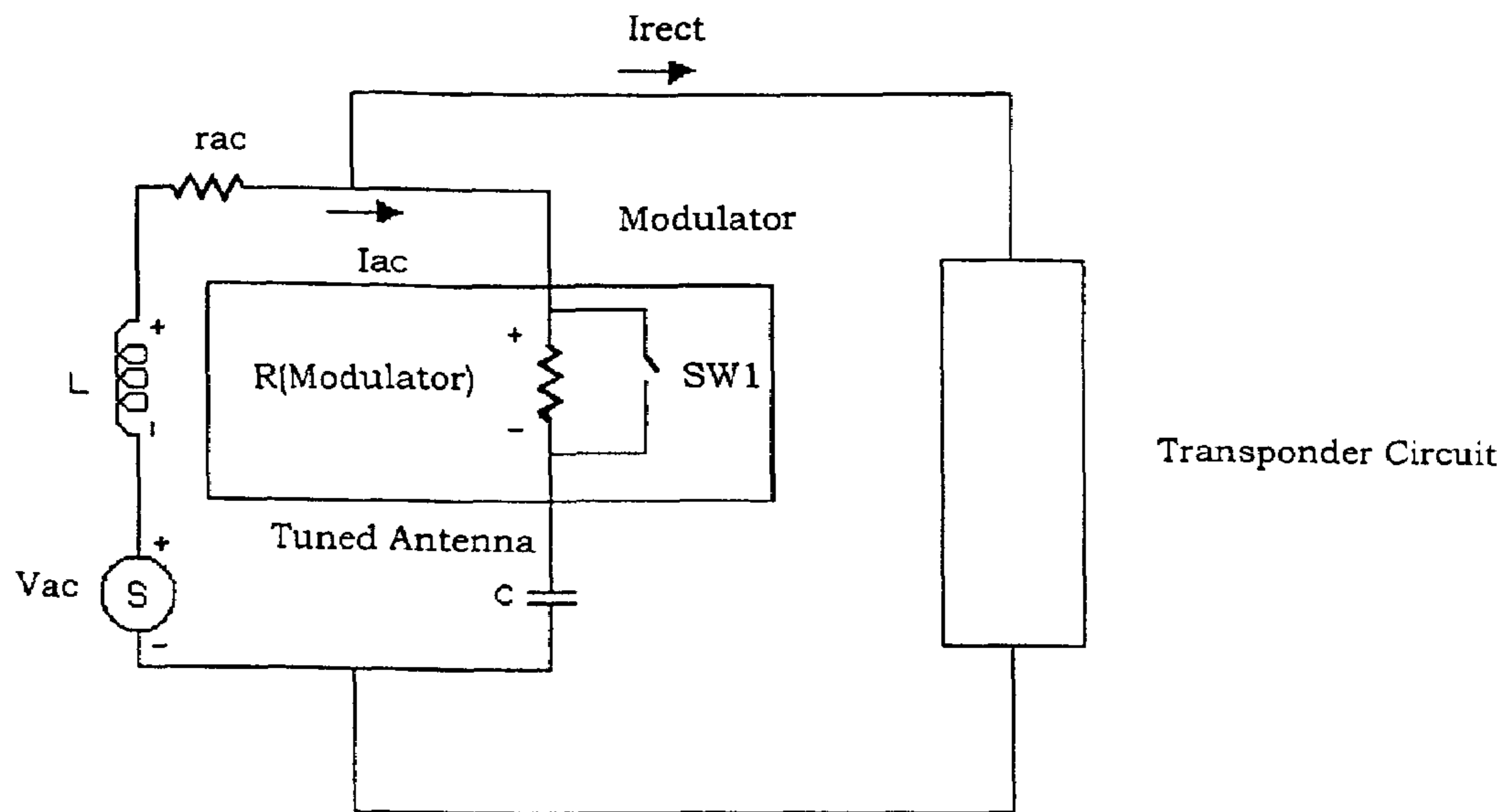
Figure 15(a): Invention with Transponder connected across Coil
