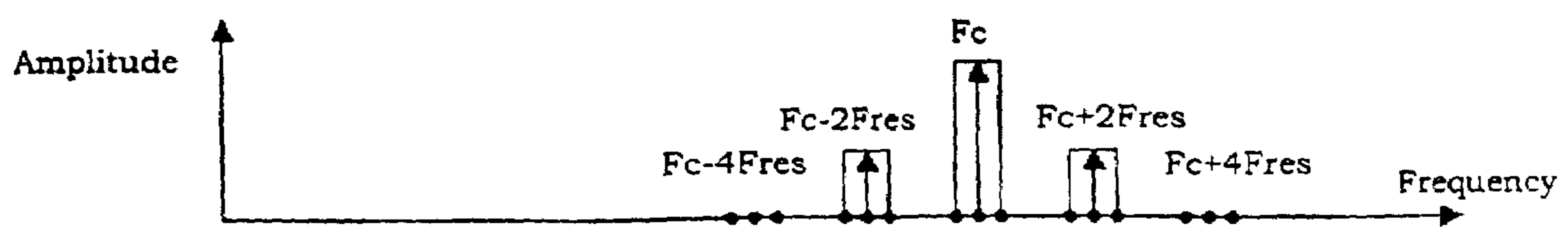
Figure 19(d): Spectrum of V(\text{modulator}) with Waveshaping
