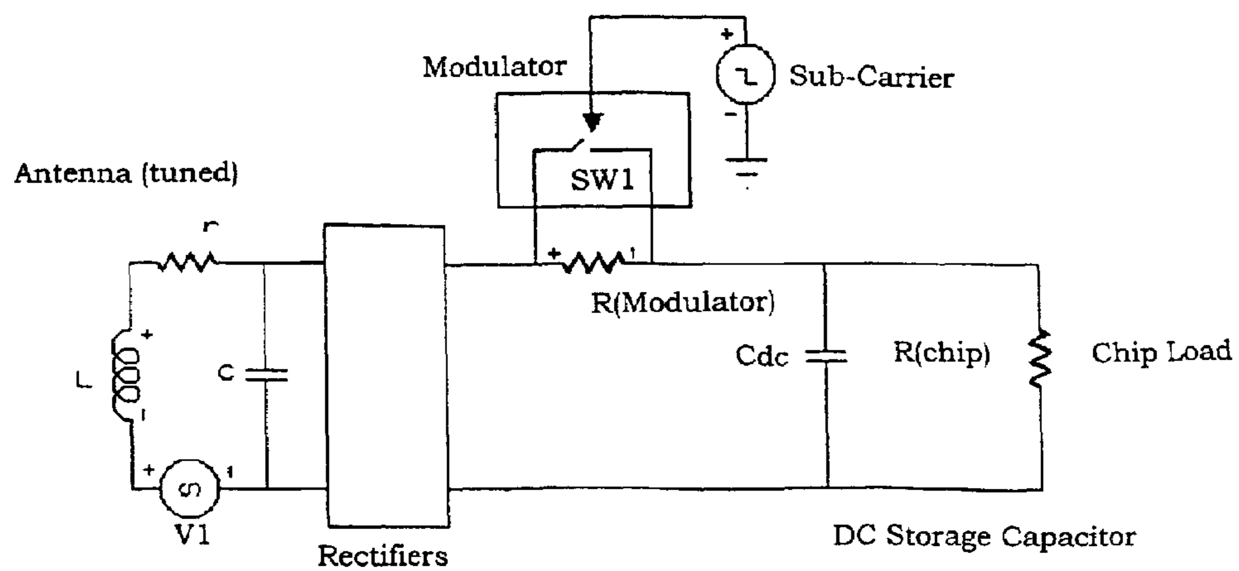
Figure 8(b): Invention with Sub-Carrier Modulation of Modulator in DC Circuit
