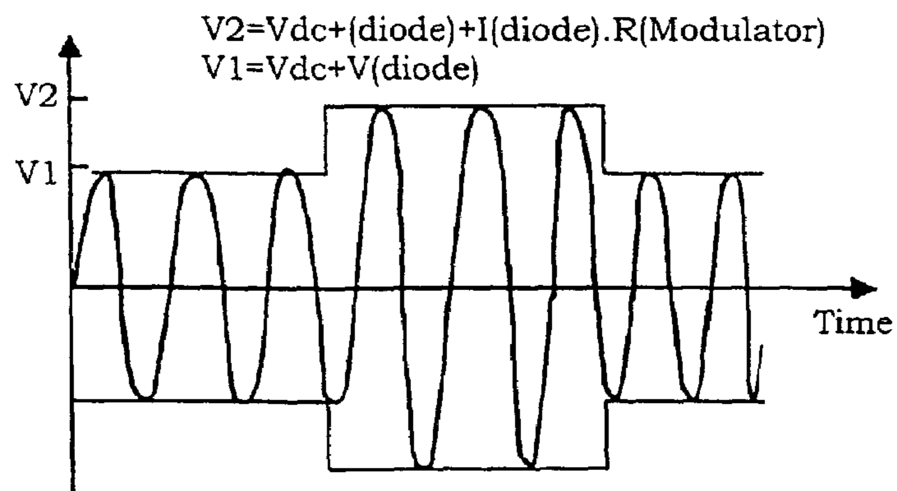
Figure 10(b): Antenna Voltage
