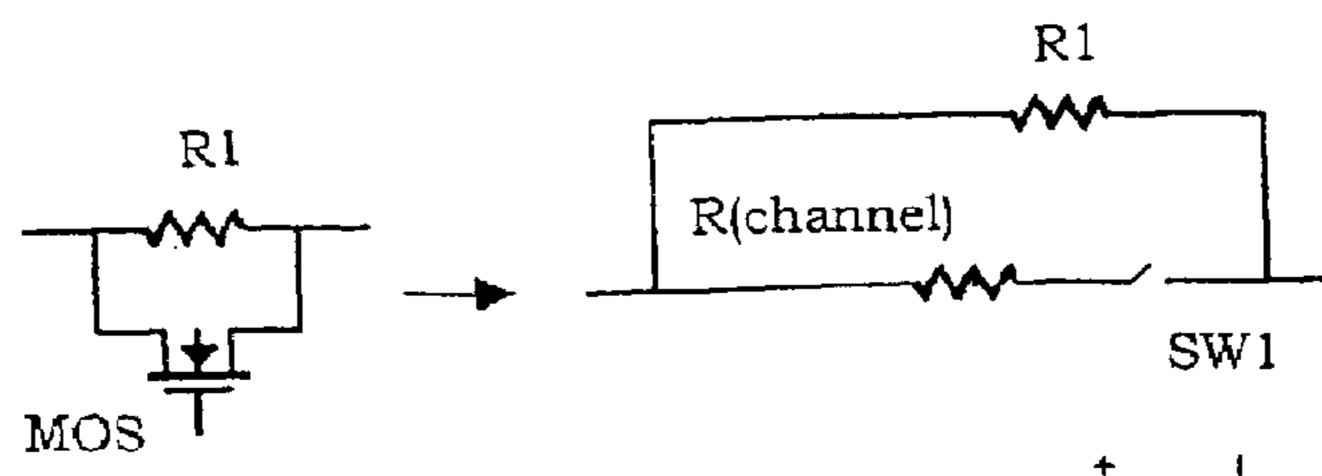
Figure 12(d): Resistance varied between Two Values
