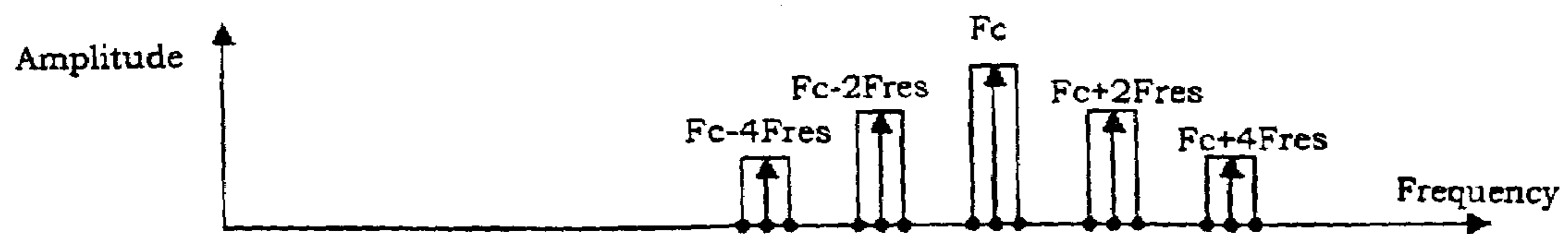
Figure 19(c): Spectrum of V(\text{modulator})
