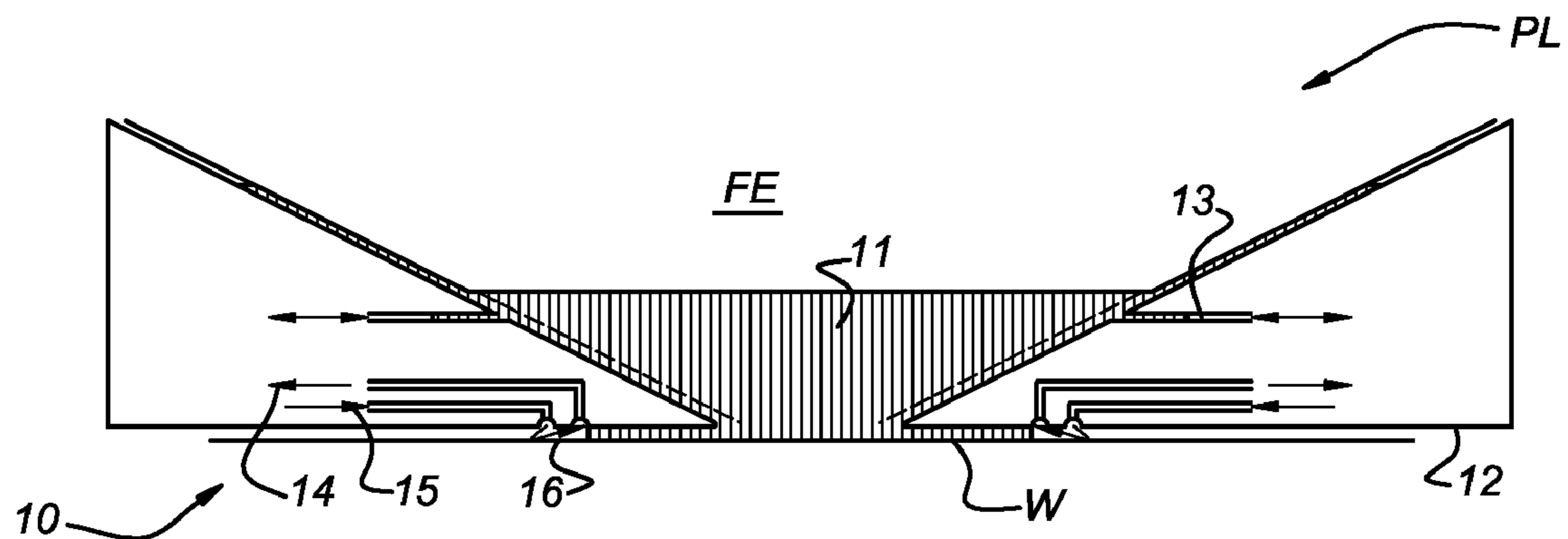
Fig 5 Prior art
