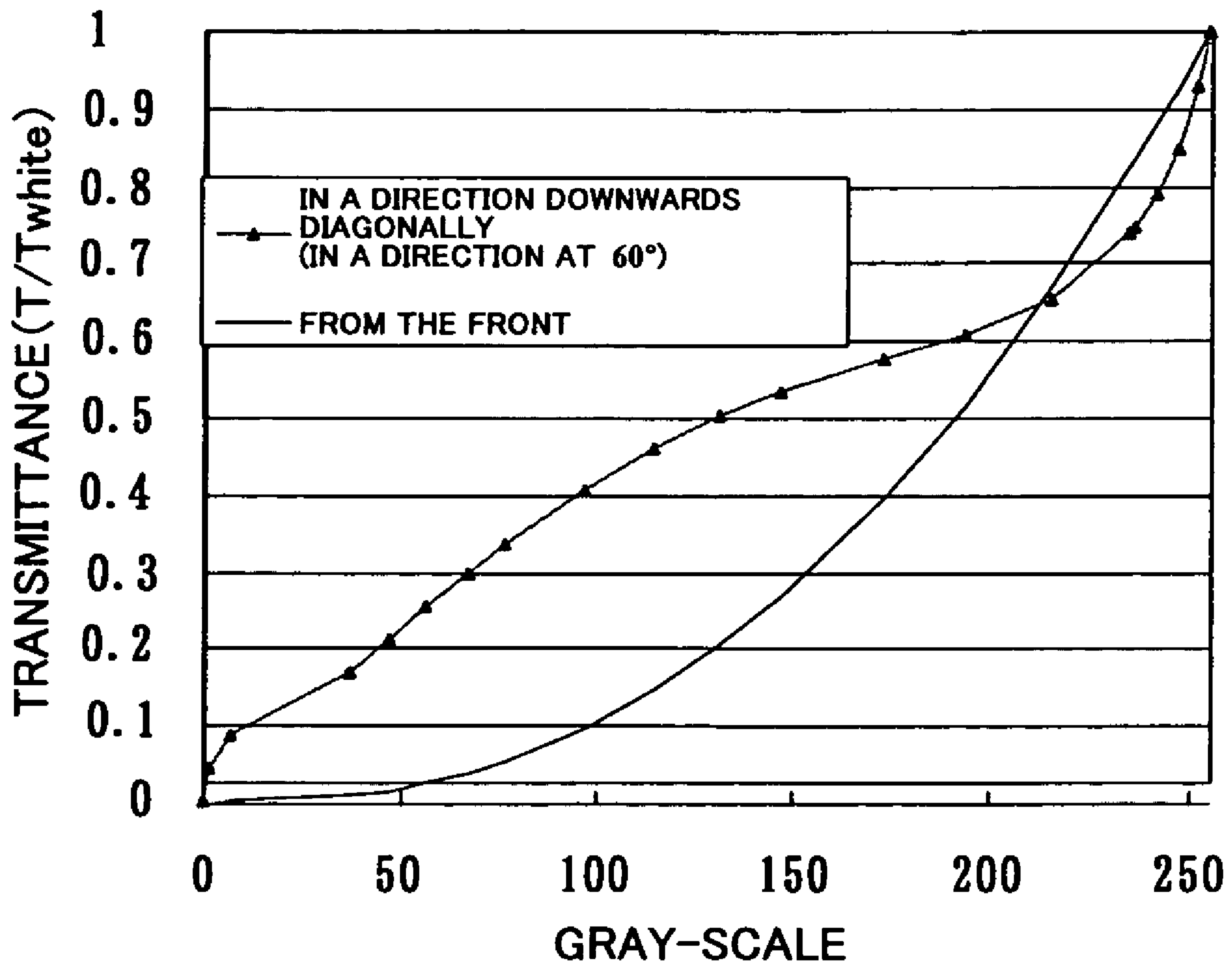
FIG. 2 (PRIOR ART)
