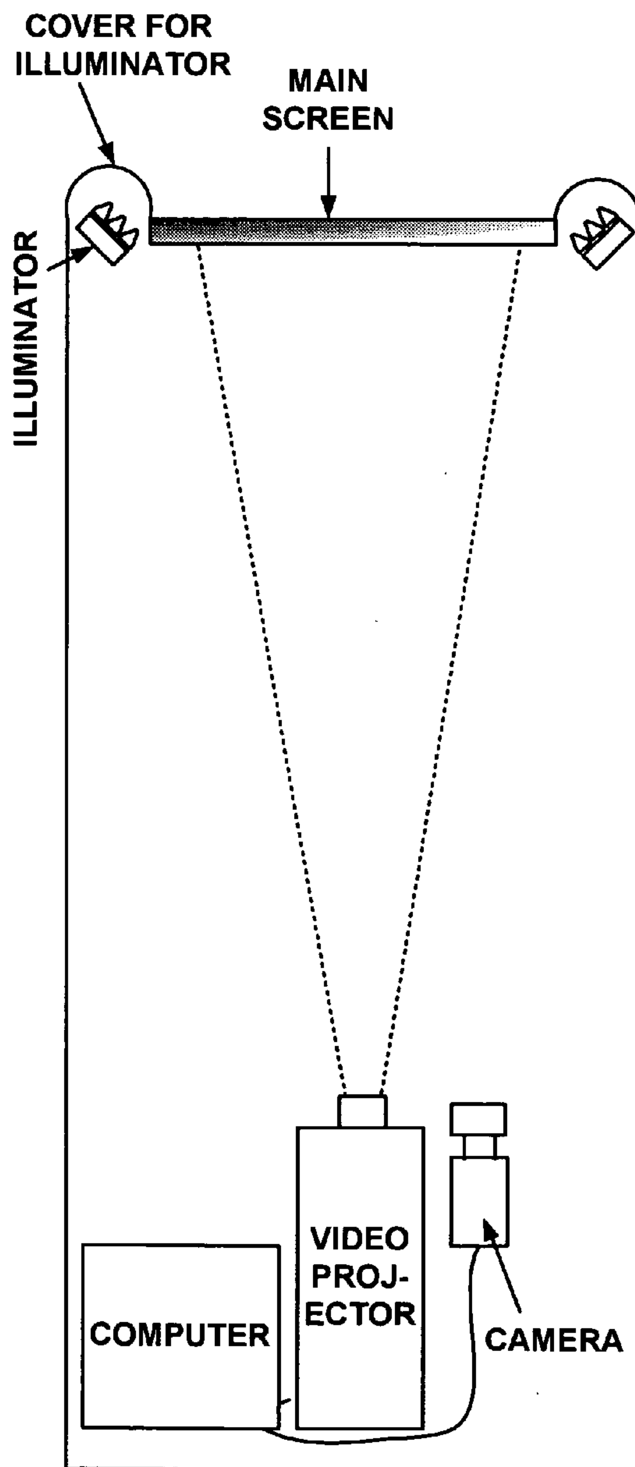
ILLUMINATORS PROTRUDE FROM DISPLAY SURFACE
