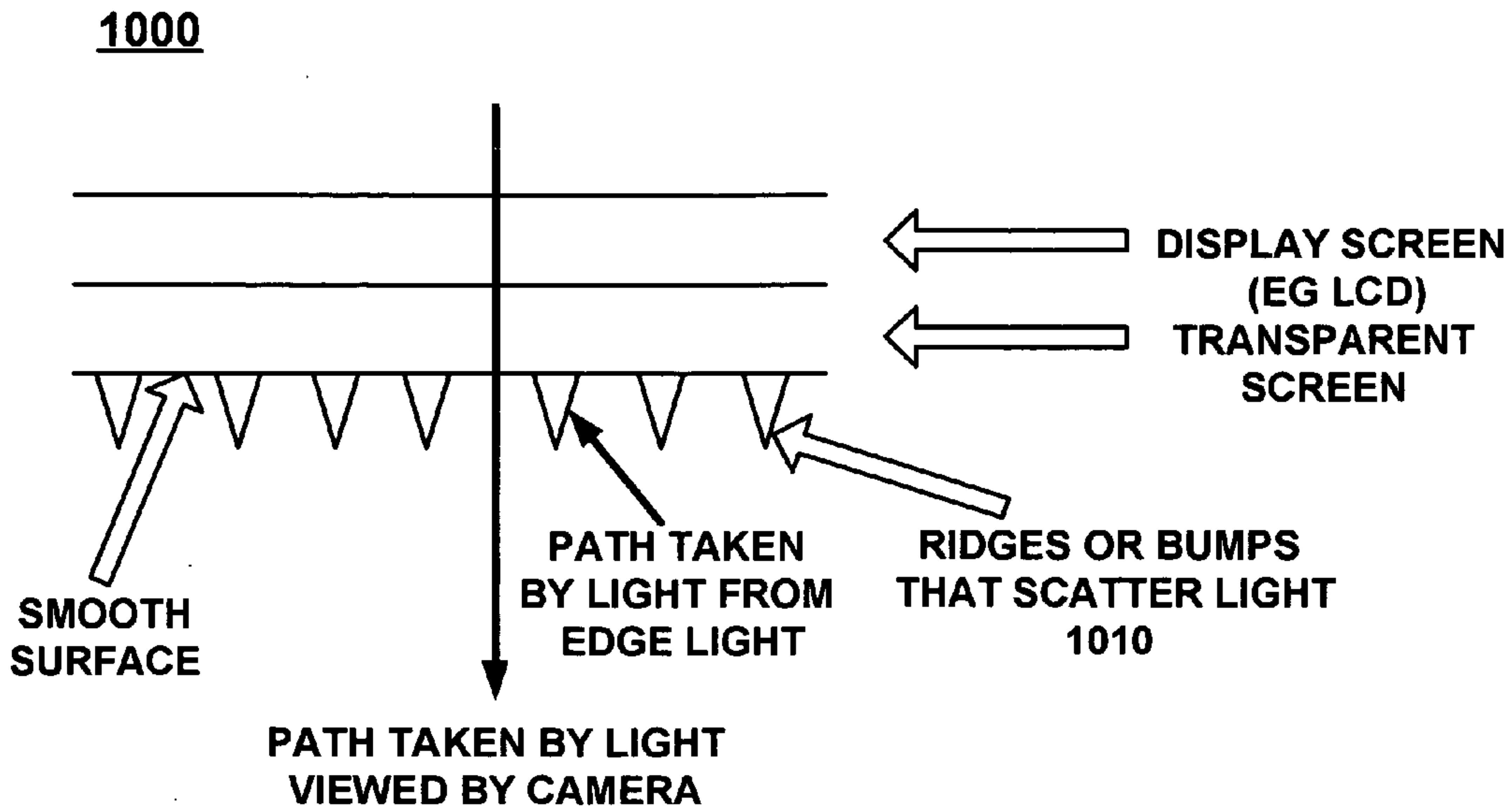
CROSS SECTION OF SCREEN WITH MICROSCOPIC SCATTERING RIDGES OR BUMPS (NOT TO SCALE)
