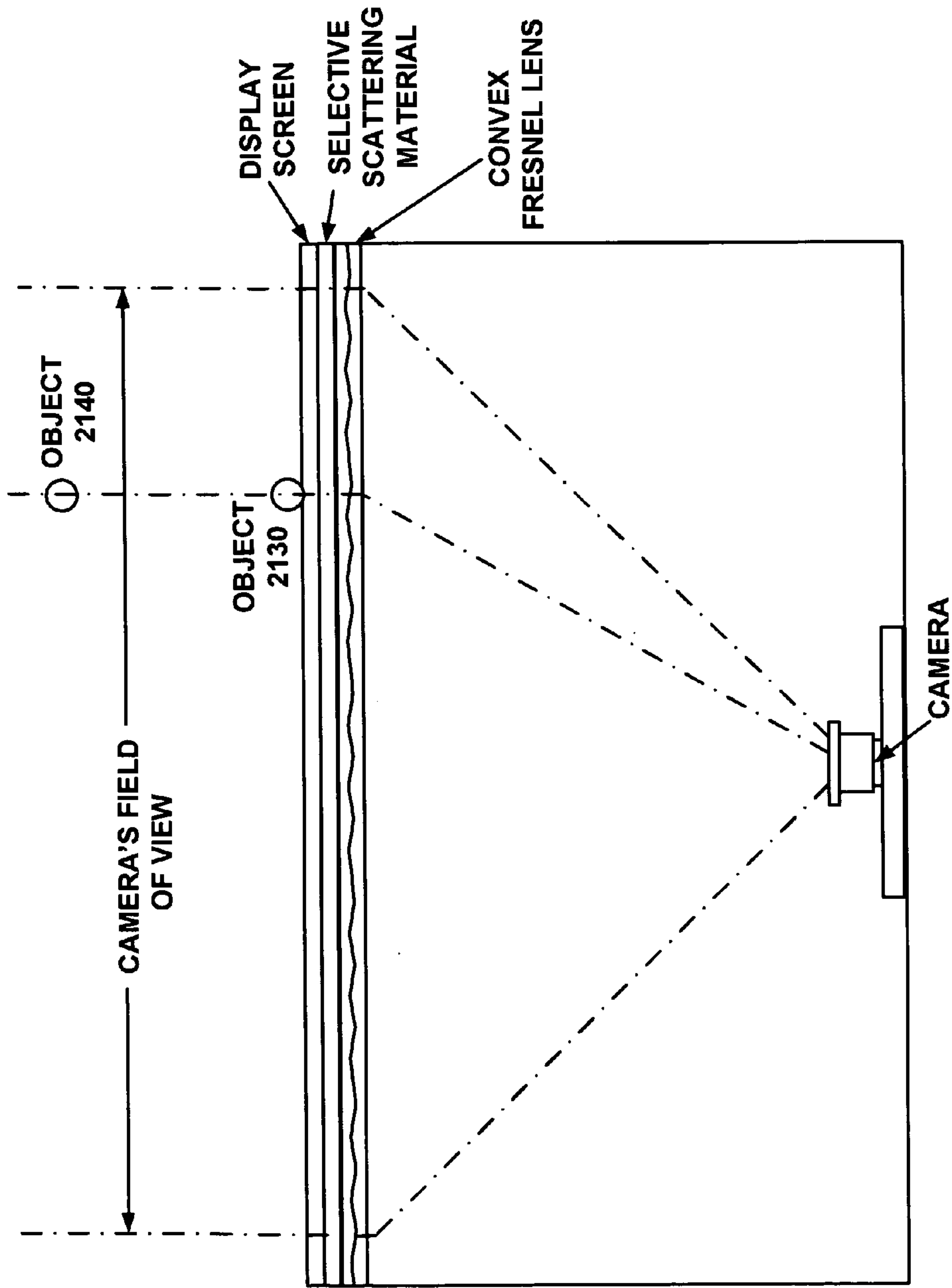
DISTORTION ELIMINATED USING FRESNEL LENS
