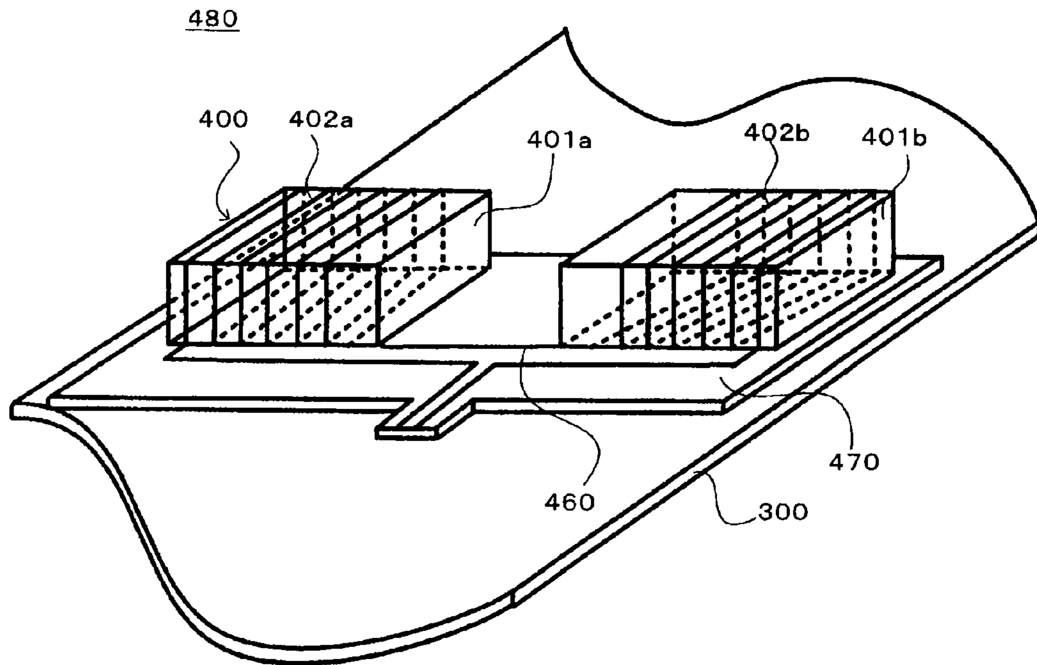
FIG. 17 Prior Art
