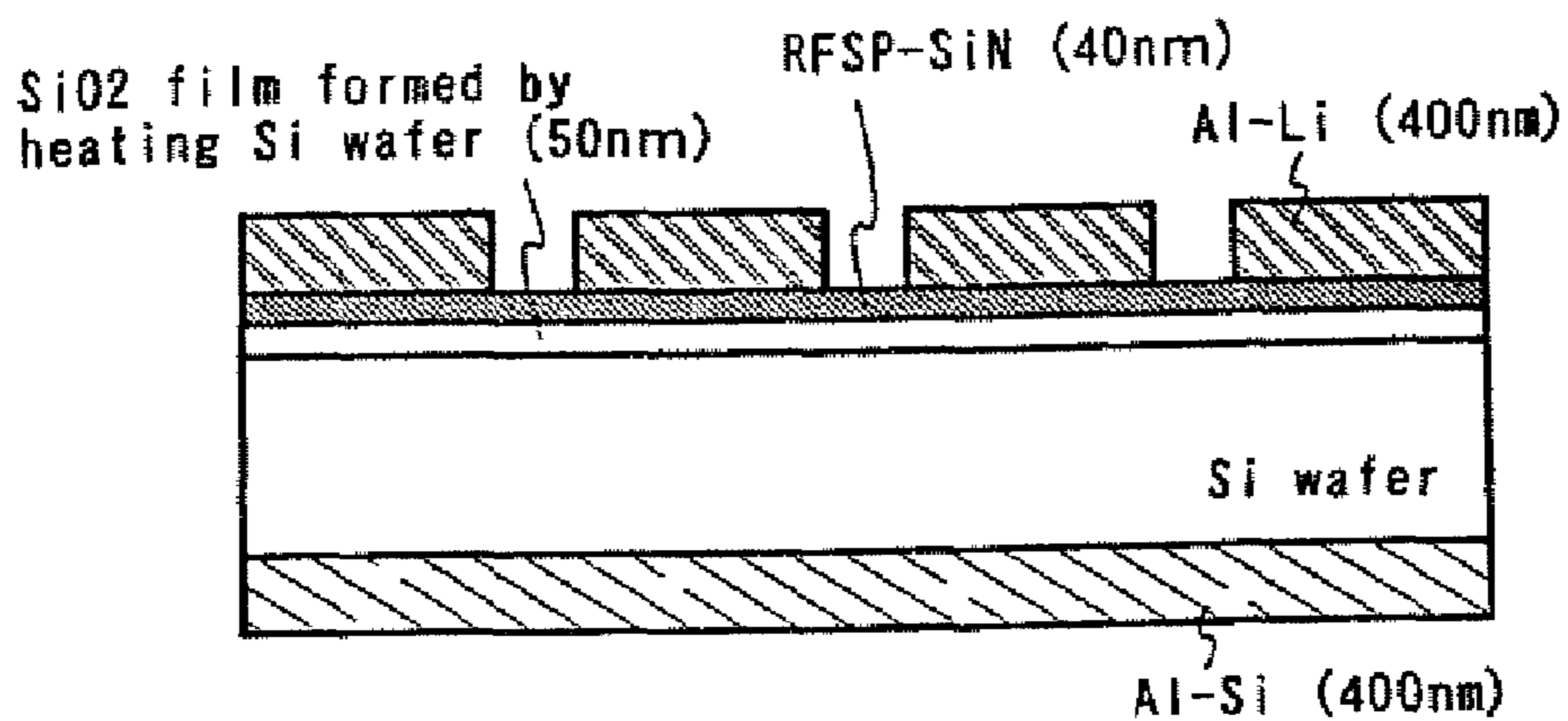
Fig. 29 B MOS structure comprising RFSP-SiN film
