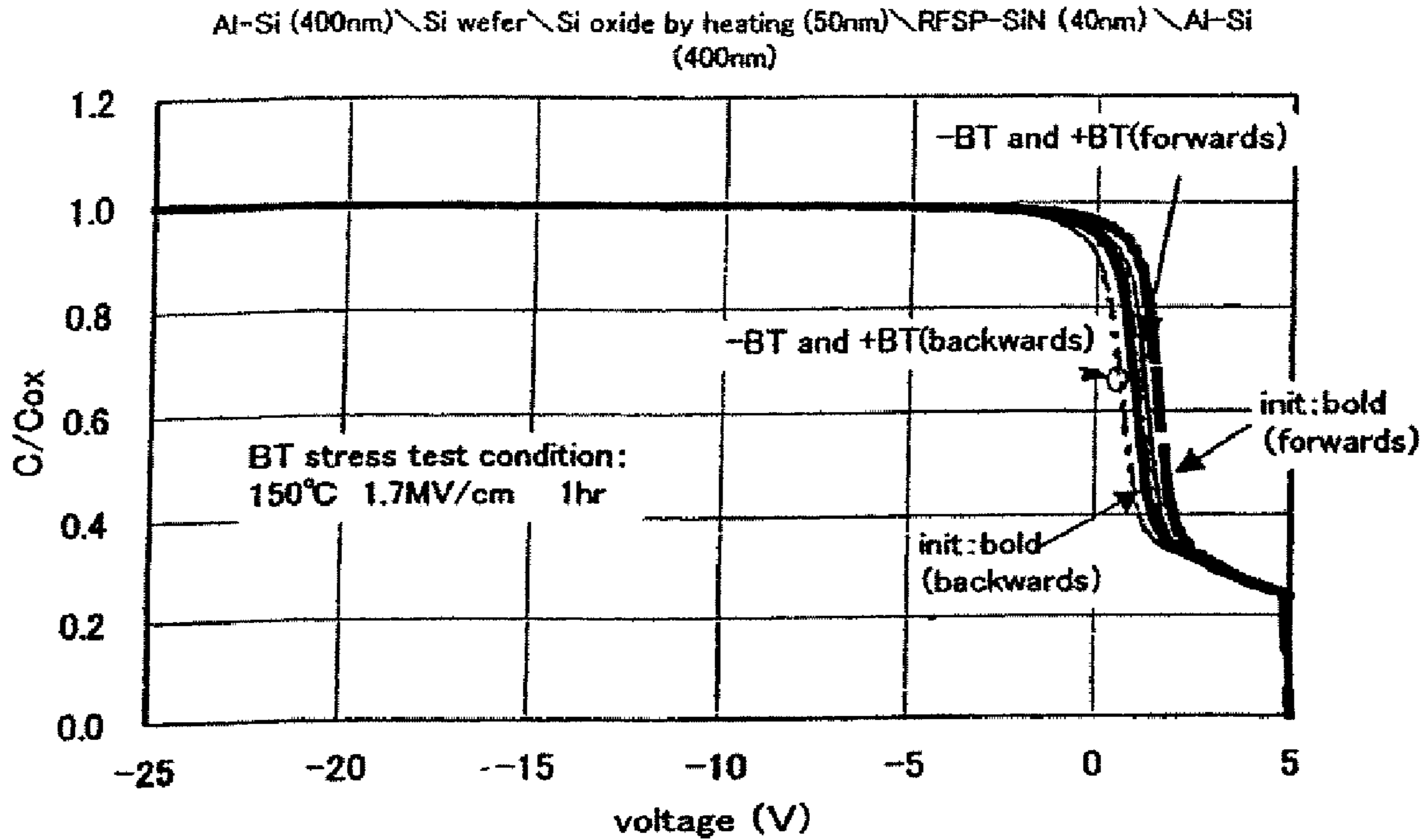
C-V characteristics of MOS structure in case that there is not a source of Li diffusion
