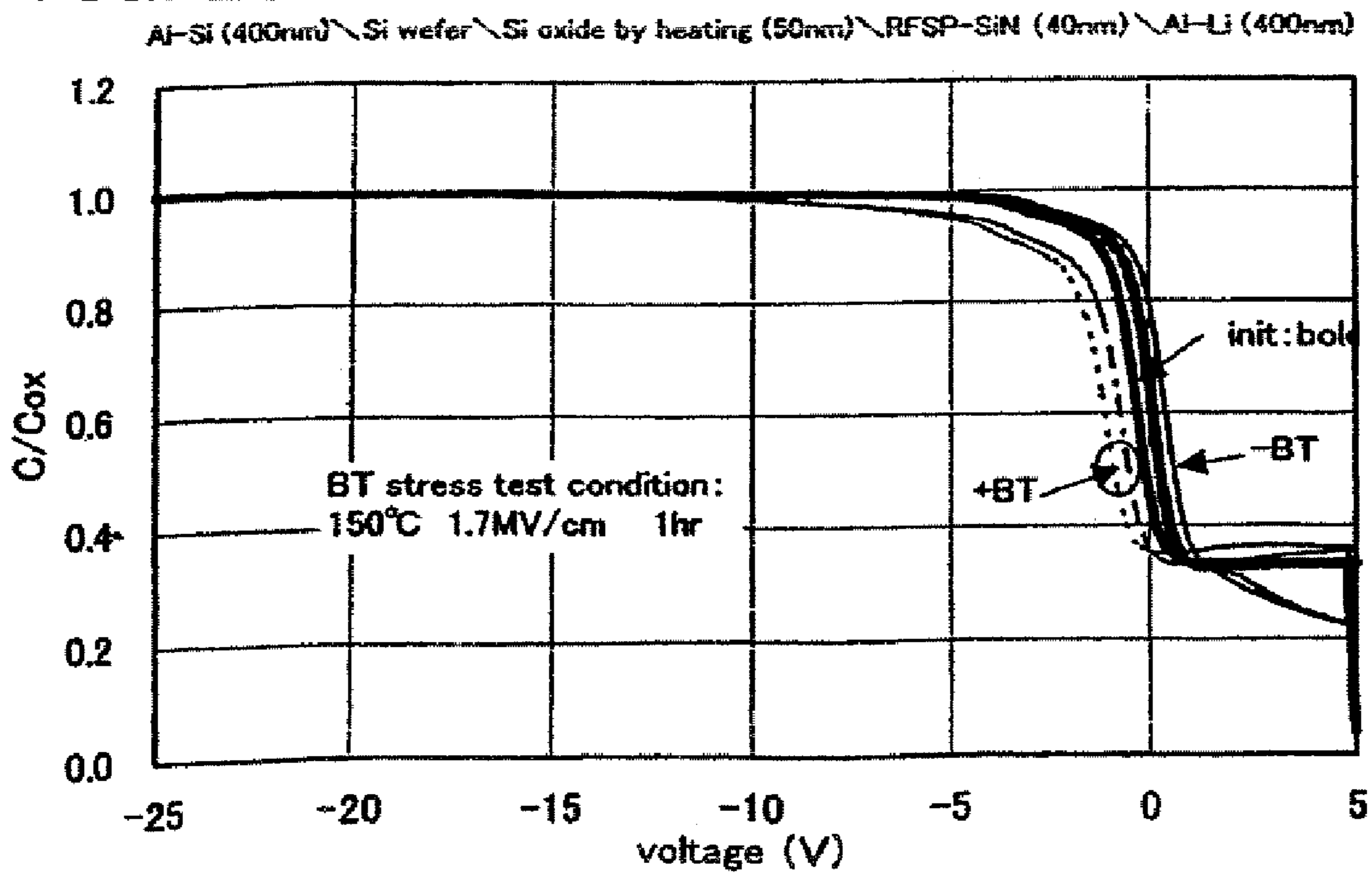
C-V characteristics of MOS structure in case that there is not a source of Li diffusion
