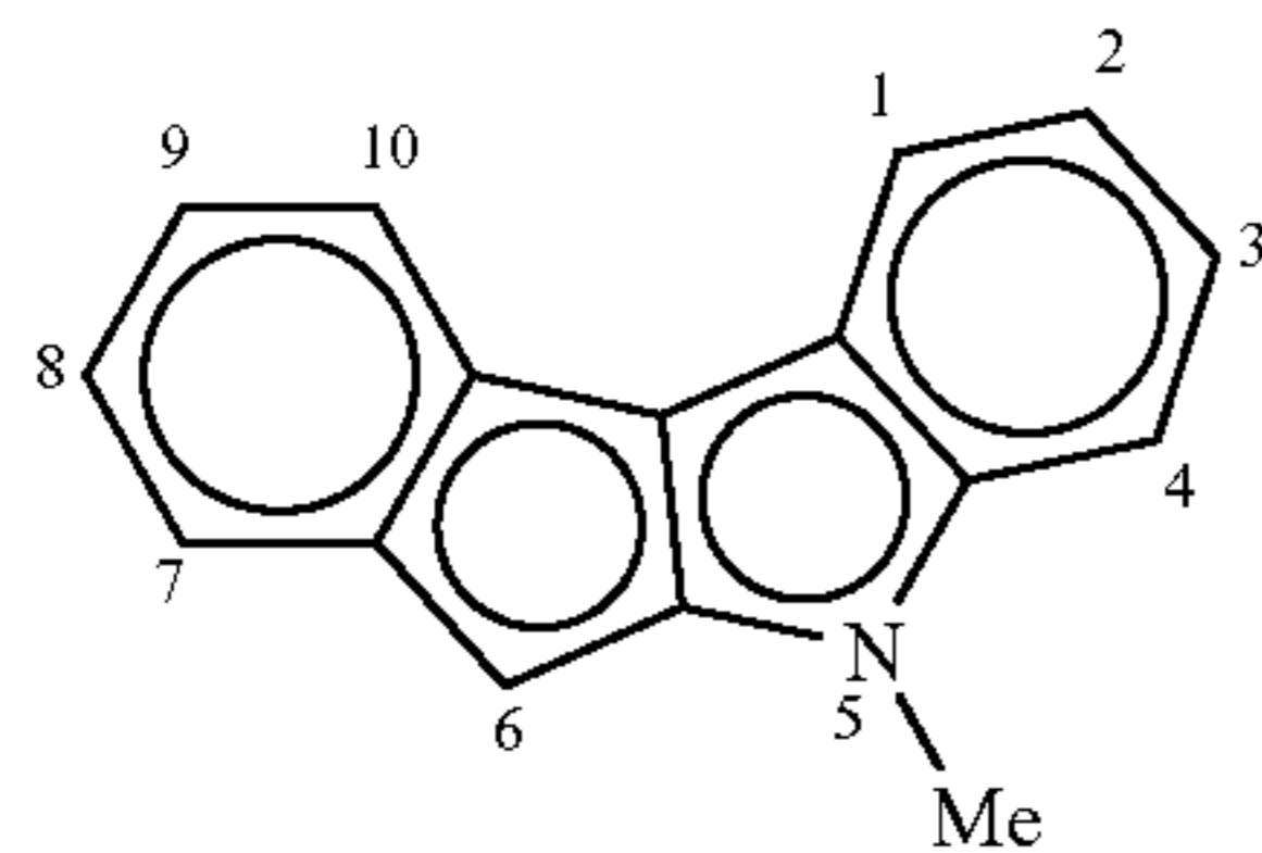
5-methylindeno[2,1-b]indolyl
