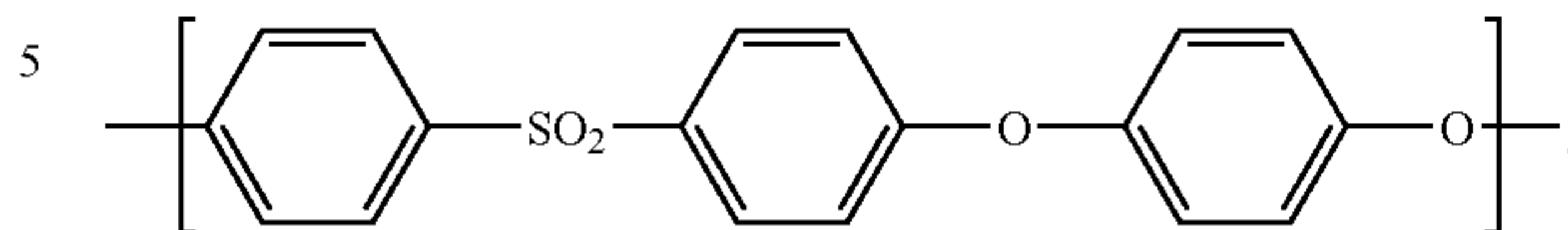
polyetherethersulfone
