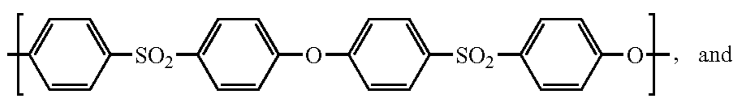
polyethersulfone
