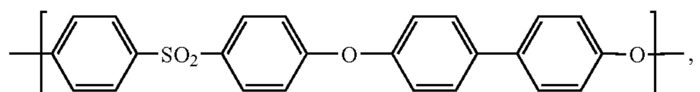
polyphenylsulfone
