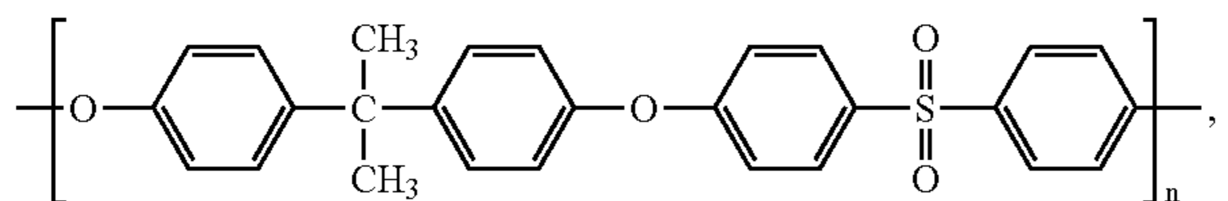
polysulfone
