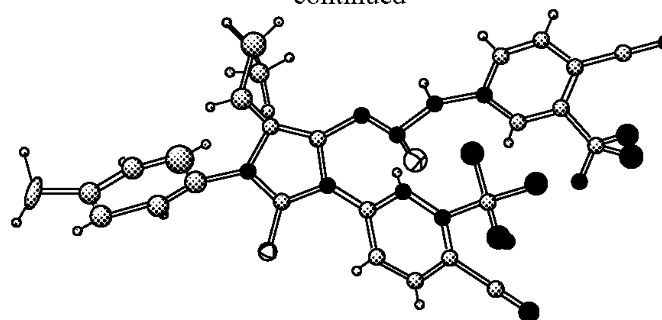
X-ray structure of 35a
