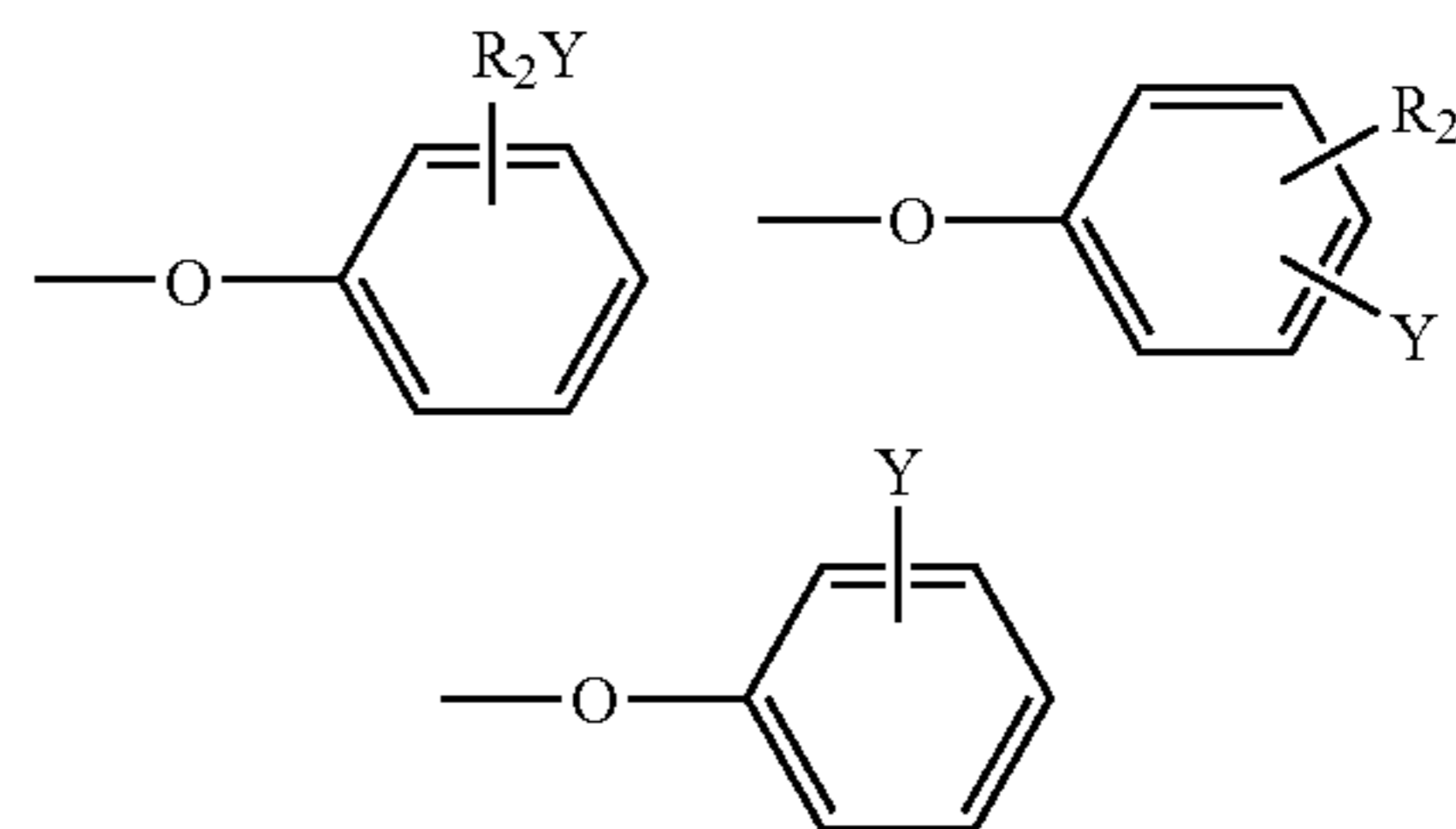
Chemical Formula 4
