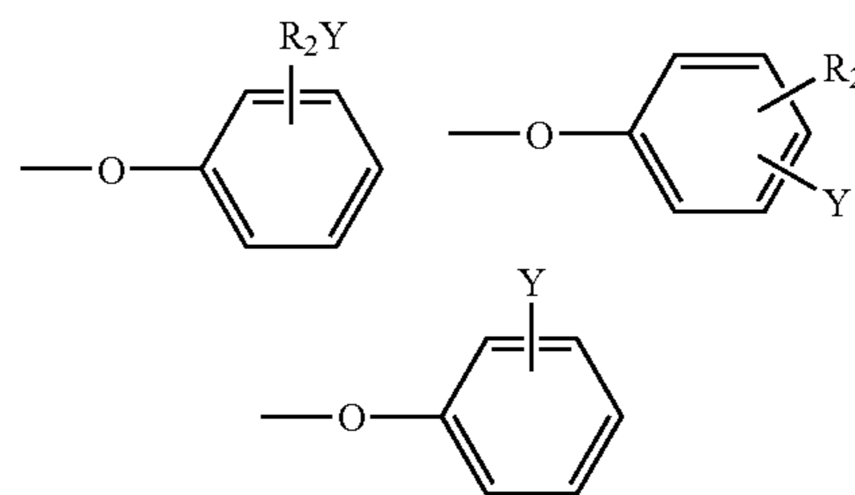
Chemical Formula 4
