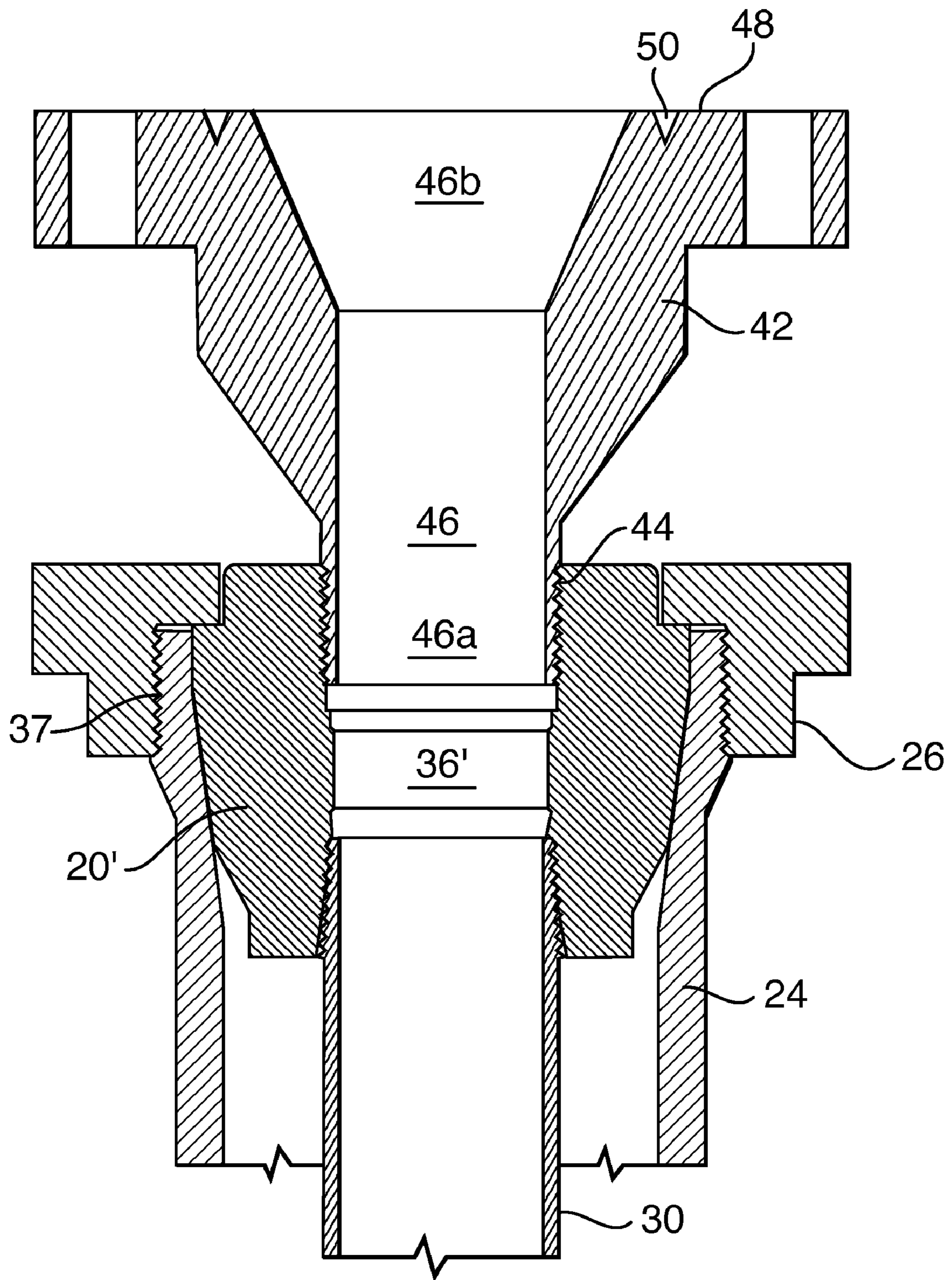
FIG. 3 PRIOR ART
