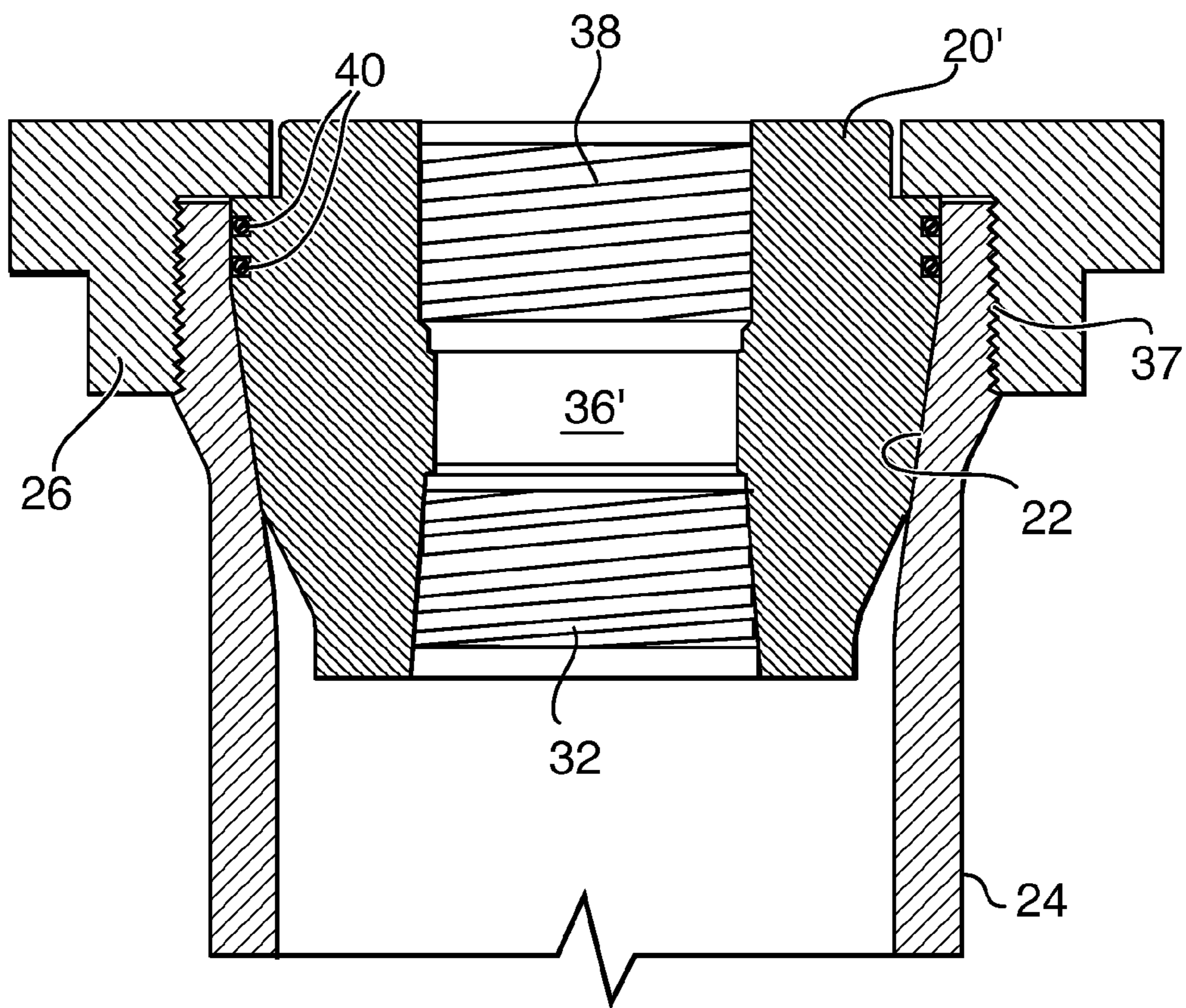
FIG. 2 PRIOR ART
