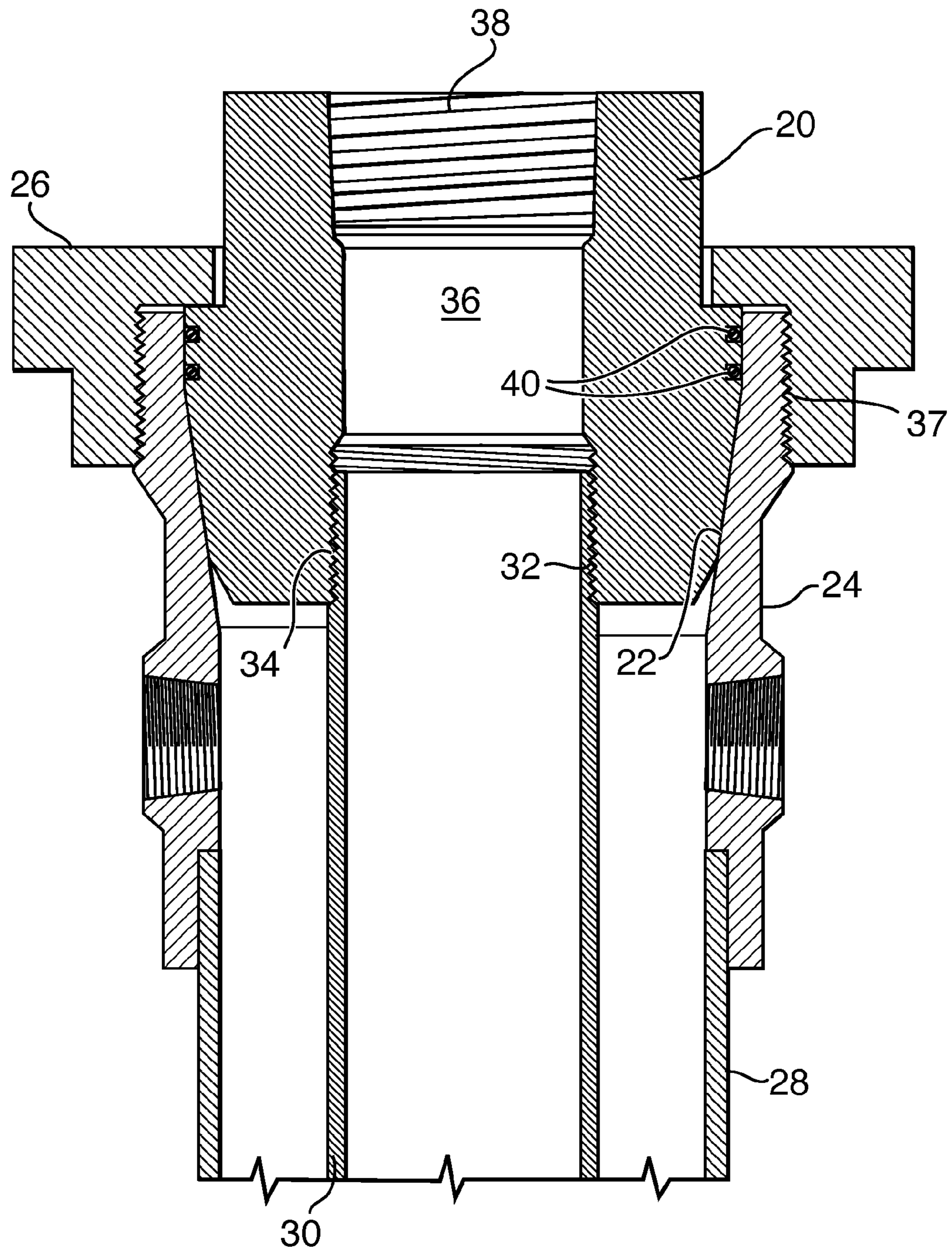
FIG. 1 PRIOR ART
