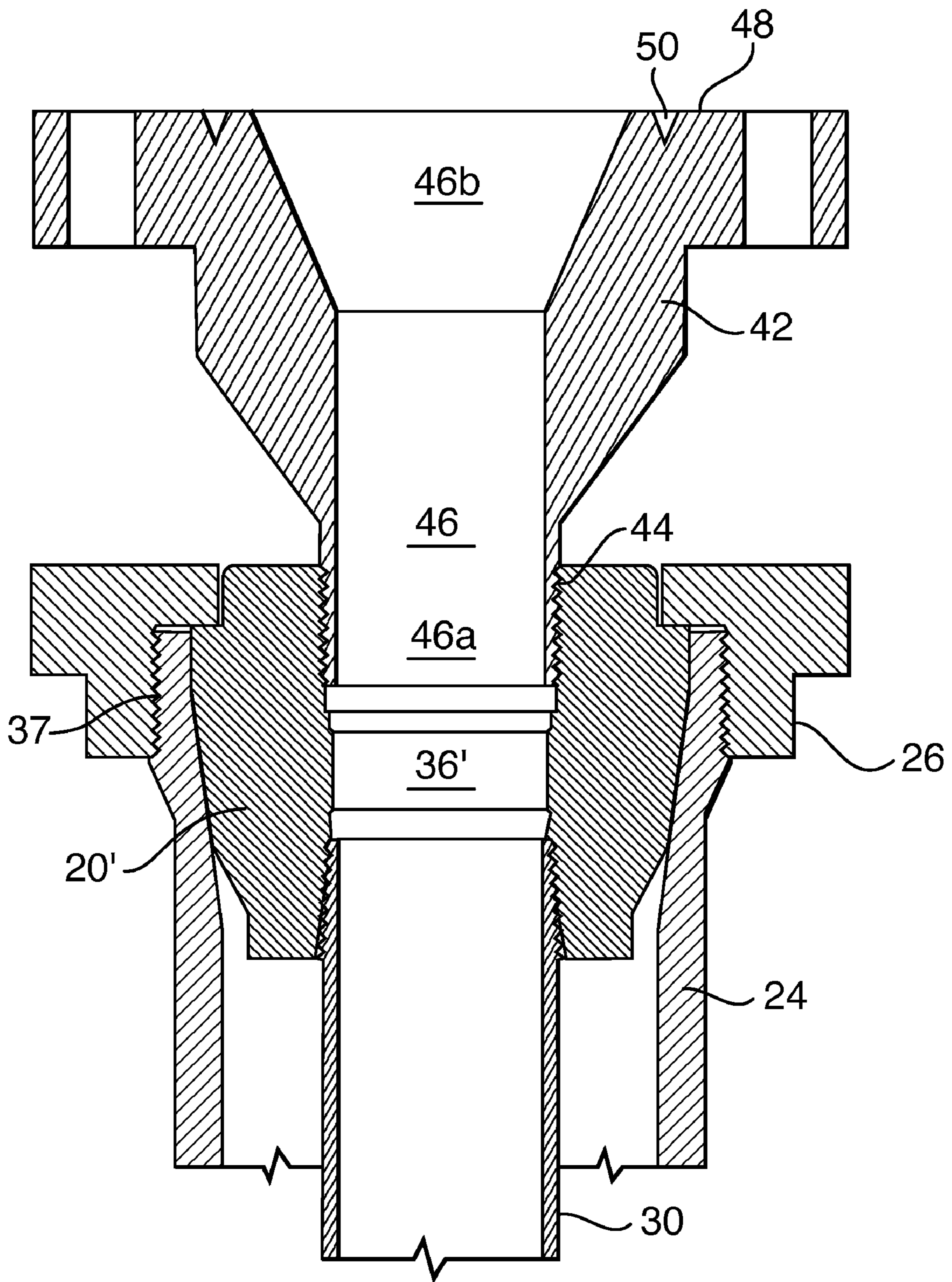
FIG. 3 PRIOR ART
