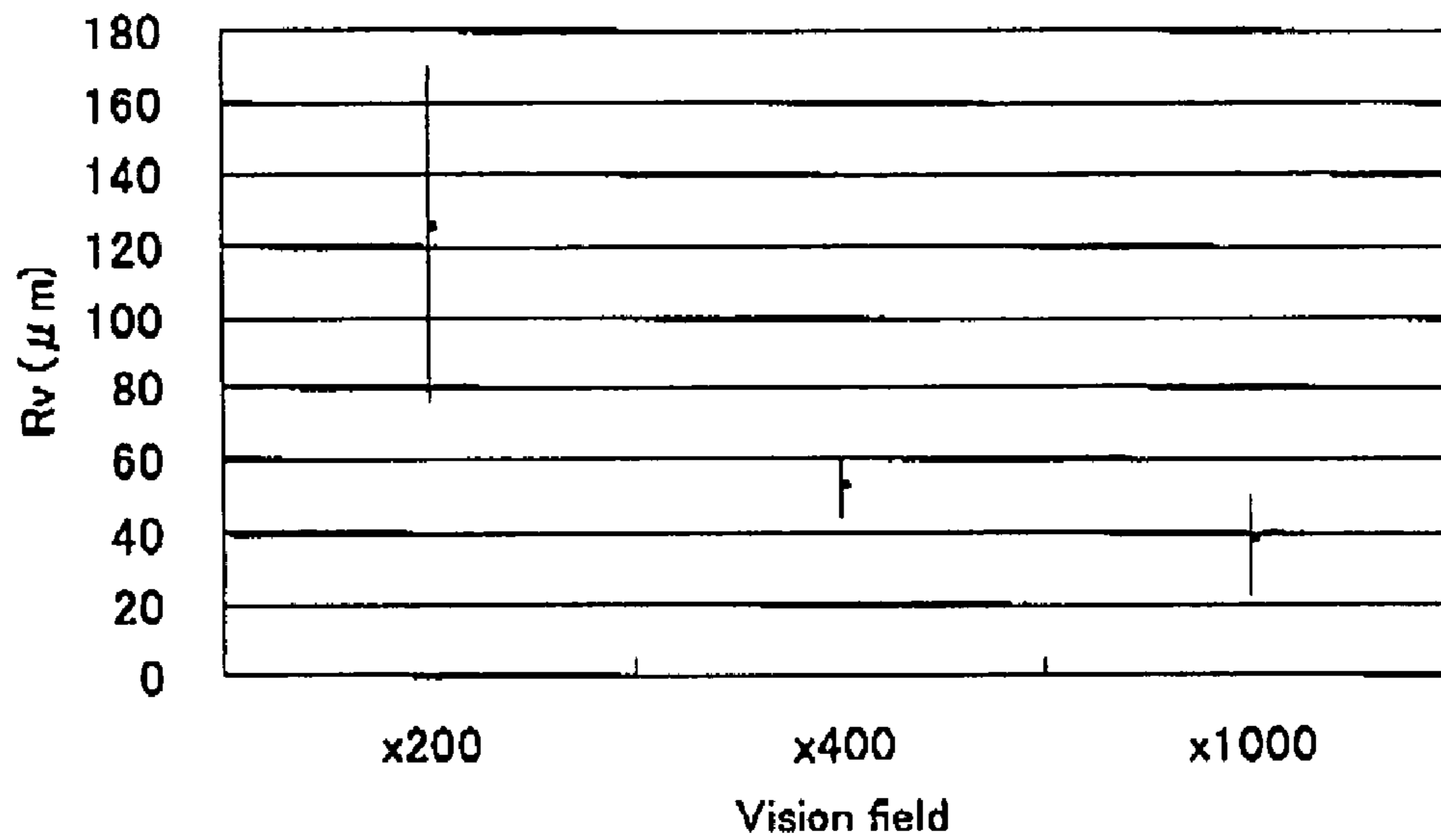
Rv of the roller of Example 4 (JIS B 0601-2001)
