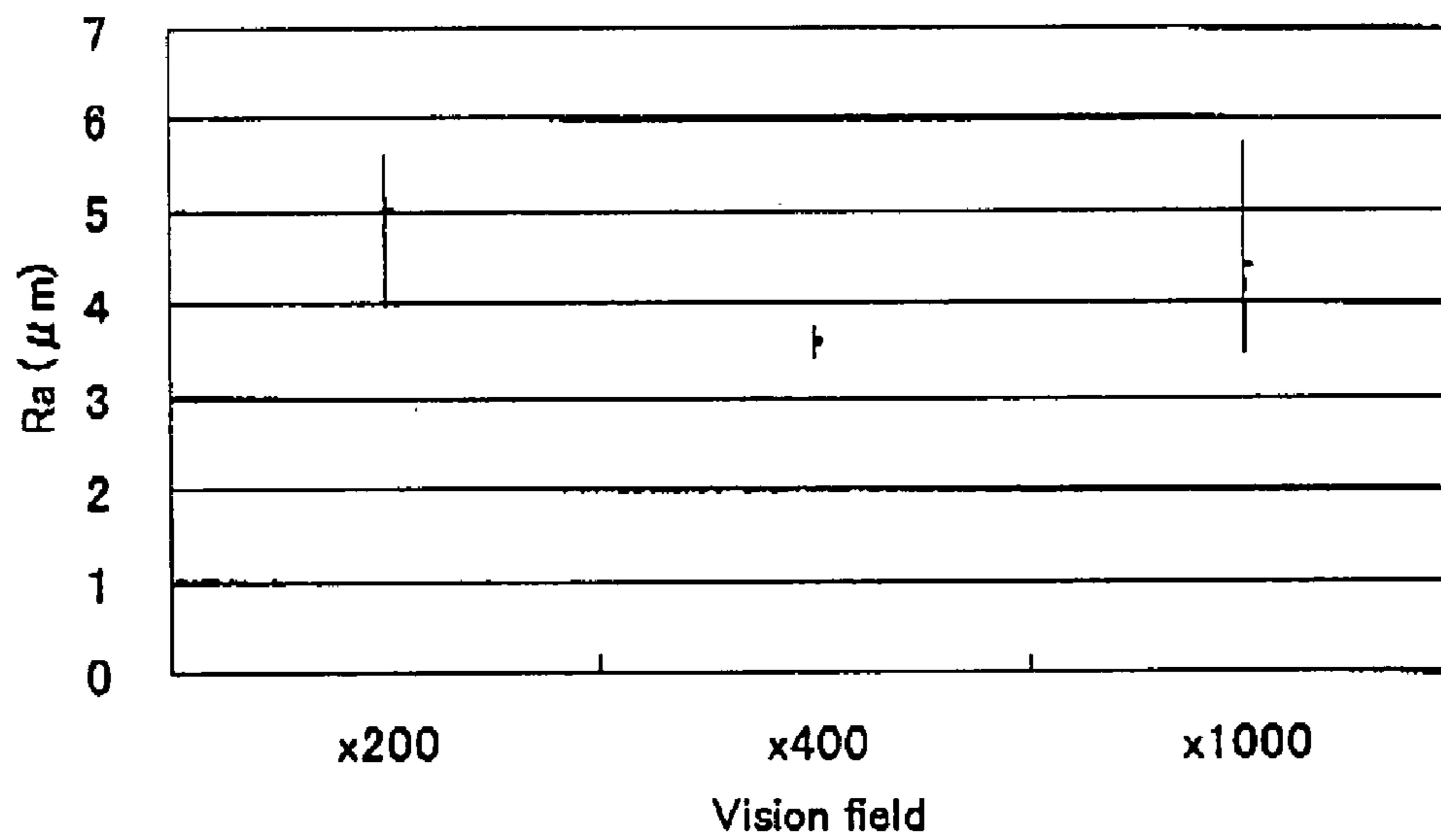
Ra of the roller of Example 4 (JIS B 0601-2001)
