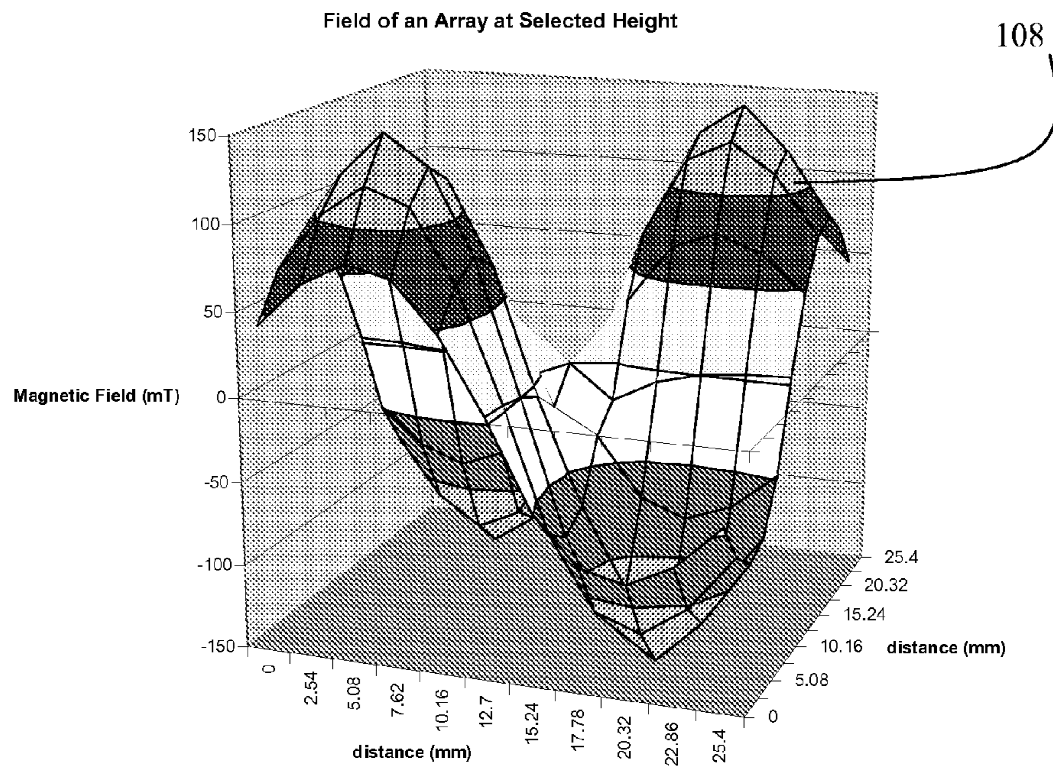
Figure 8. Example QMA Magnetic Field plot.
