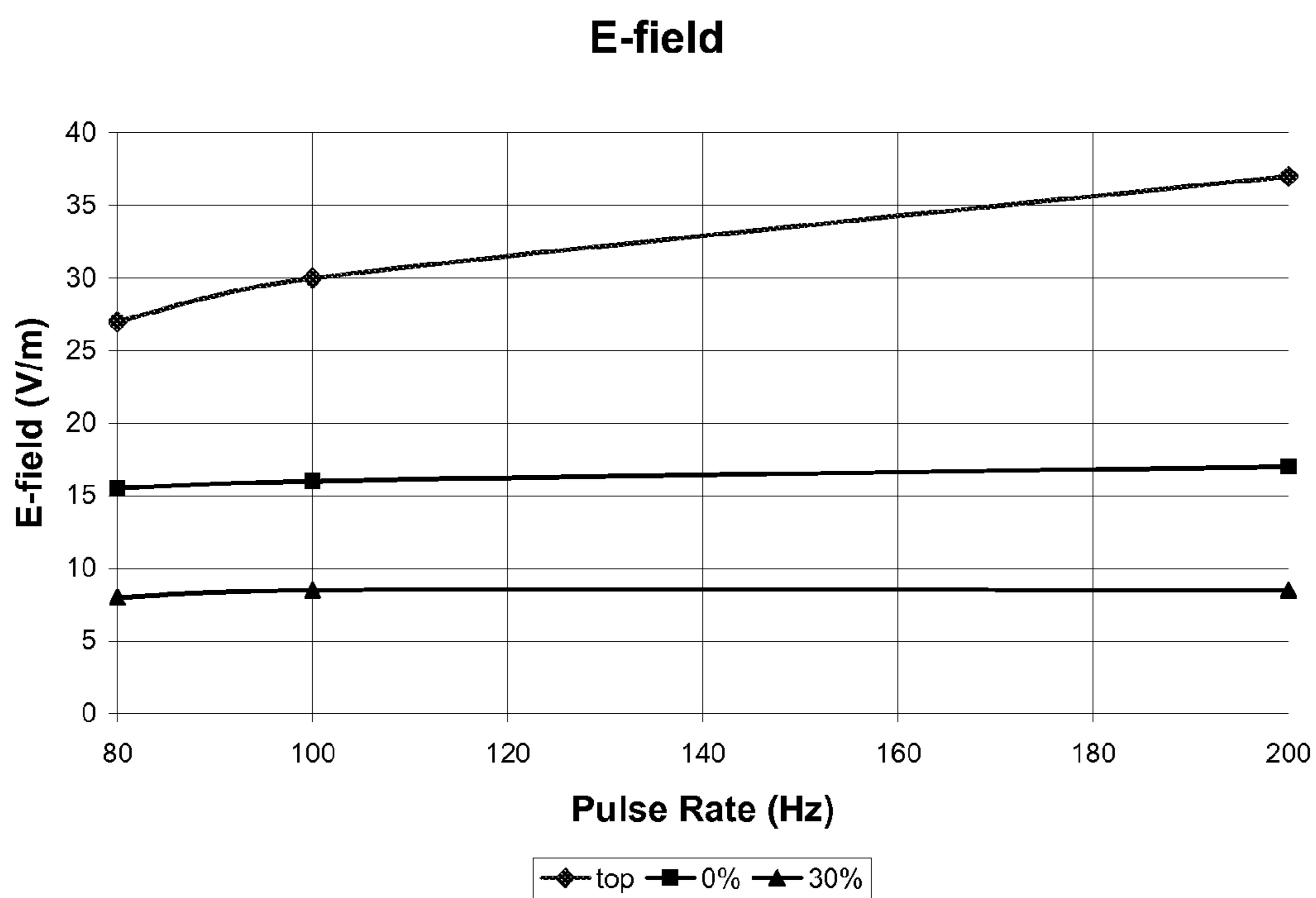
Figure 10. E-fields at Top and Bottom of Flesh
