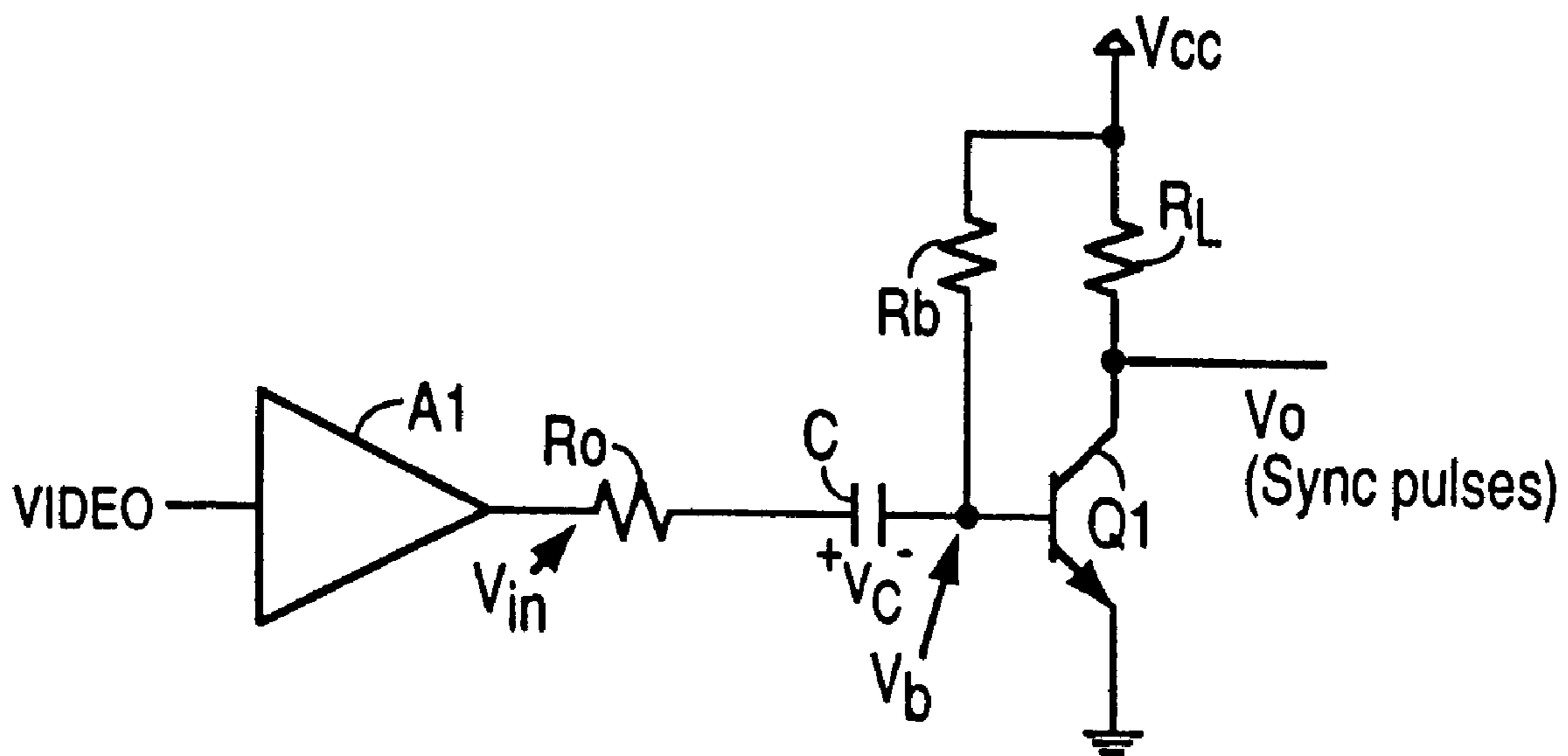
FIG. 10 (PRIOR ART)
