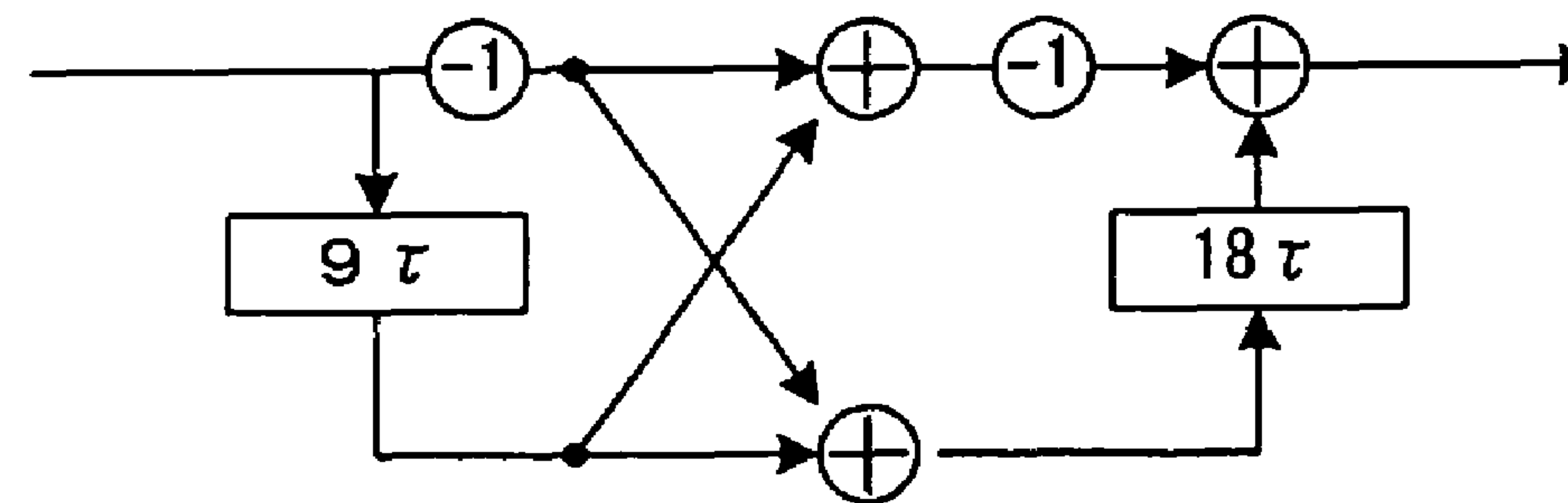
FIG. 12D D MATCHED FILTER
