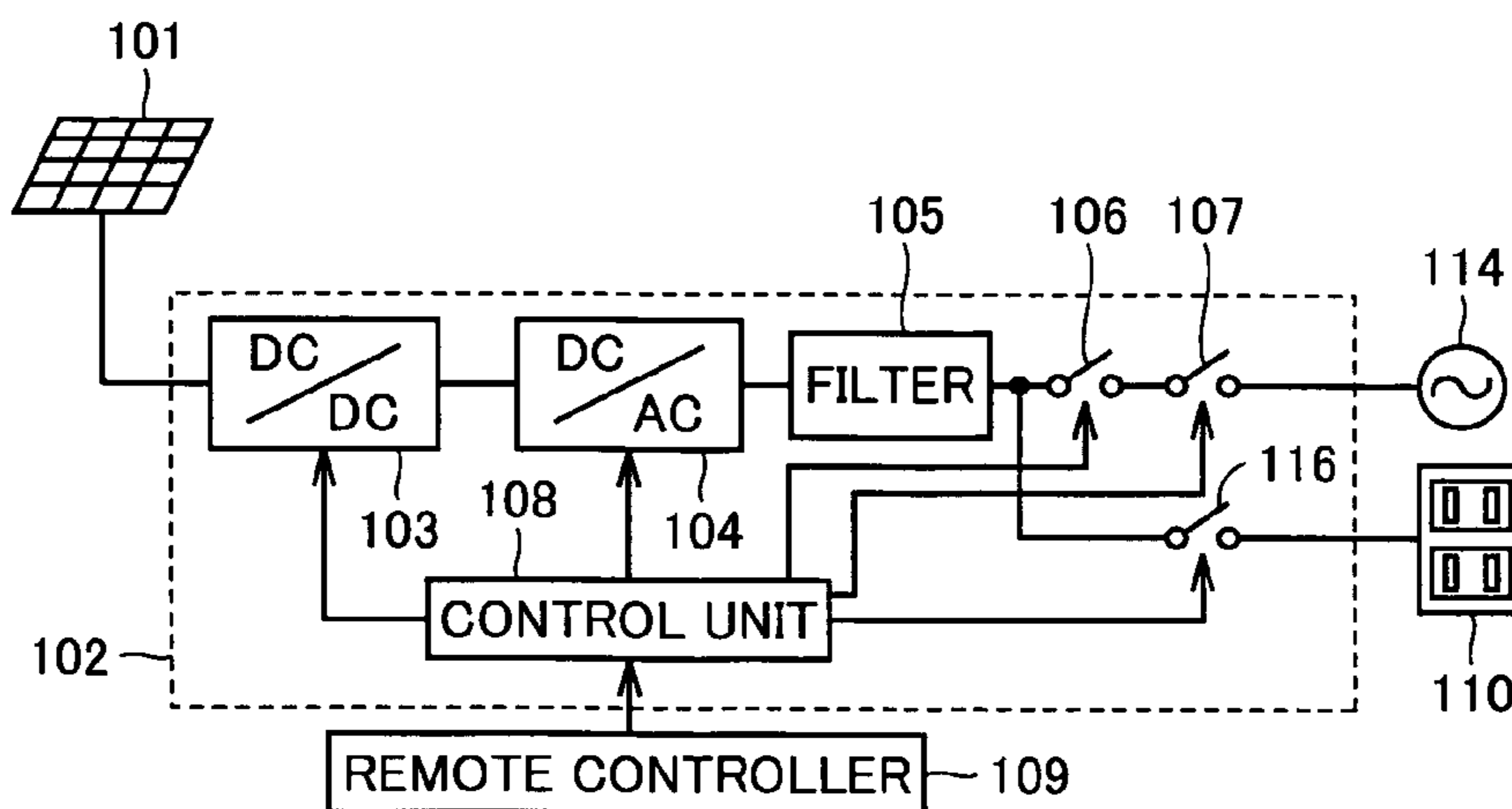
FIG.5 PRIOR ART
