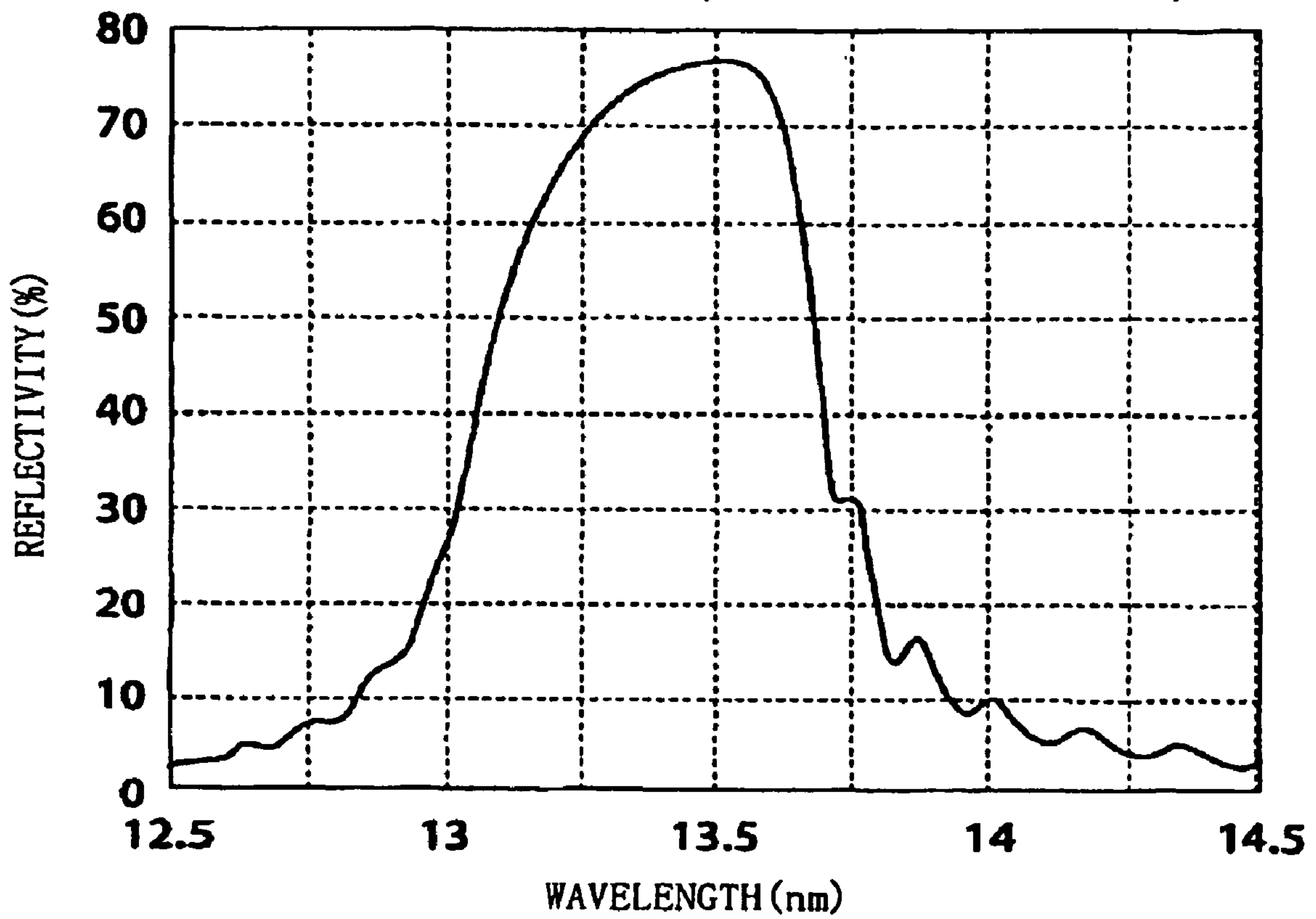
SPECTRAL REFLECTIVITY (AT VERTICAL INCIDENCE)
