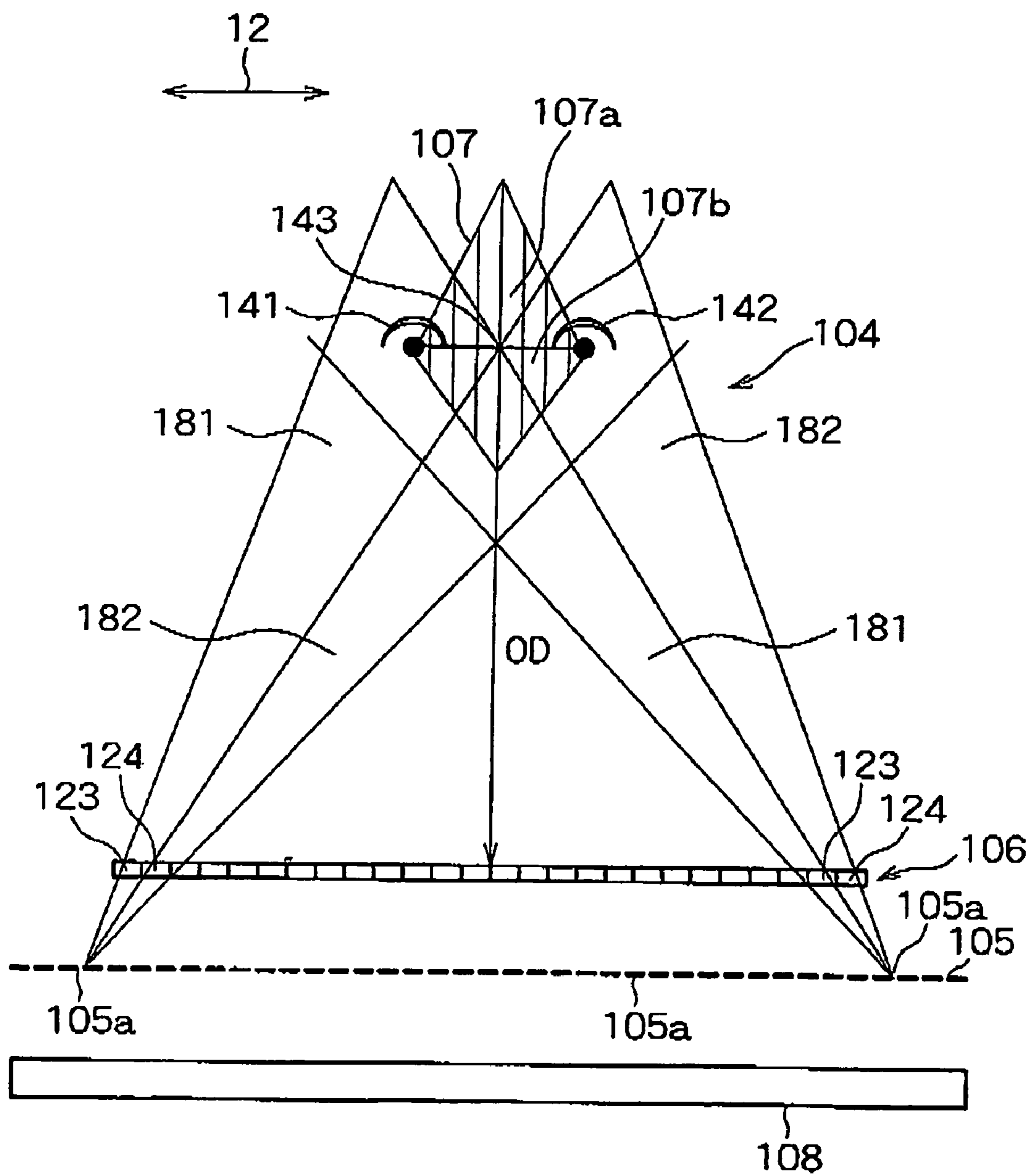
FIG. 1 (PRIOR ART)
