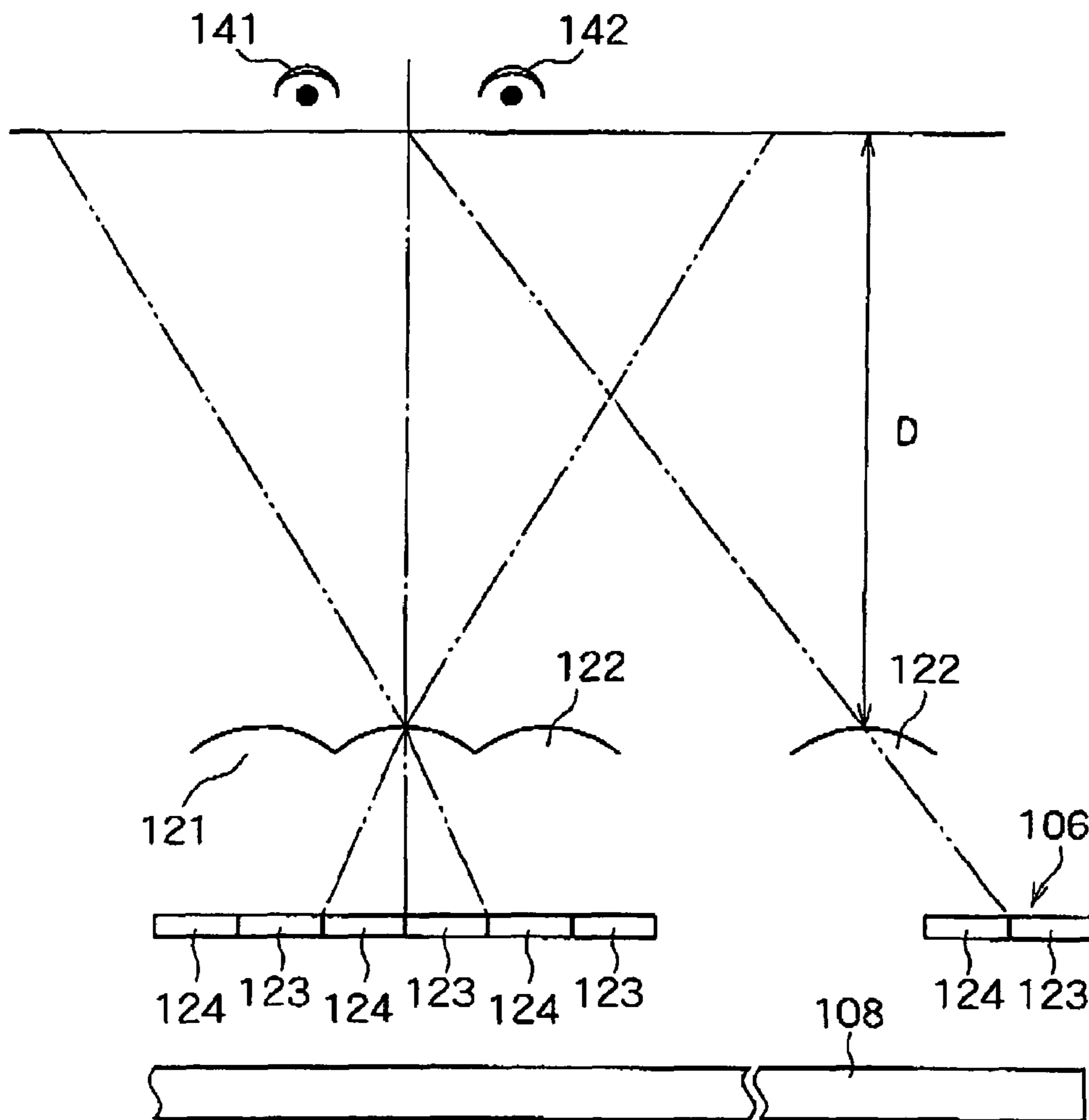
FIG. 3 (PRIOR ART)
