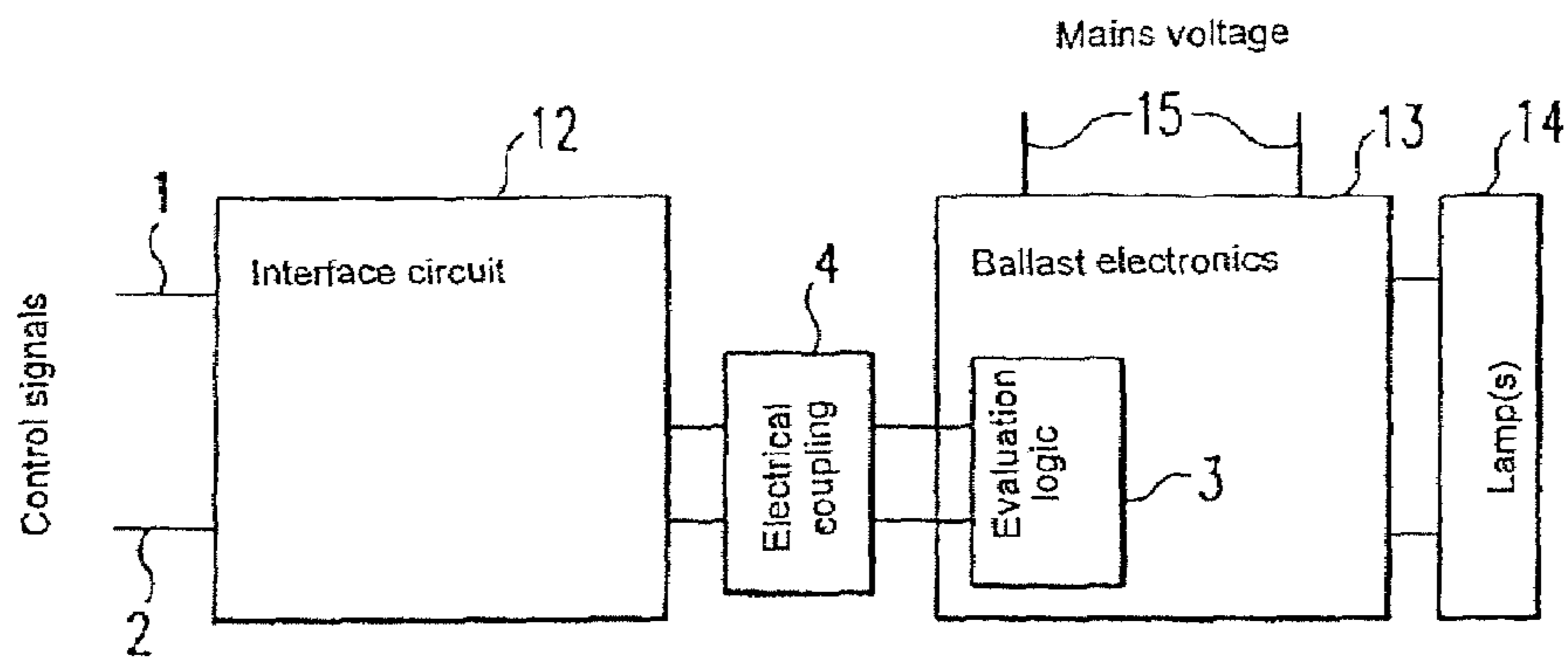
Fig. 6 PRIOR ART
