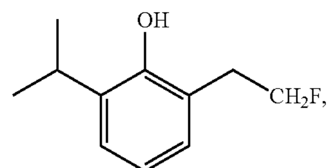
2-(2-Fluoro-ethyl)-6-isopropyl-phenol
