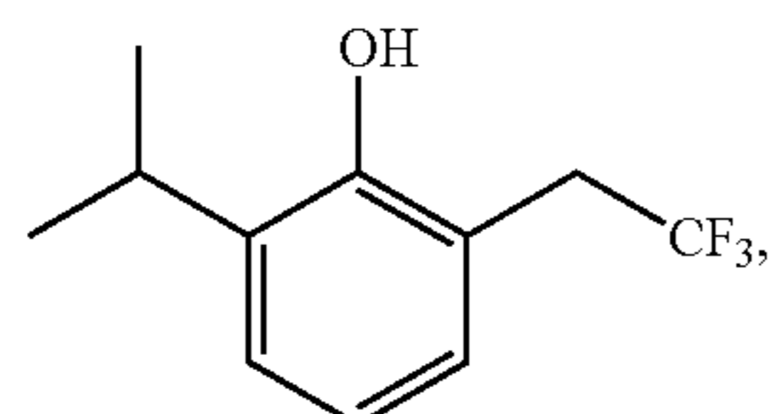
2-Isopropyl-6-(2,2,2-trifluoro-ethyl)-phenol
