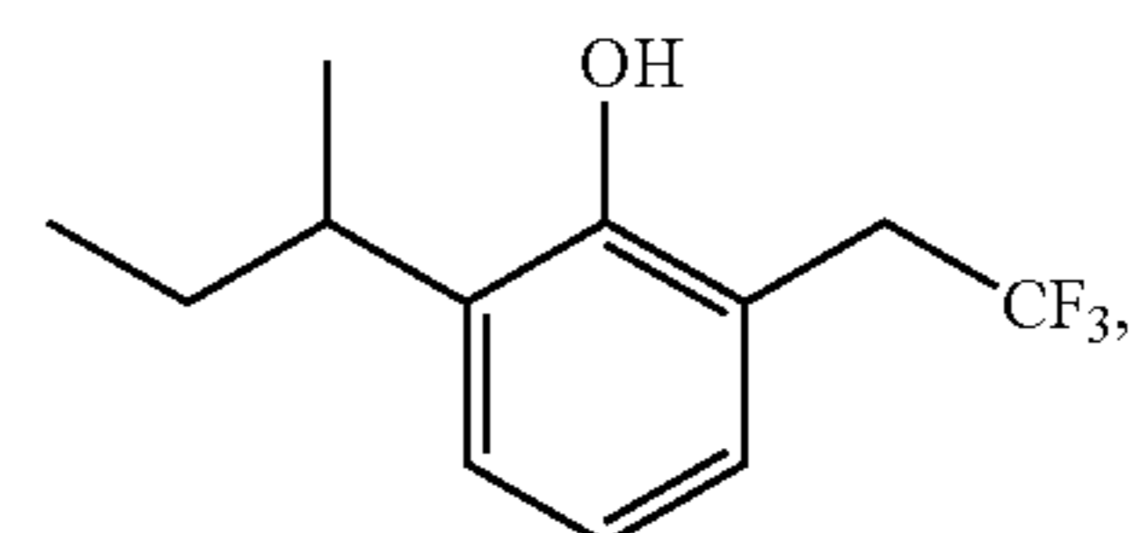
2-sec-Butyl-6-(2,2,2-trifluoro-ethyl)-phenol
