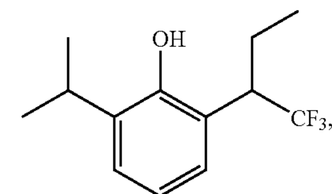
2-Isopropyl-6-(1-trifluoromethyl-propyl)-phenol
