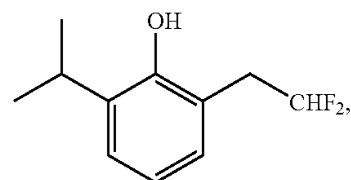
2-(2,2-Difluoro-ethyl)-6-isopropyl-phenol
