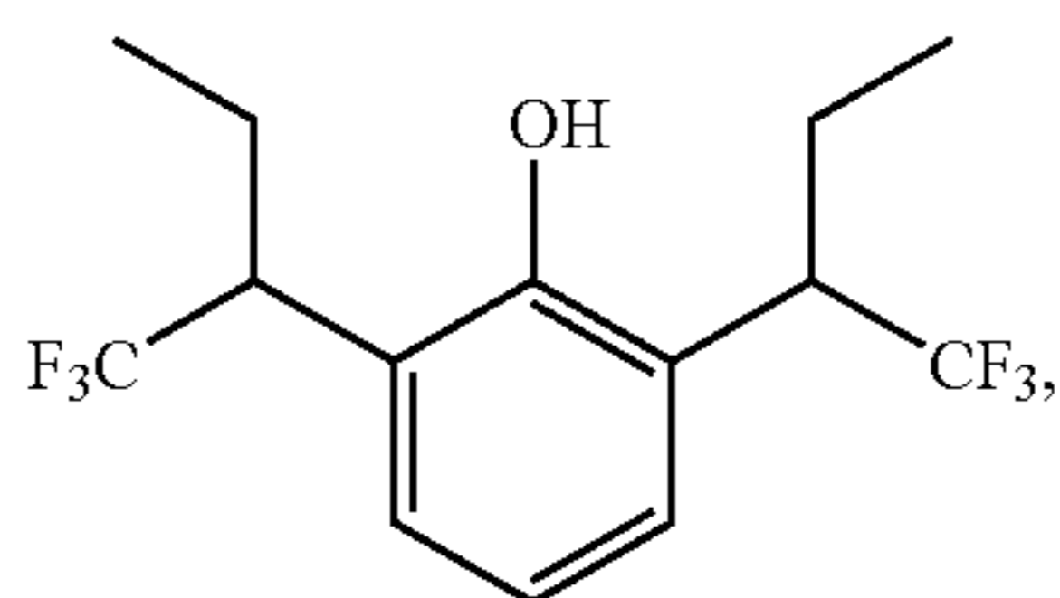
2,6-Bis-(1-trifluoromethyl-propyl)-phenol
