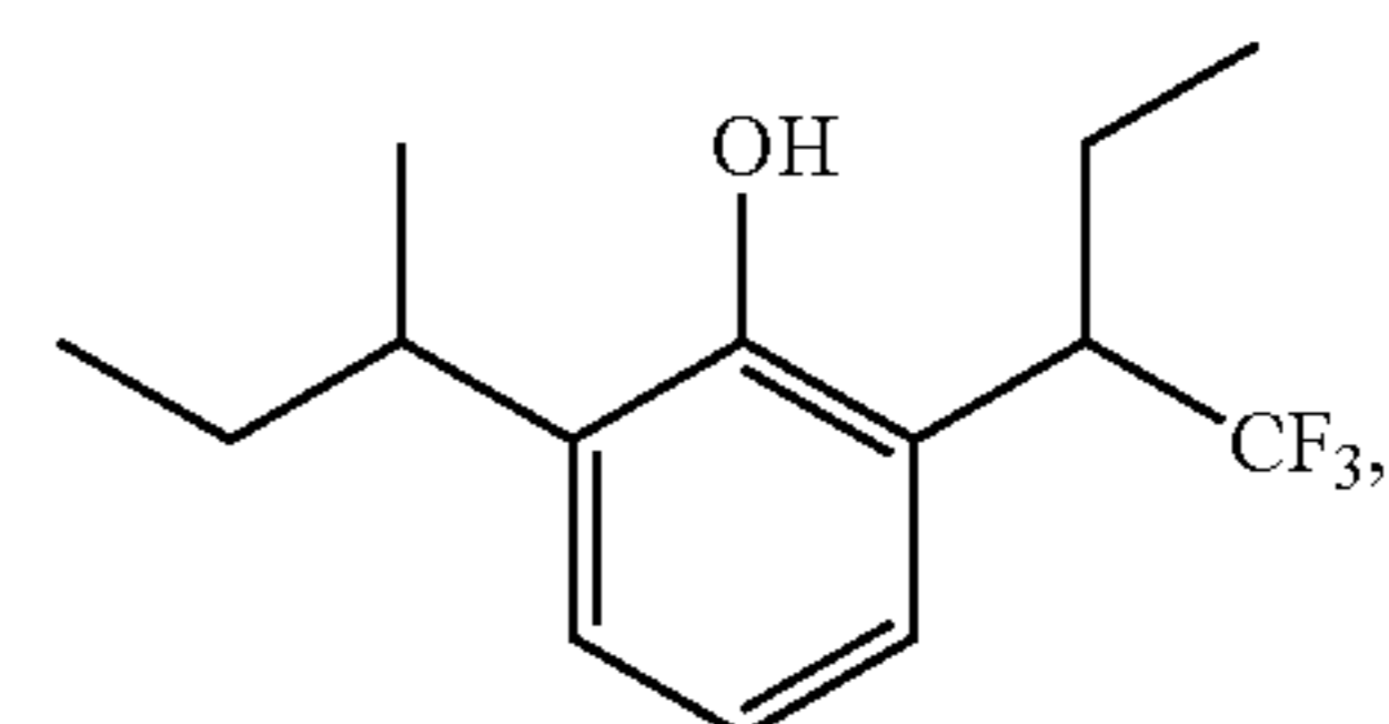
2-sec-Butyl-6-(1-trifluoromethyl-propyl)-phenol
