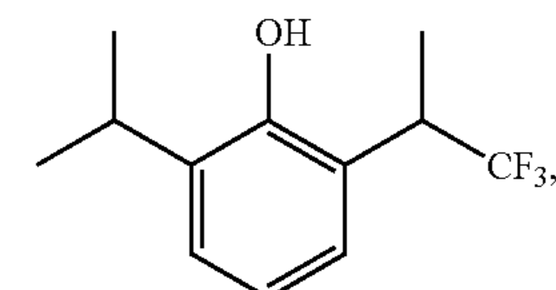
2-Isopropyl-6-(2,2,2-trifluoro-1-methyl-ethyl)-phenol
