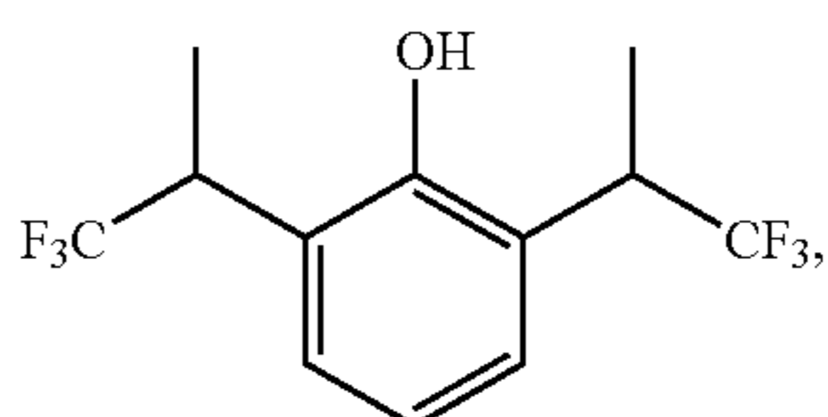
2,6-Bis-(2,2,2-trifluoro-1-methyl-ethyl)-phenol
