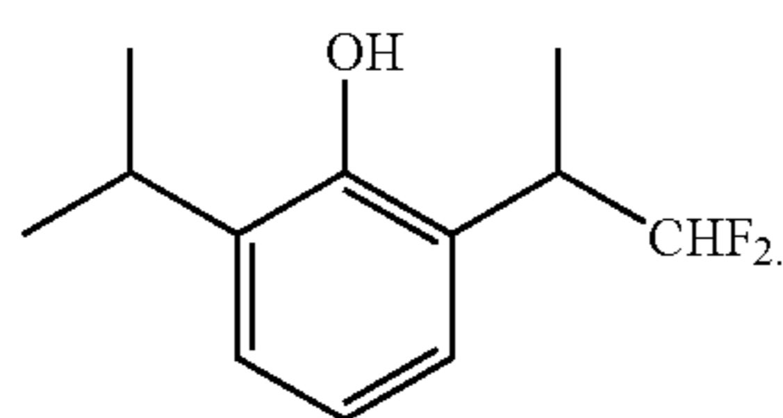
2-(2,2,-Difluoro-1-methyl-ethyl)-6-isopropyl-phenol
