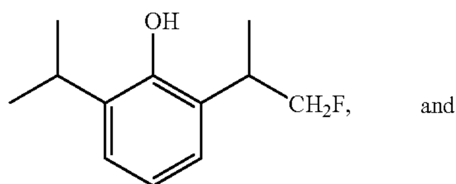
2-(2-Fluoro-1-methyl-ethyl)-6-isopropyl-phenol
