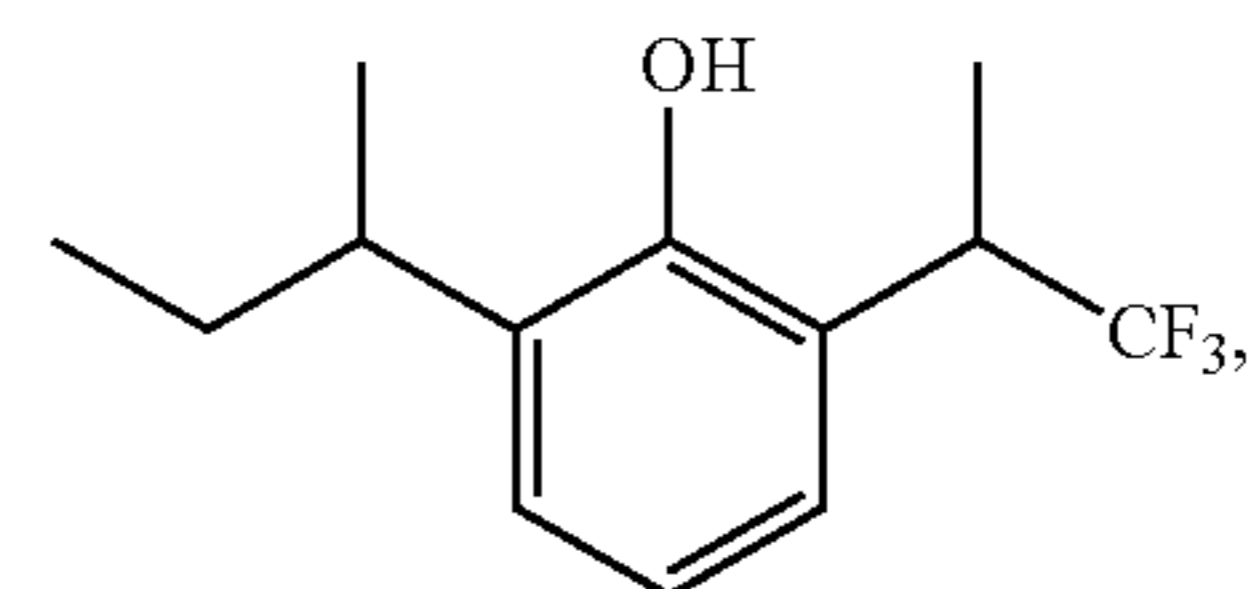
2-sec-Butyl-6-(2,2,2-trifluoro-1-methyl-ethyl)-phenol
