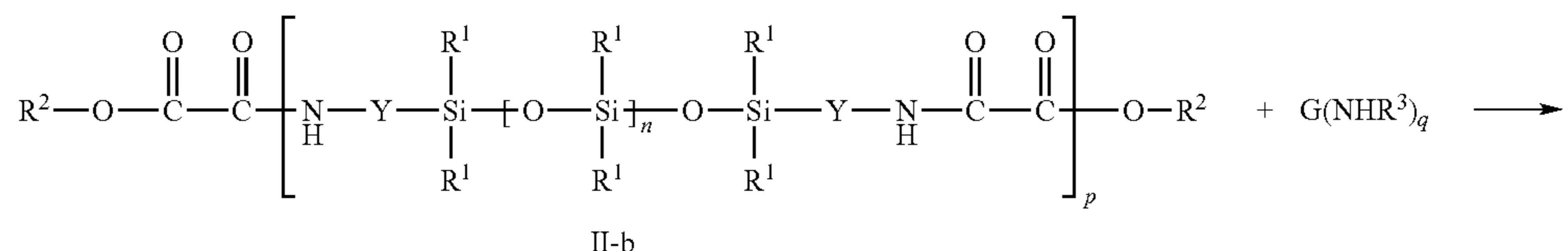
Reaction Scheme A-2
