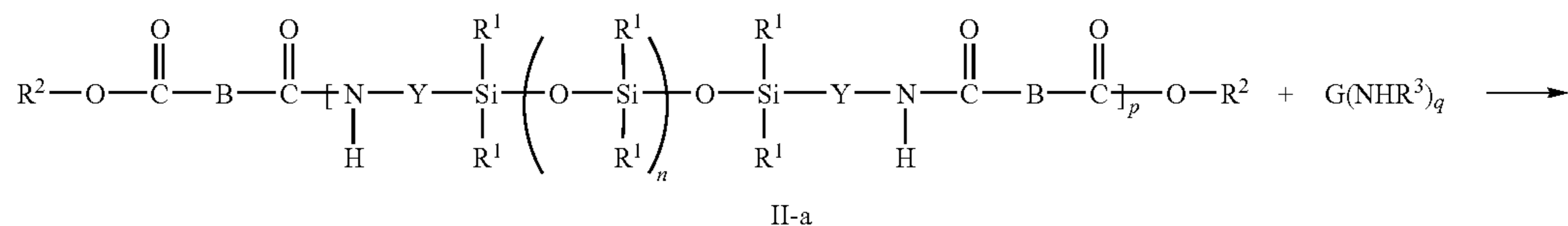
Reaction Scheme A-1
