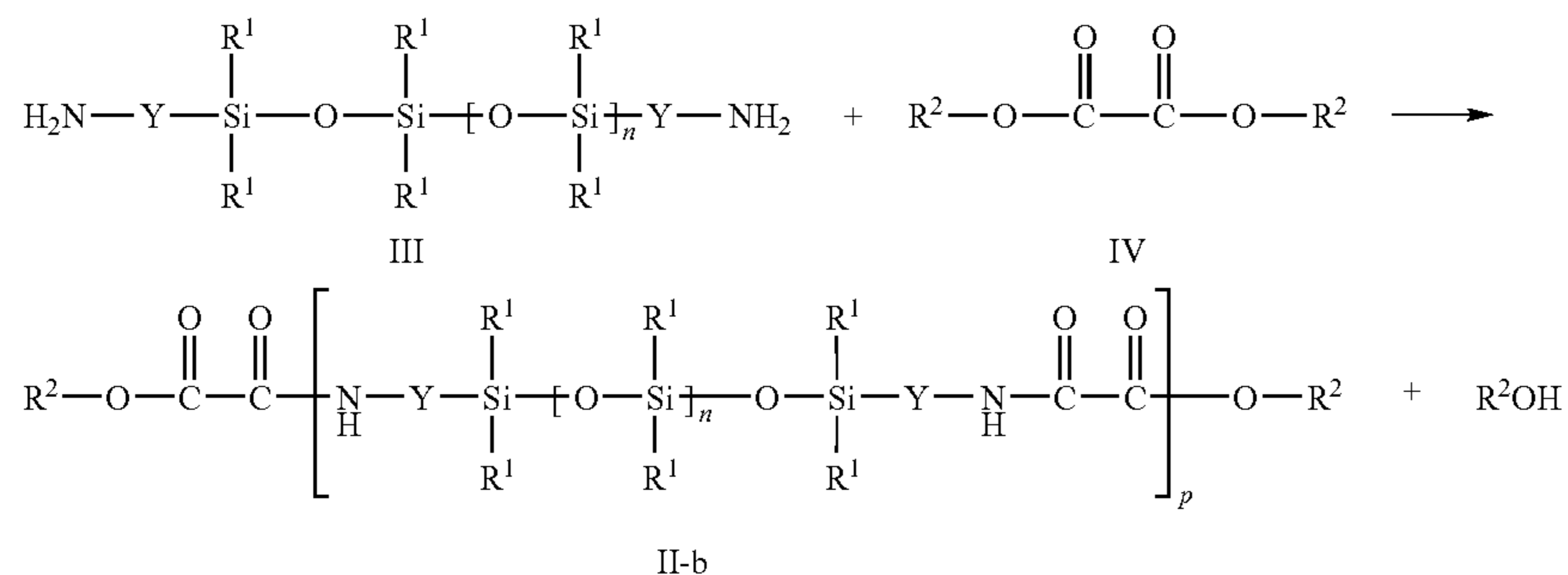
Reaction Scheme B
