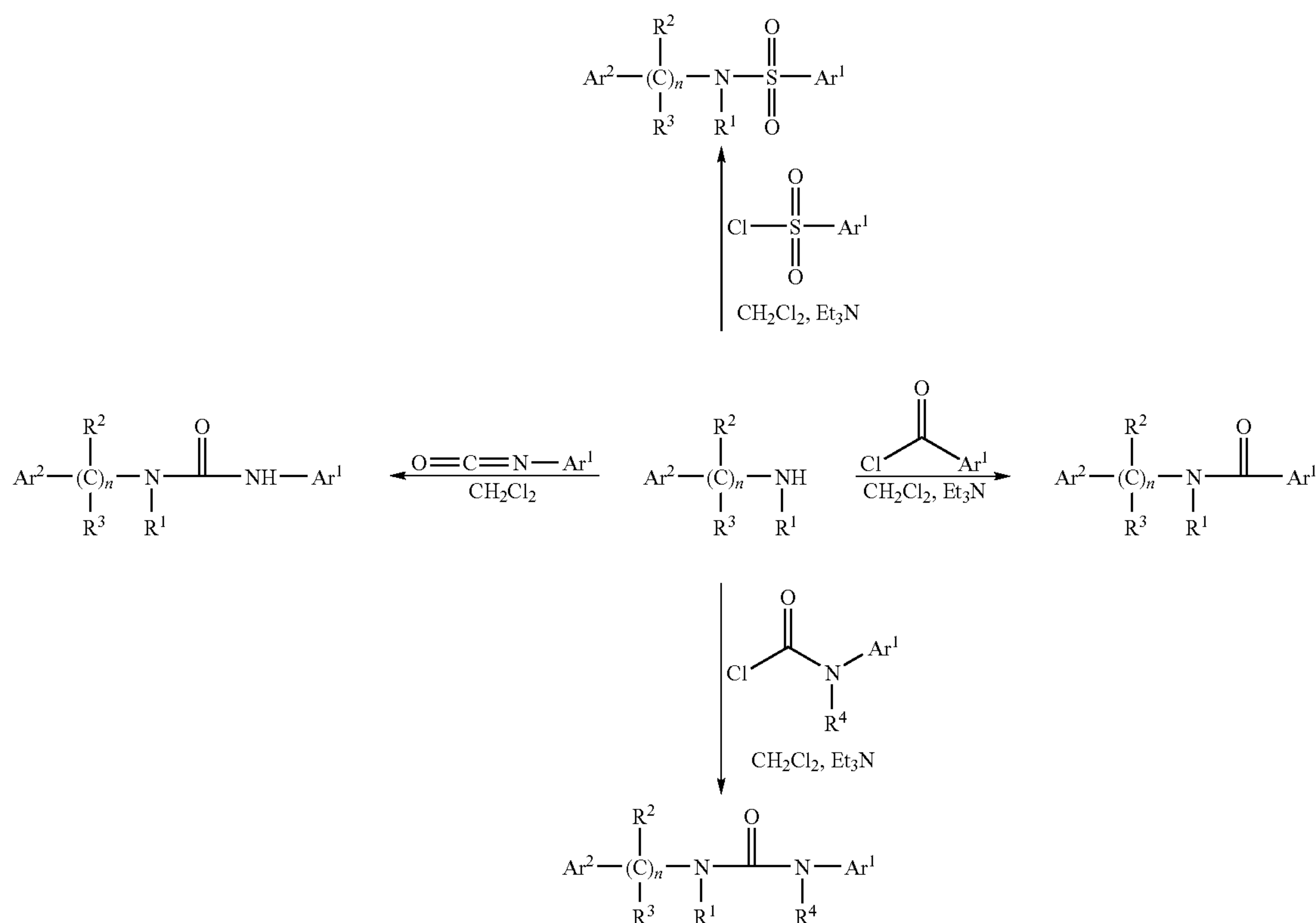
Reaction scheme 1
