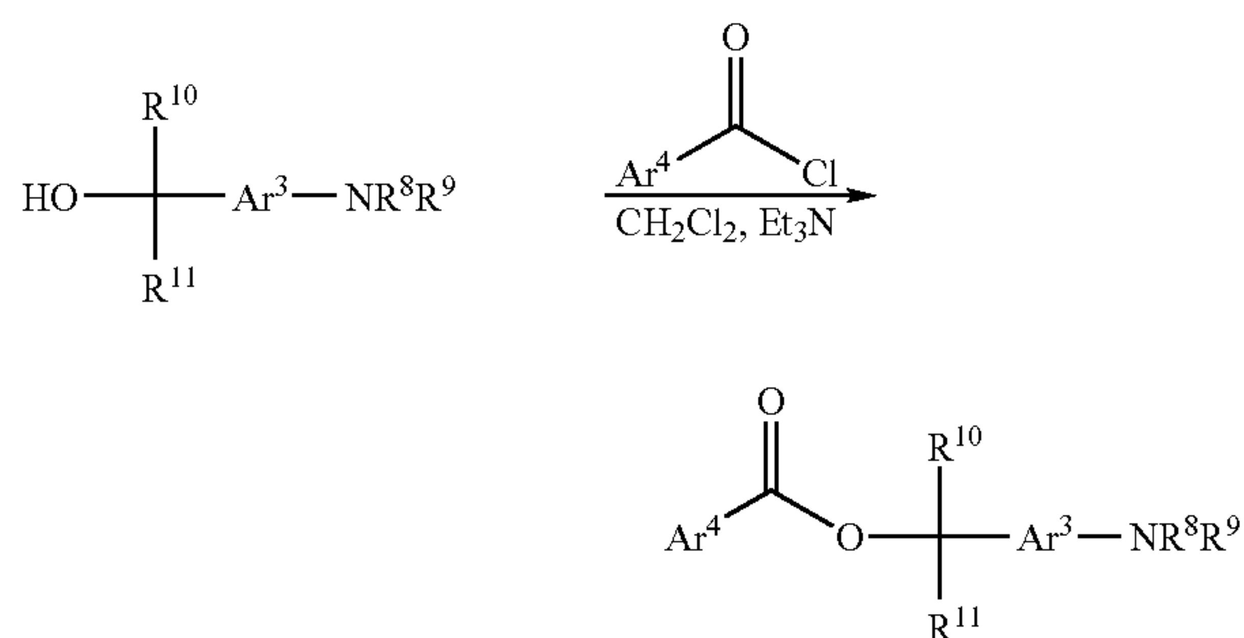
Reaction Scheme 2
