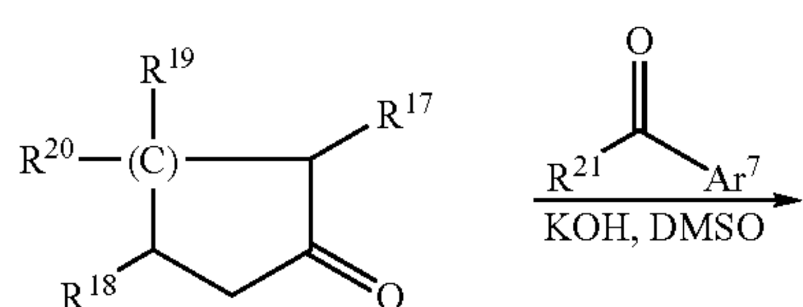
Reaction Scheme 4
