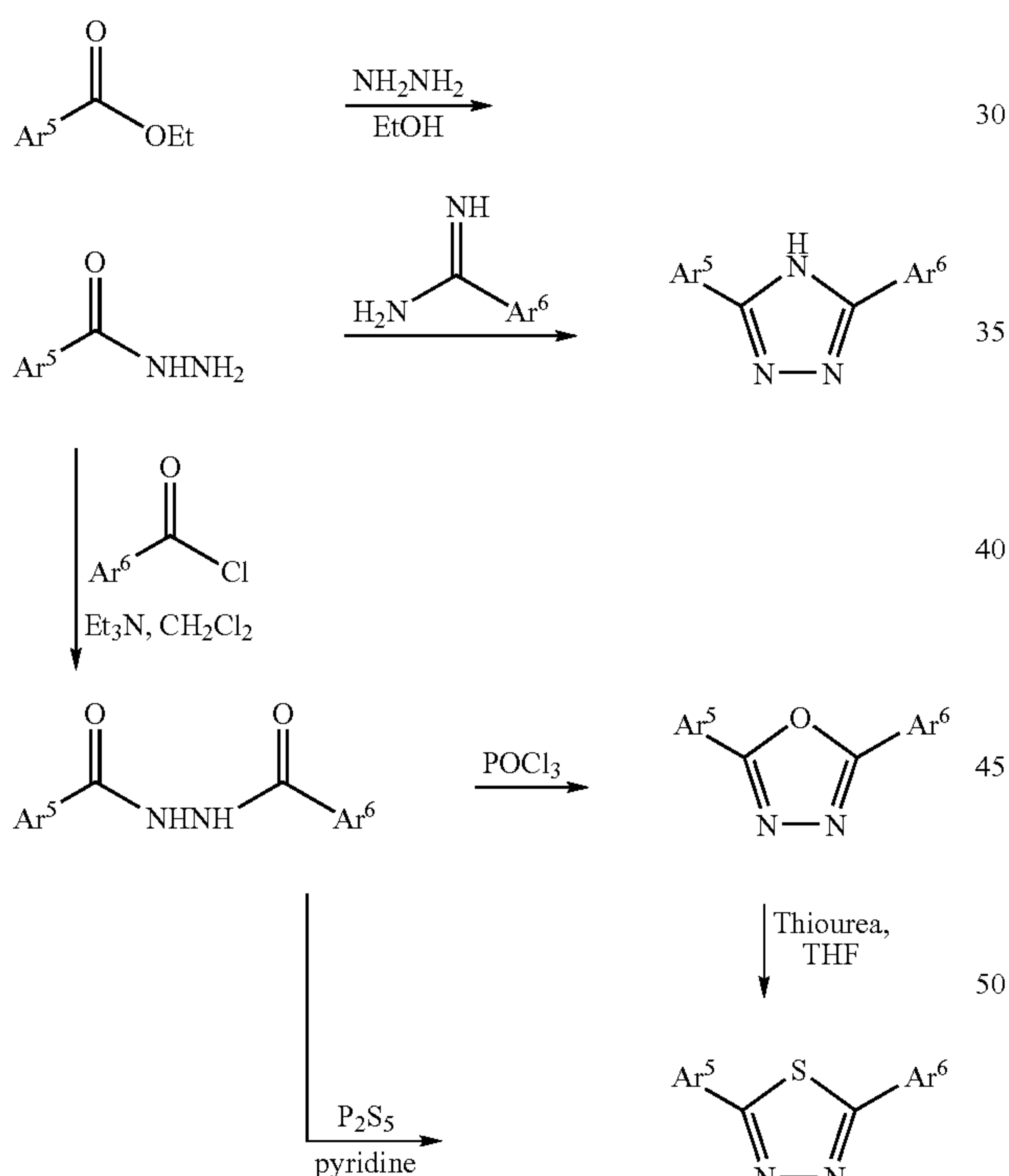
Reaction Scheme 3
