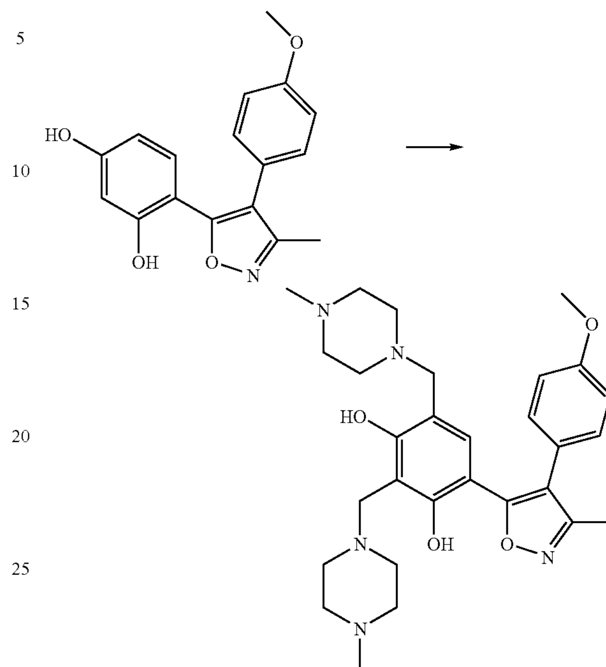
Scheme 2: Mannich reaction
