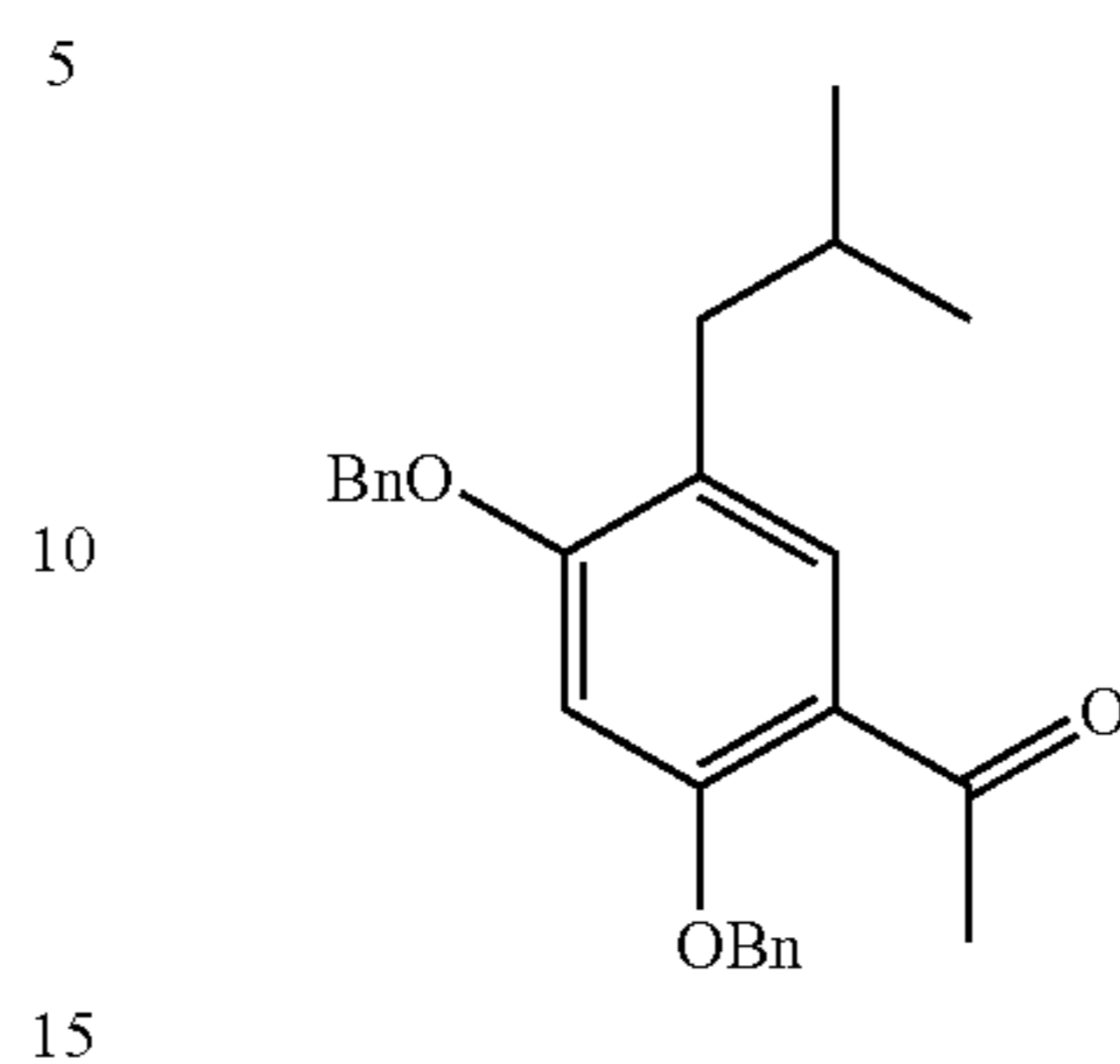
1-(2,4-Bis-benzyloxy-5-isobutyl-phenyl)-ethanone
