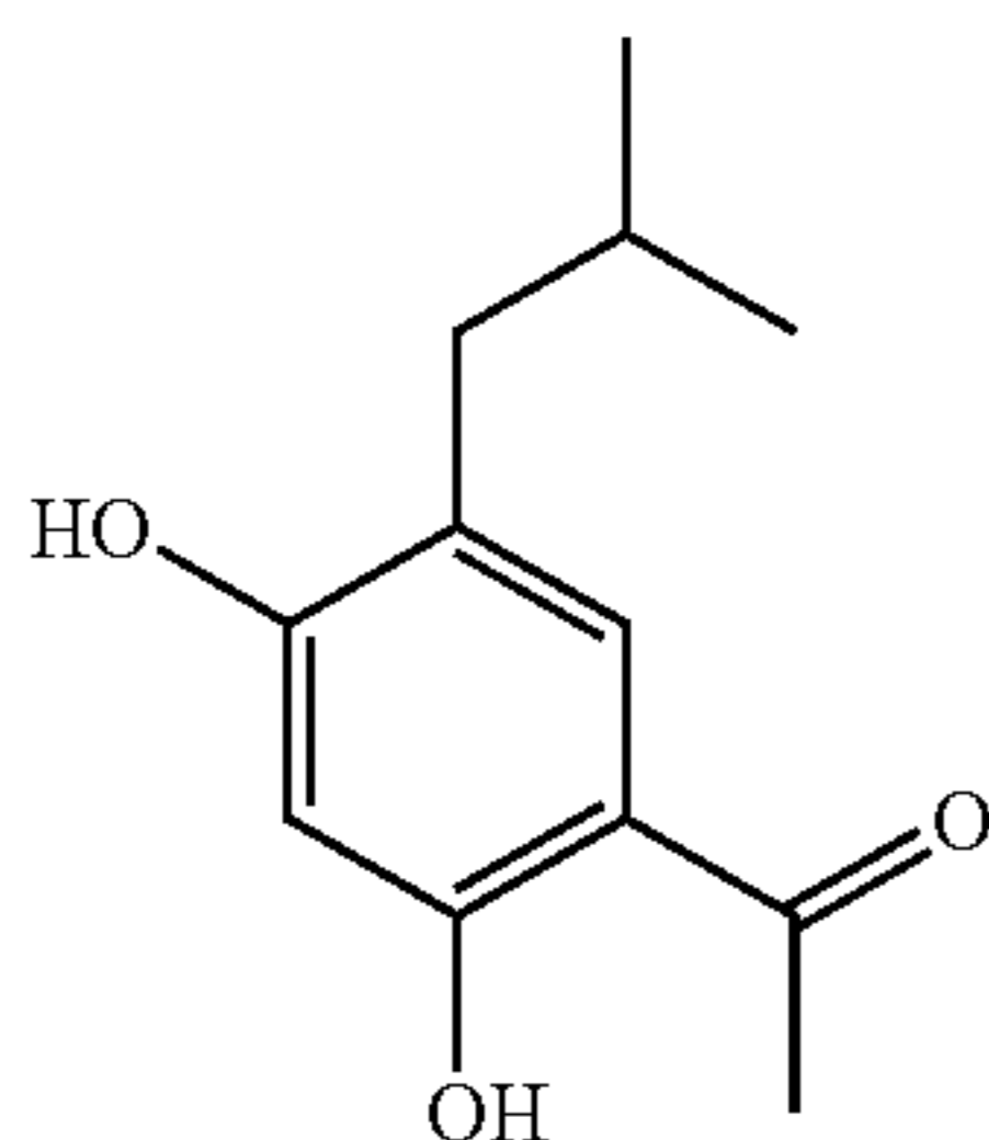
1-(2,4-Dihydroxy-5-isobutyl-phenyl)-ethanone
