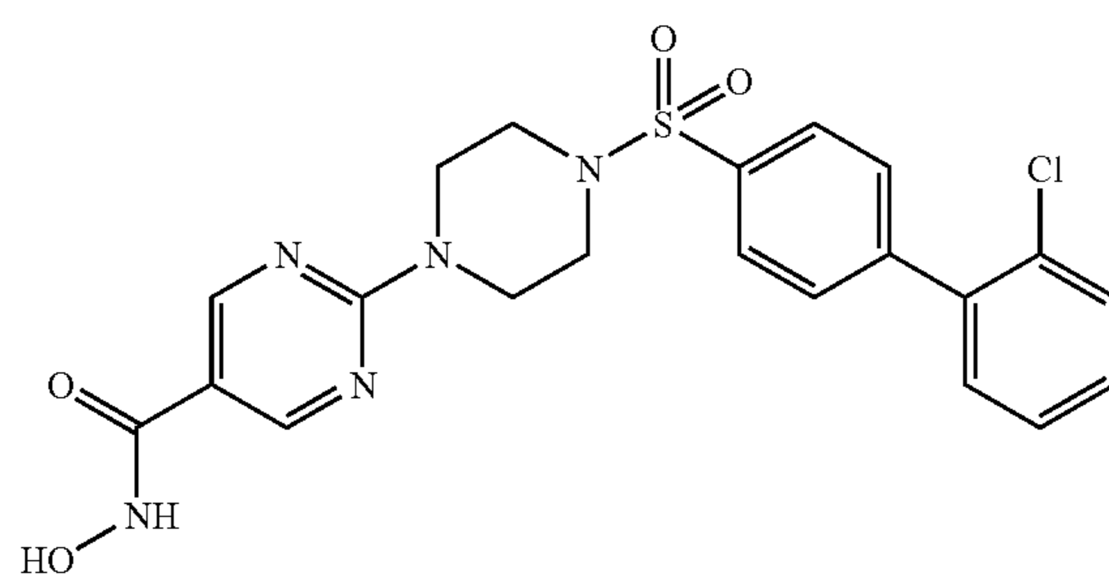
Co. No. 108; Ex. [B16]
