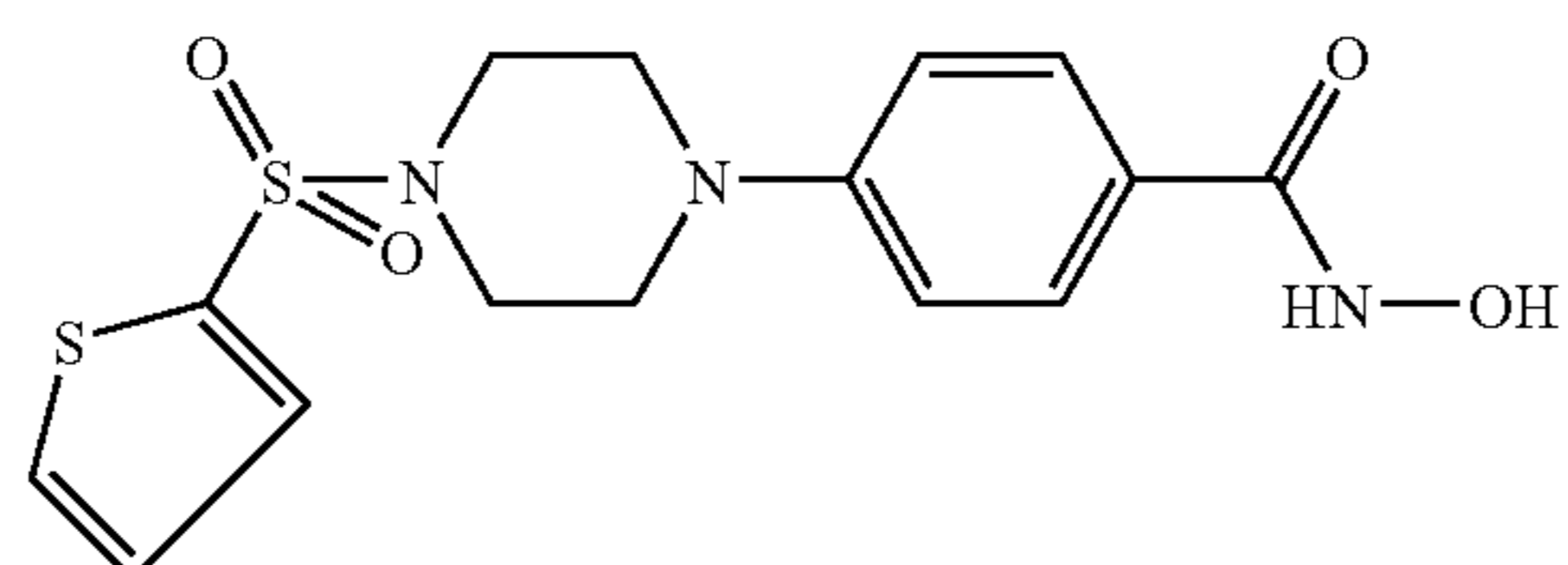
Co. No. 70; Ex. [B1]; mp. 228° C.
