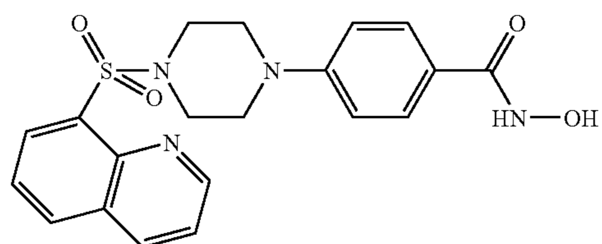
Co. No. 71; Ex. [B1]
