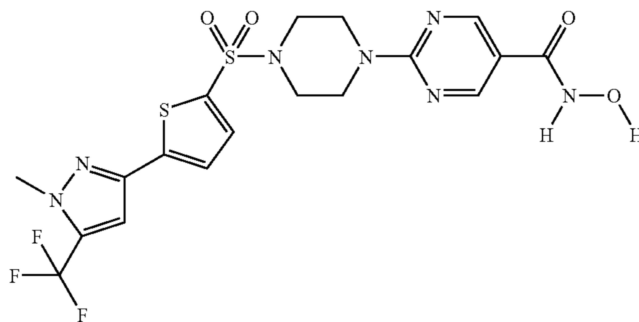
Co. No. 93; Ex. [B15]
