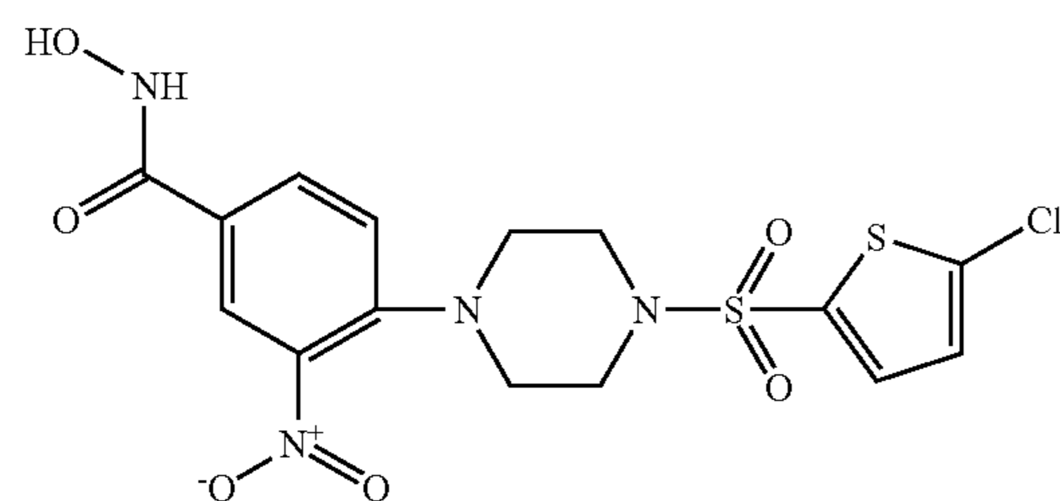
•C 2 HF 3 O 2 (1:1), Co. No. 20; Ex. [B1]; ms.
