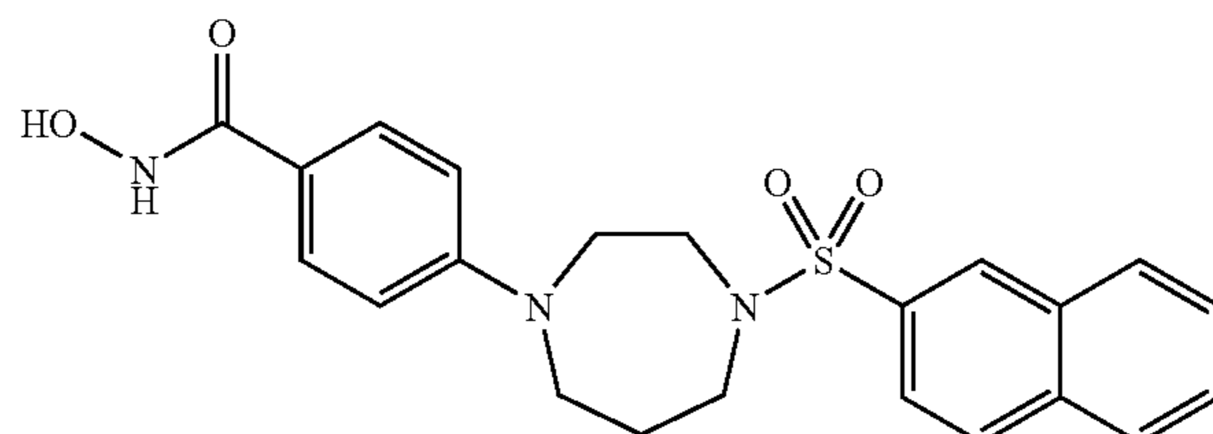
Co. No. 1; Ex. [B2]
