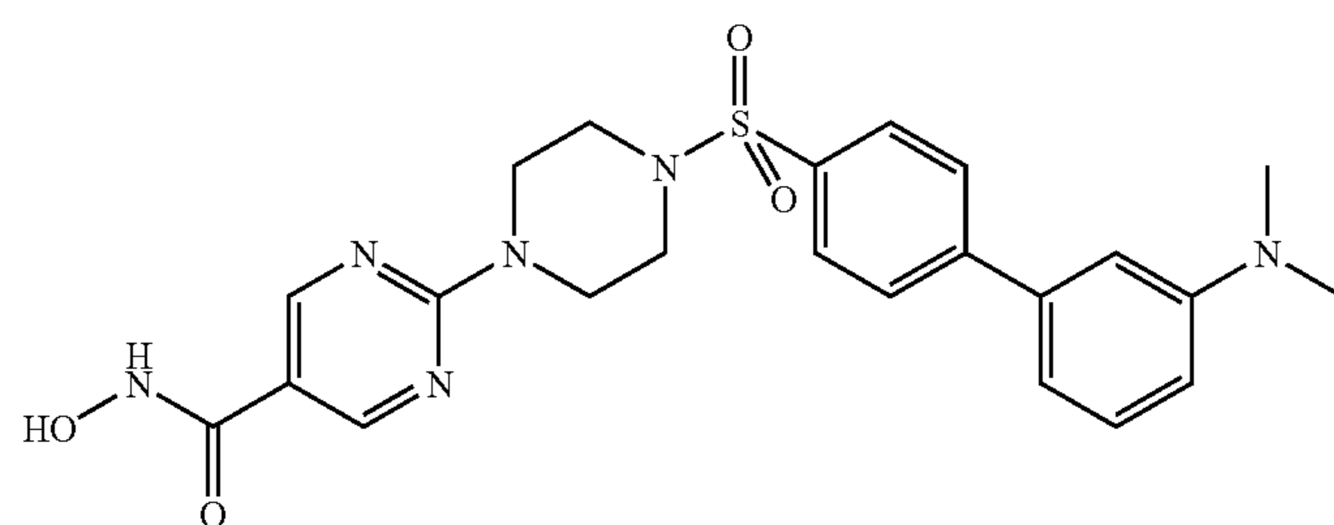
\cdot\text{C}_2\text{HF}_3\text{O}_2 ; Co. No. 135; Ex. [B16]
