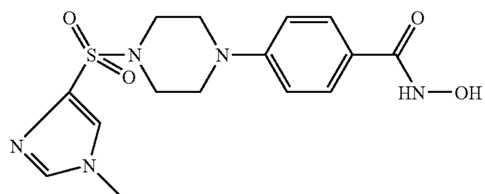
Co. No. 65; Ex. [B1]; mp. 252° C.
