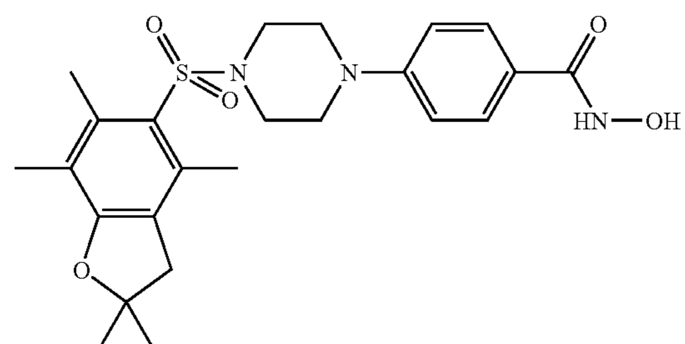
Co. No. 67; Ex. [B1]; mp. 226° C.
