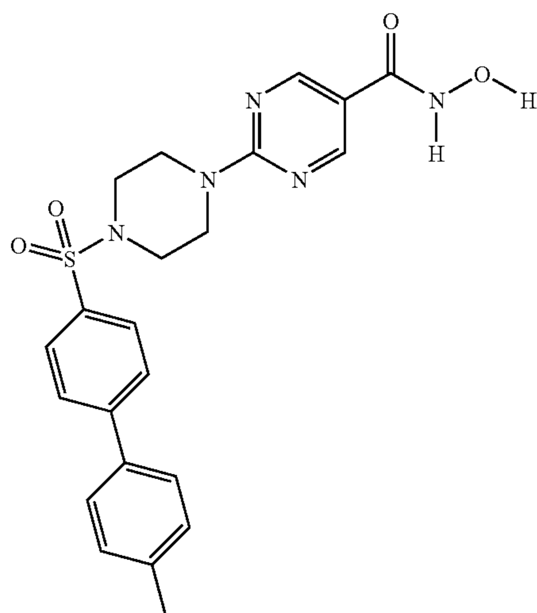
Co. No. 179; Ex. [B32]
