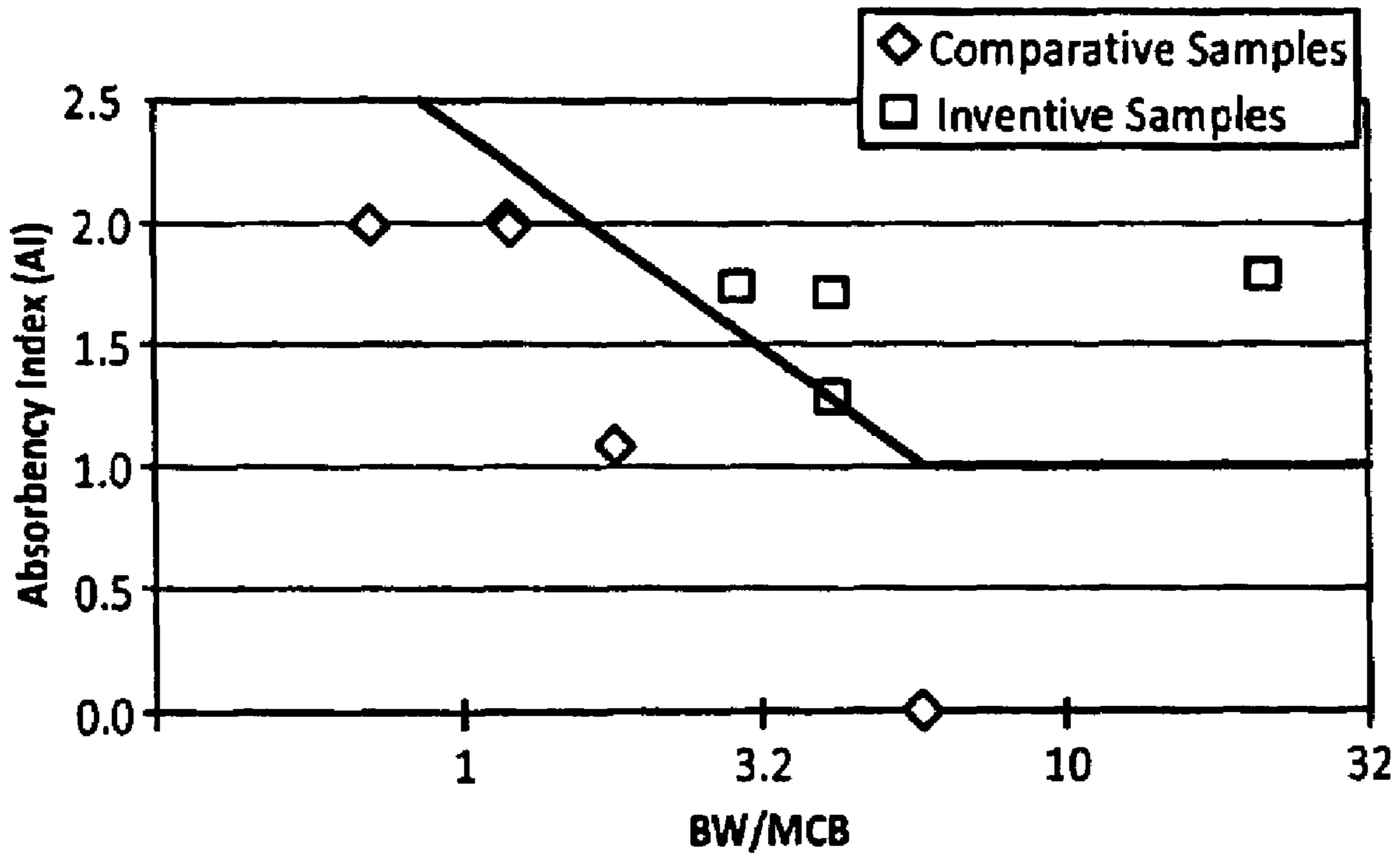
Absorbency vs Drape (thickness \leq 2.5 mm)
