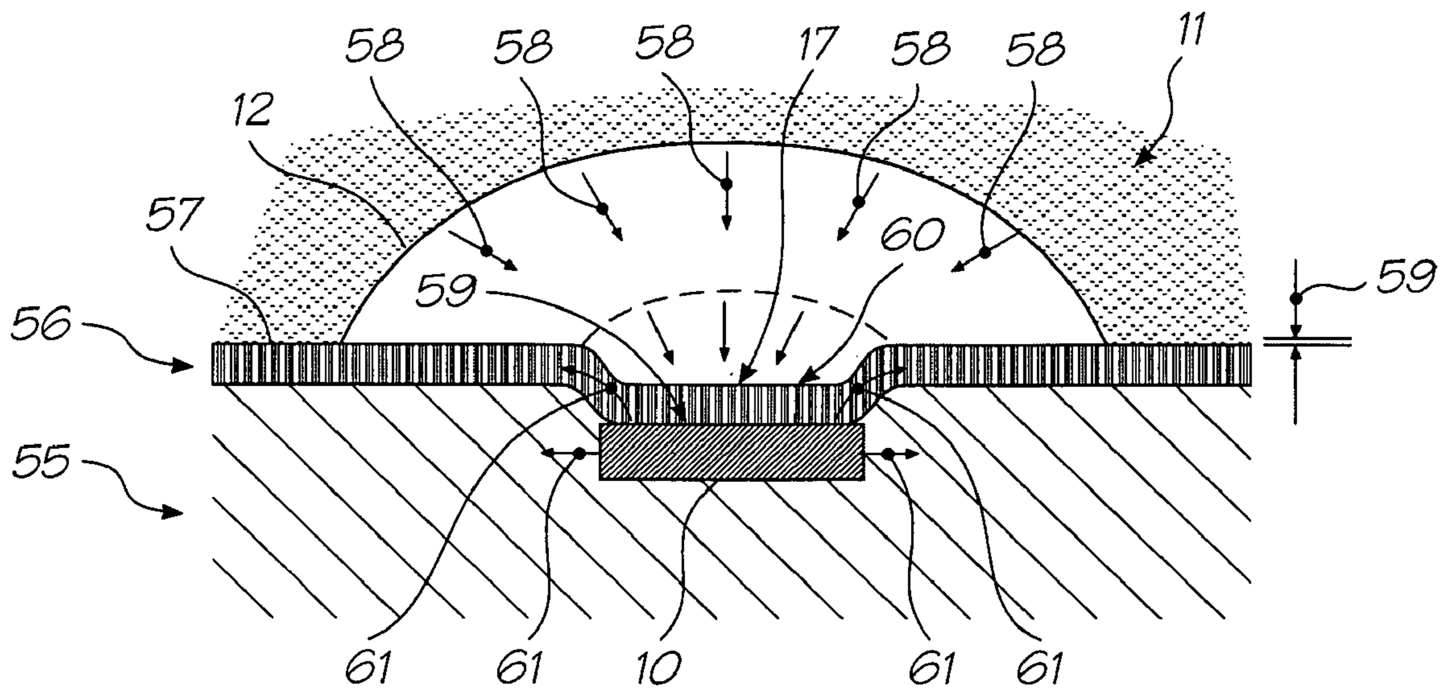
FIG. 47 (PRIOR ART)
