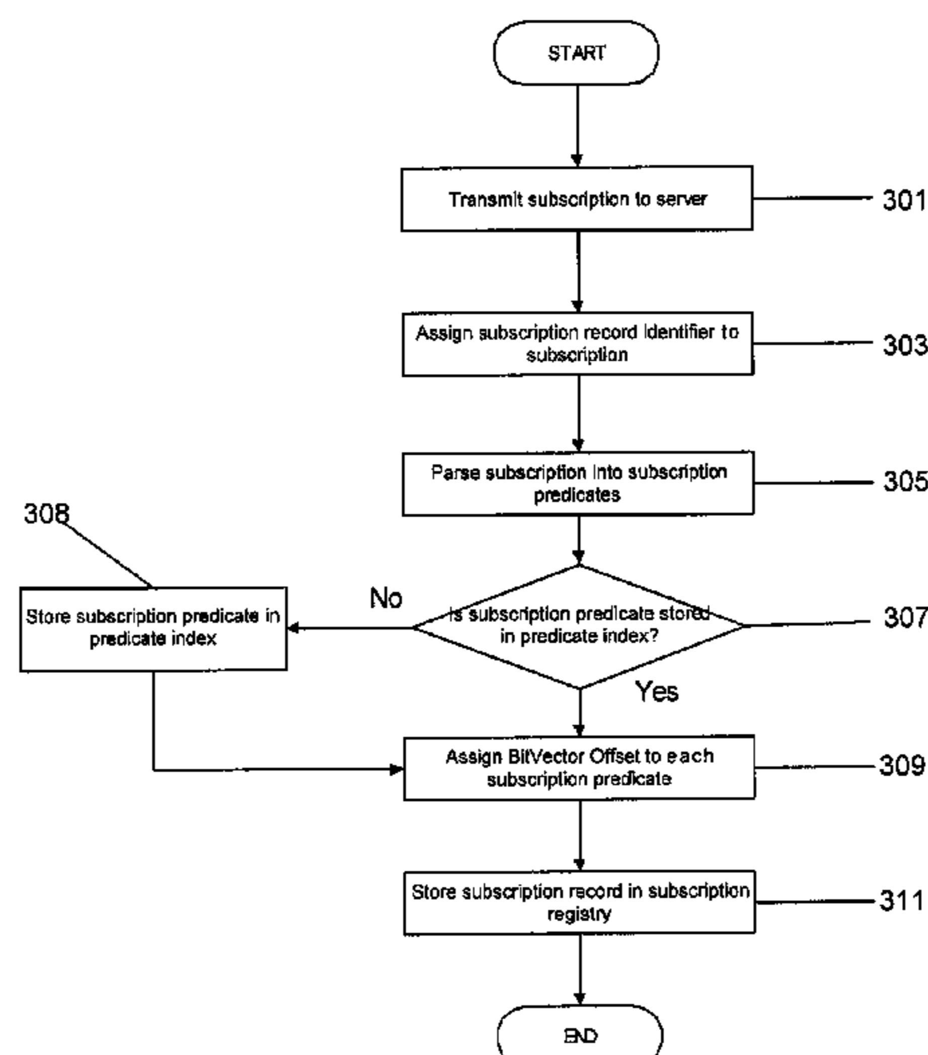
Method 300 for Registering a Subscription
