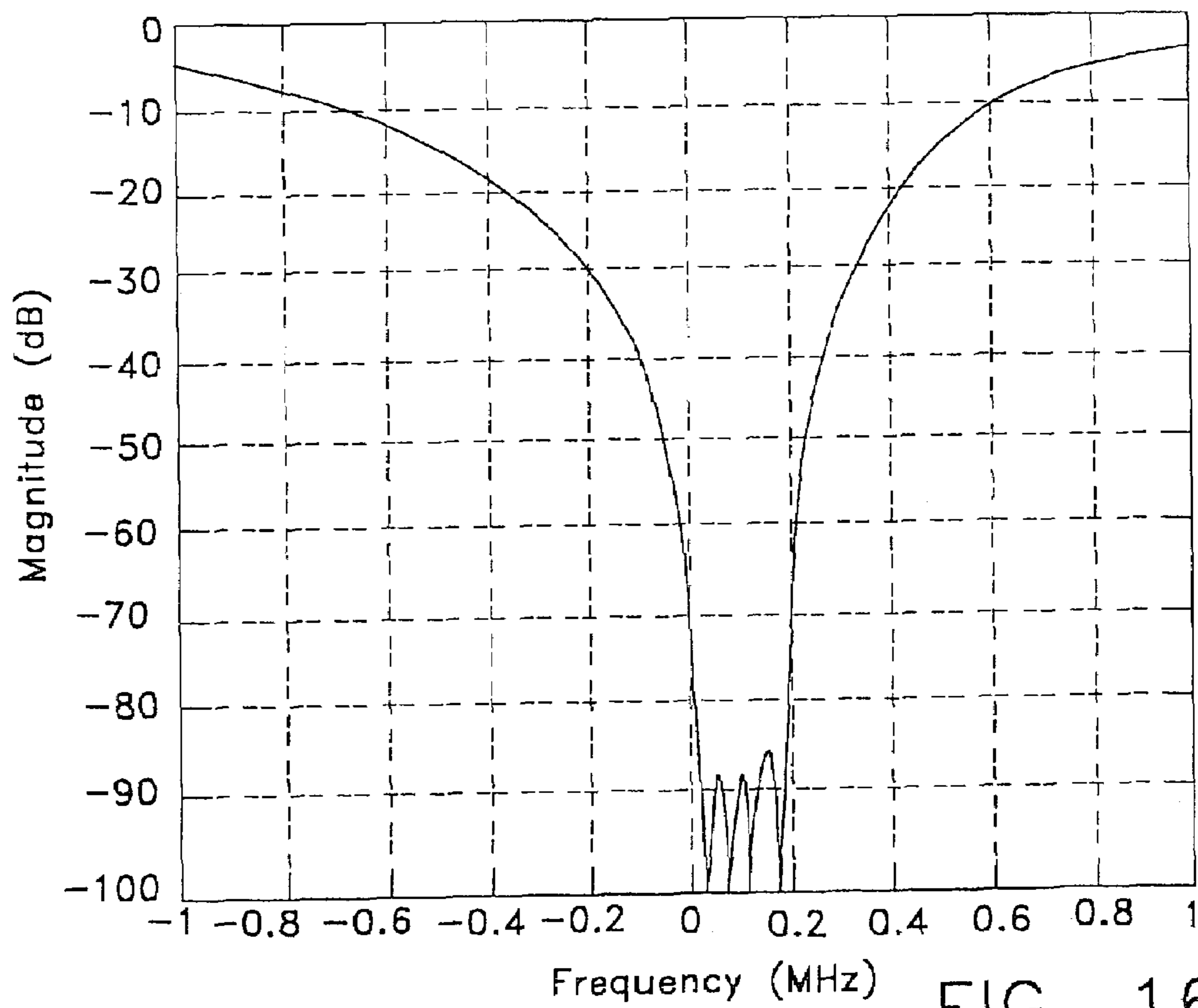
Delta-Sigma ADC Quantization Noise Transfer Function
