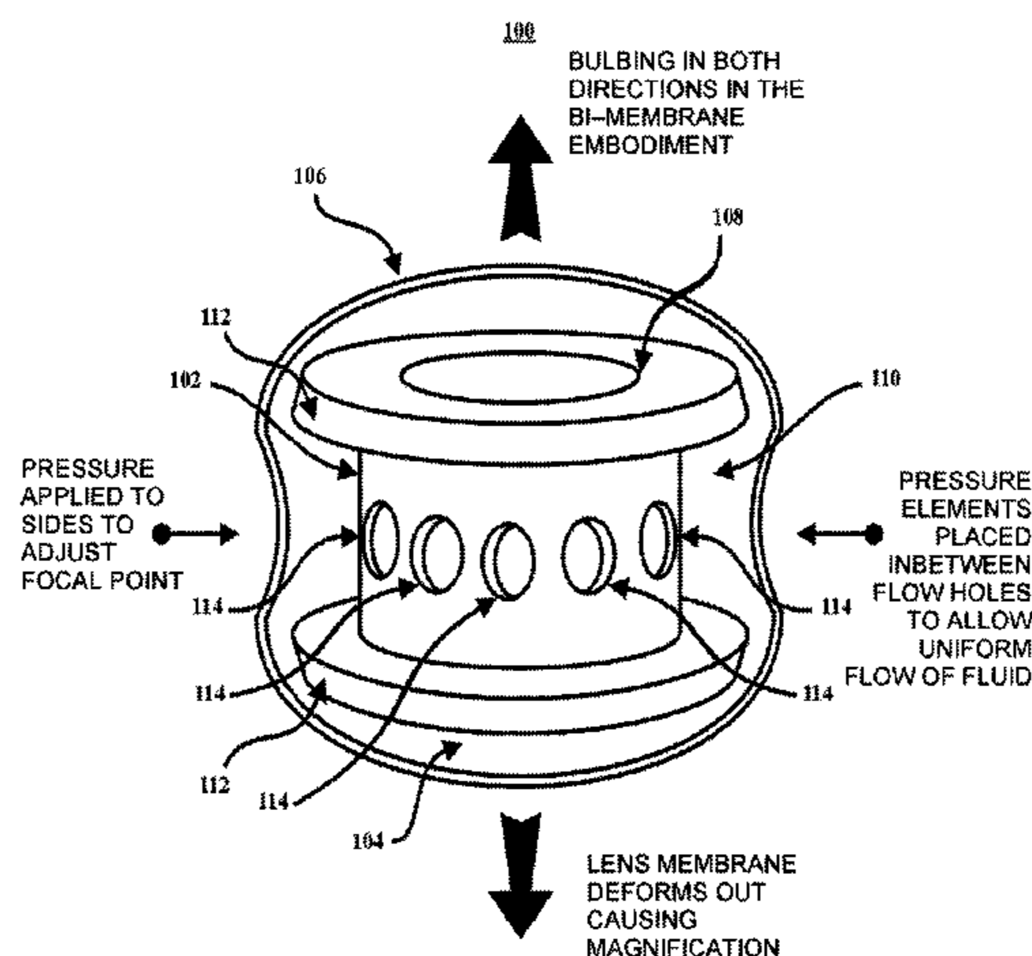
BASIC CONCEPT OF LIQUID LENS IN BI-DIRECTIONAL USE
