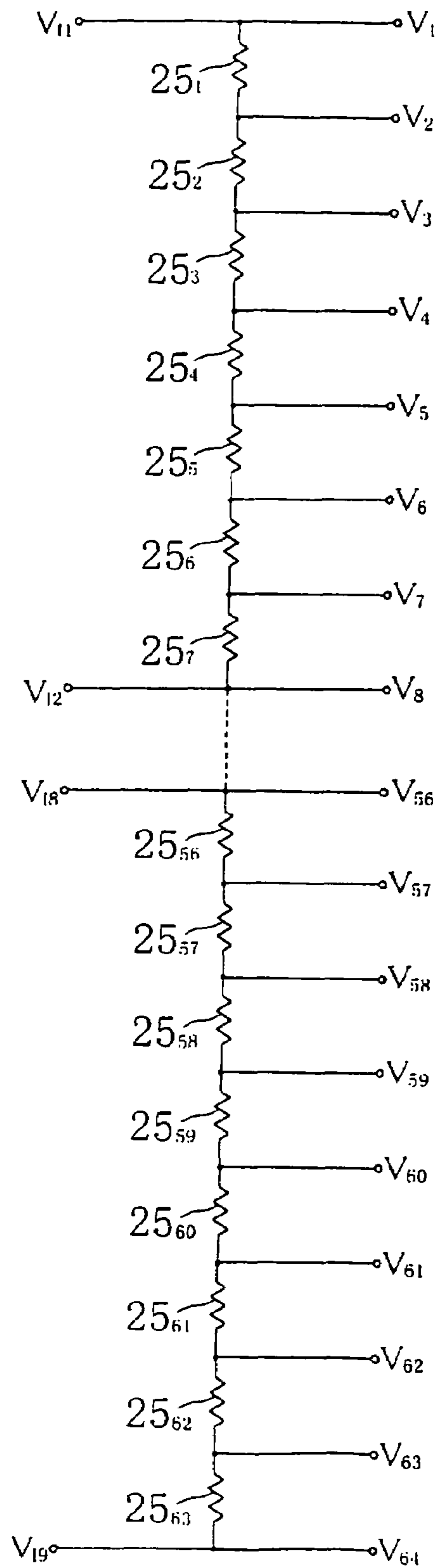
FIG. 5 prior art
