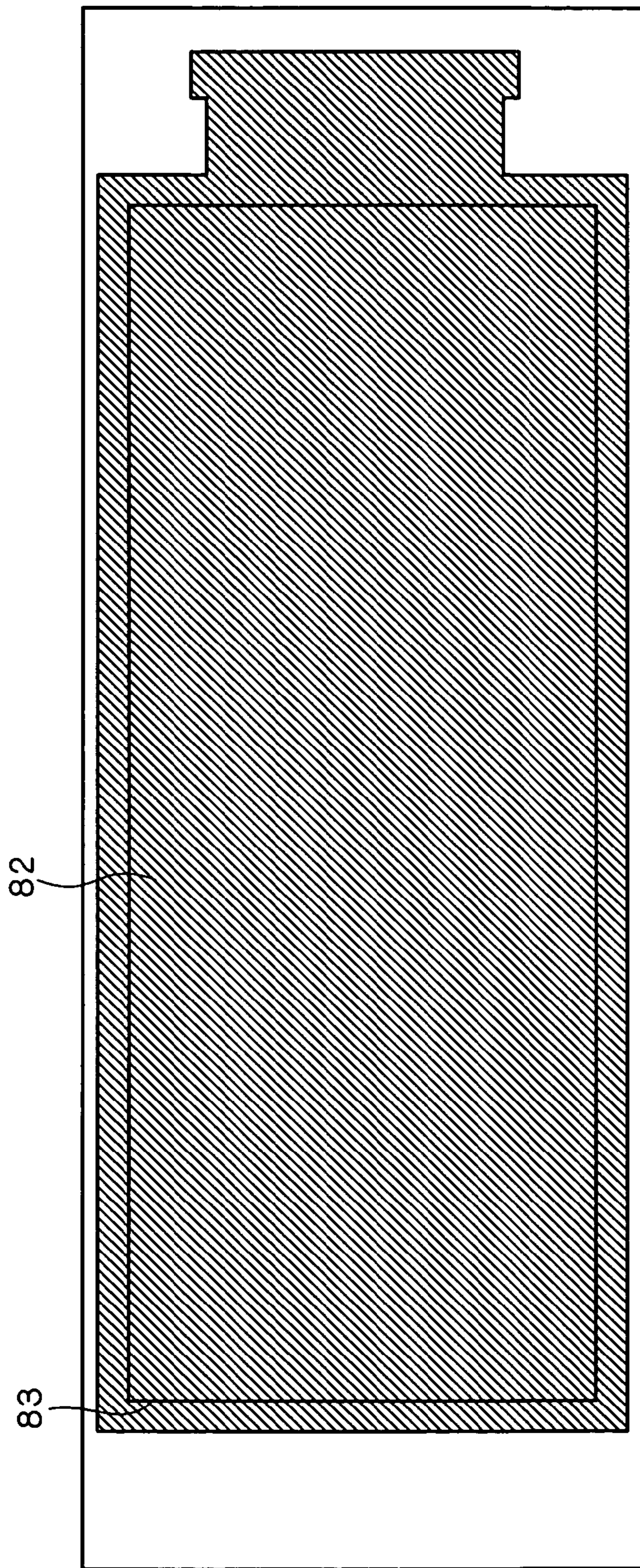
FIFTH METAL WIRING LAYER AND PAD OPENING
