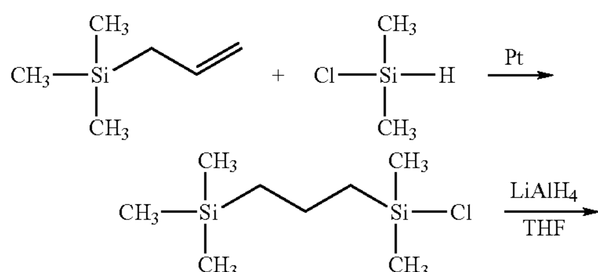
Figure 3 - Reaction Sequence for Preparation of Hydride Intermediate
