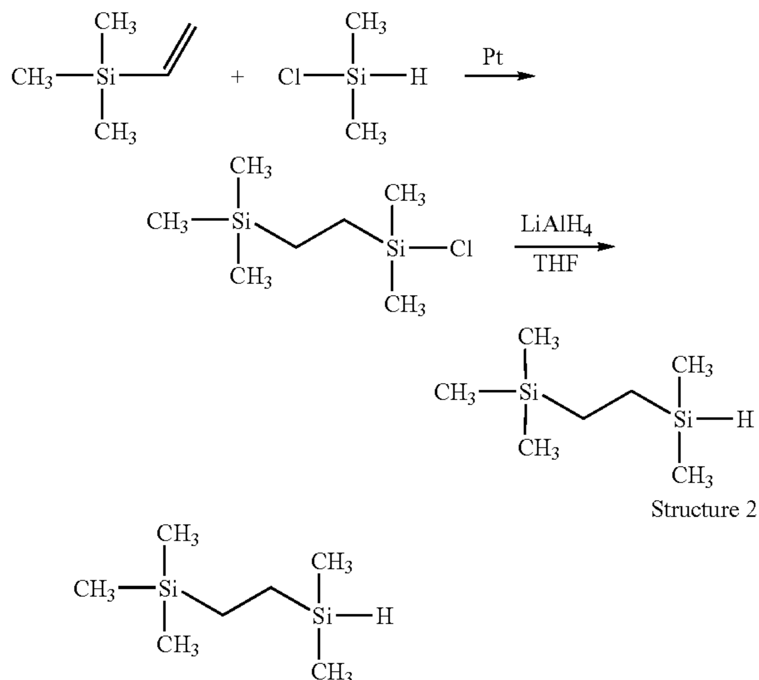
Figure 2 - Reaction Sequence for Preparation of Hydride Intermediate
