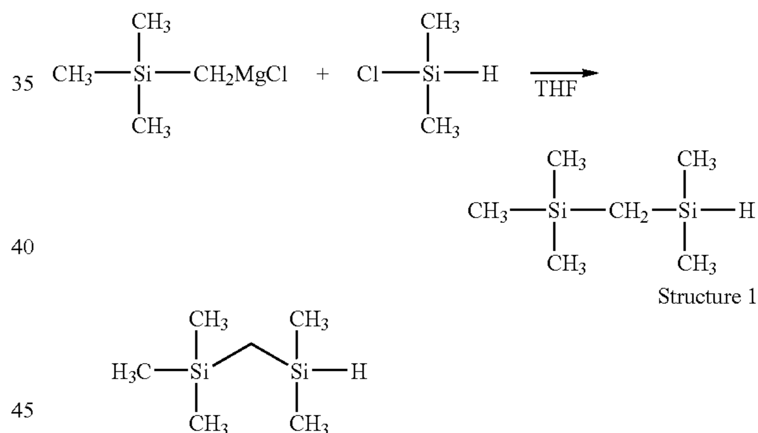
Figure 1 - Reaction Sequence for Preparation of Hydride Intermediate
