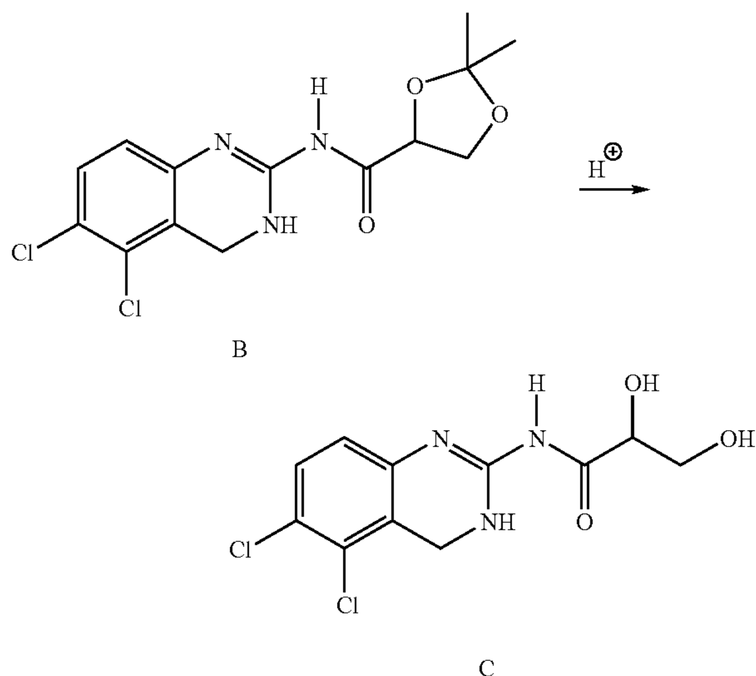
Scheme 3: Hydrolysis of compound B to compound C
