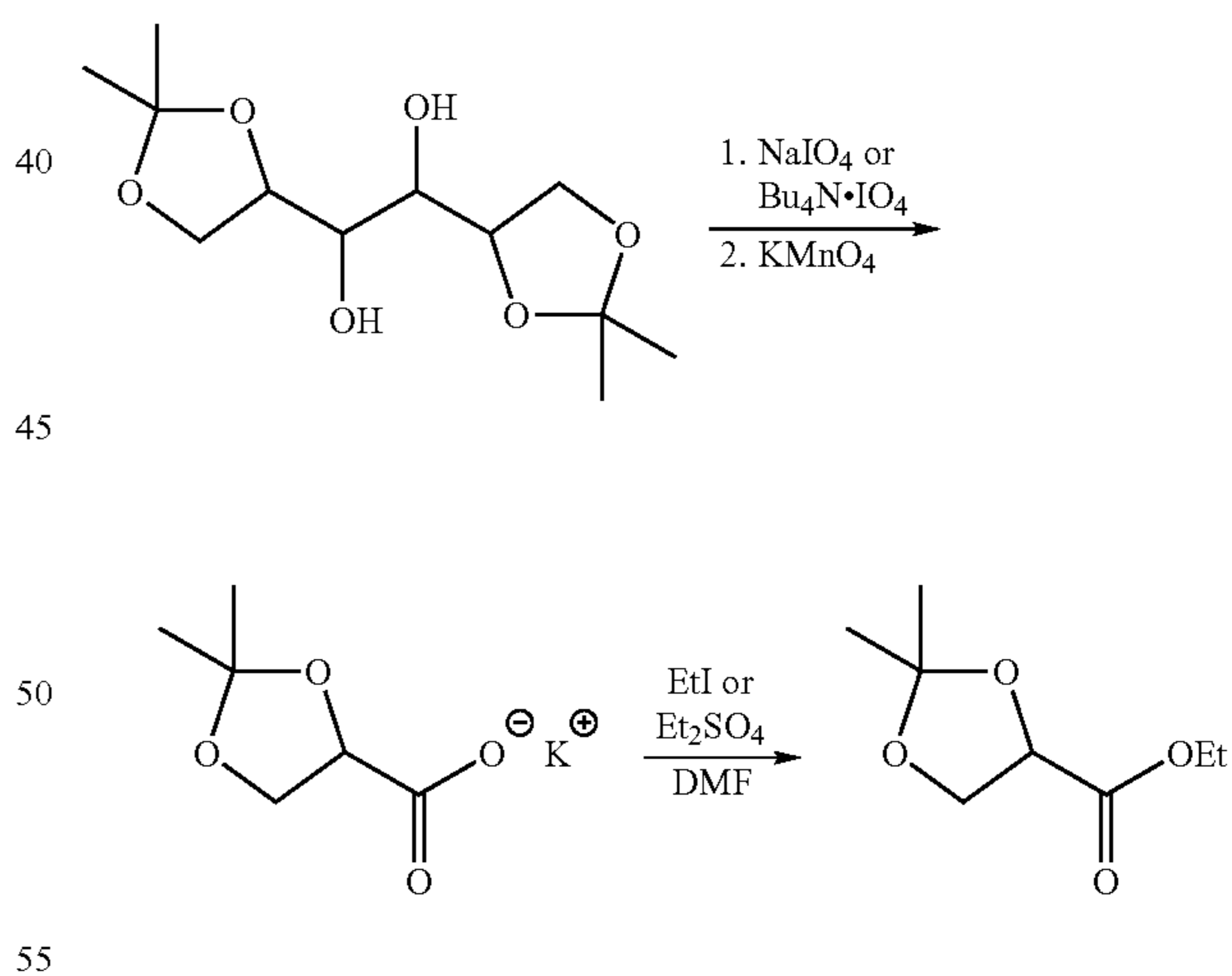
Scheme 2: Syntheses of ethyl 2,3-isopropylidene glycerate
