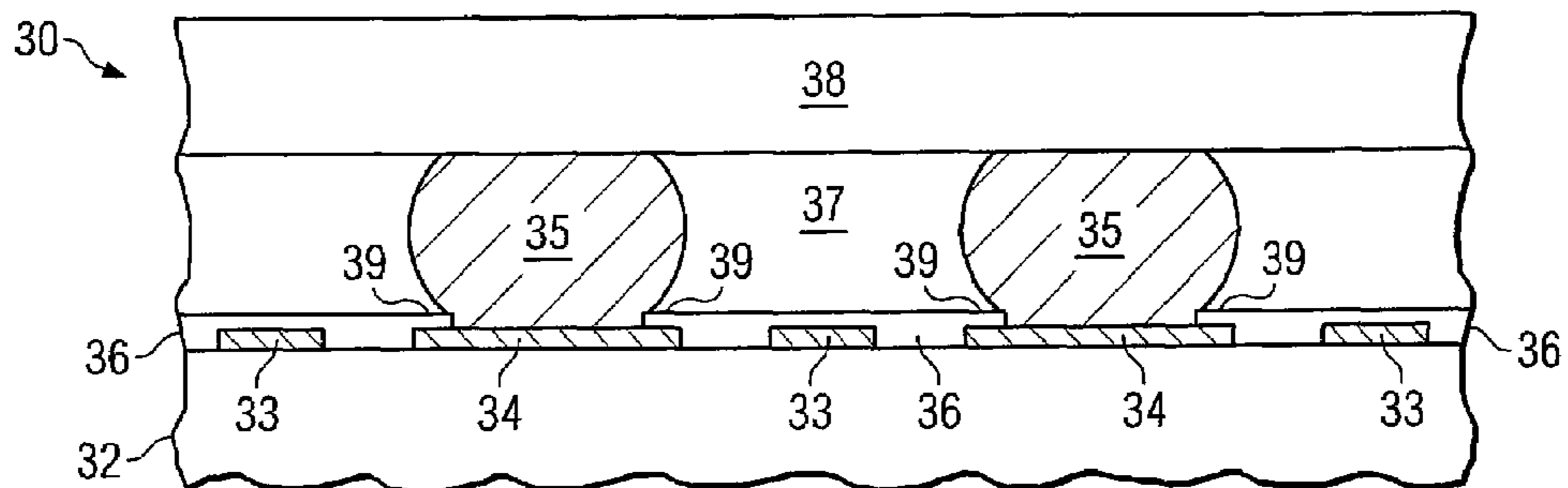
FIG. 3 (PRIOR ART)
