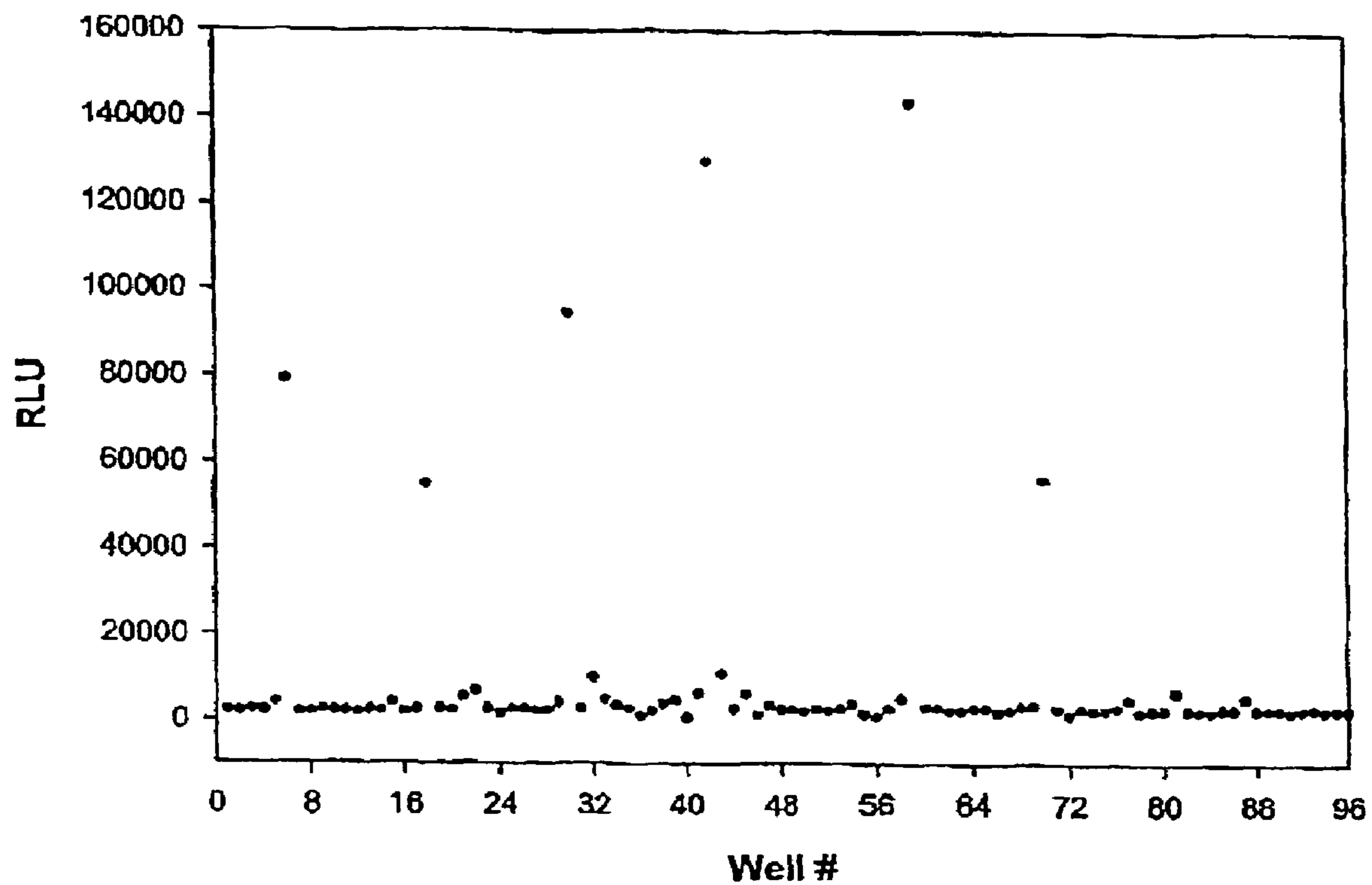
Screening compounds from Plate 6 of the LOPAC library for inhibitors of PKA.
