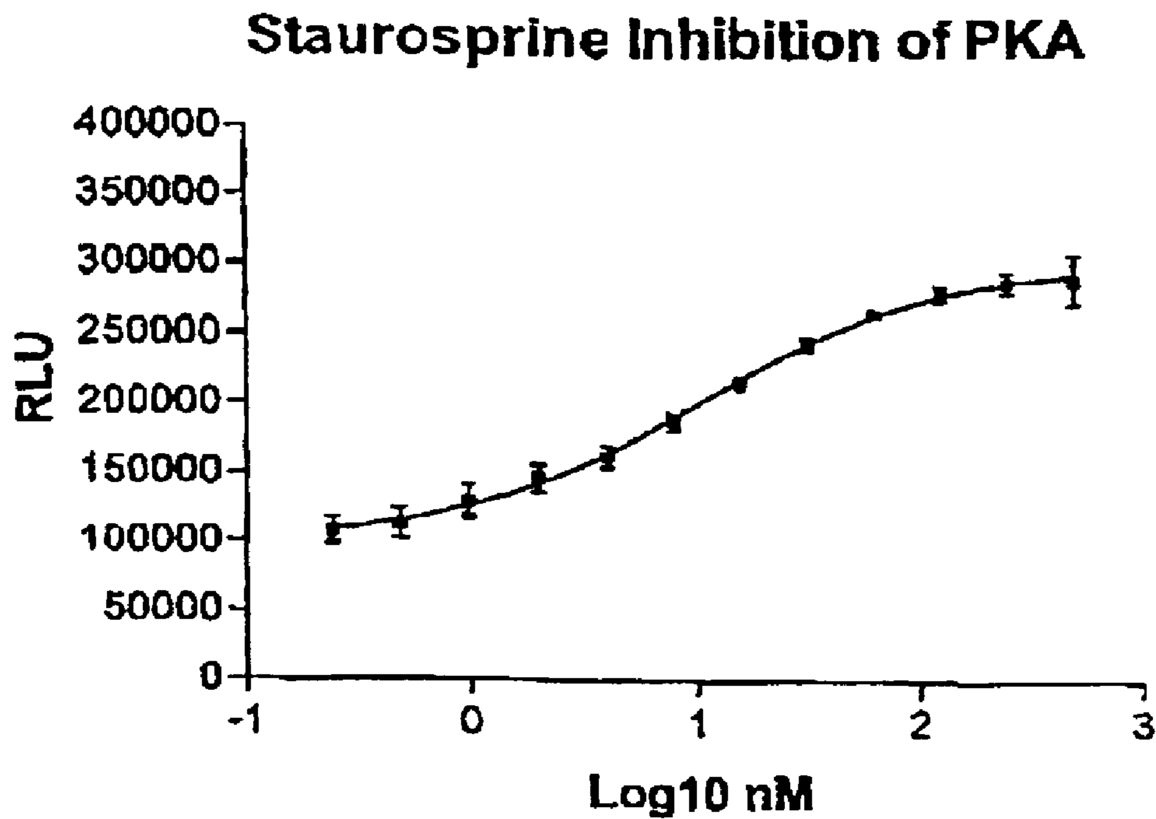
Figure 4 Staurosporine induced inhibition of PKA
