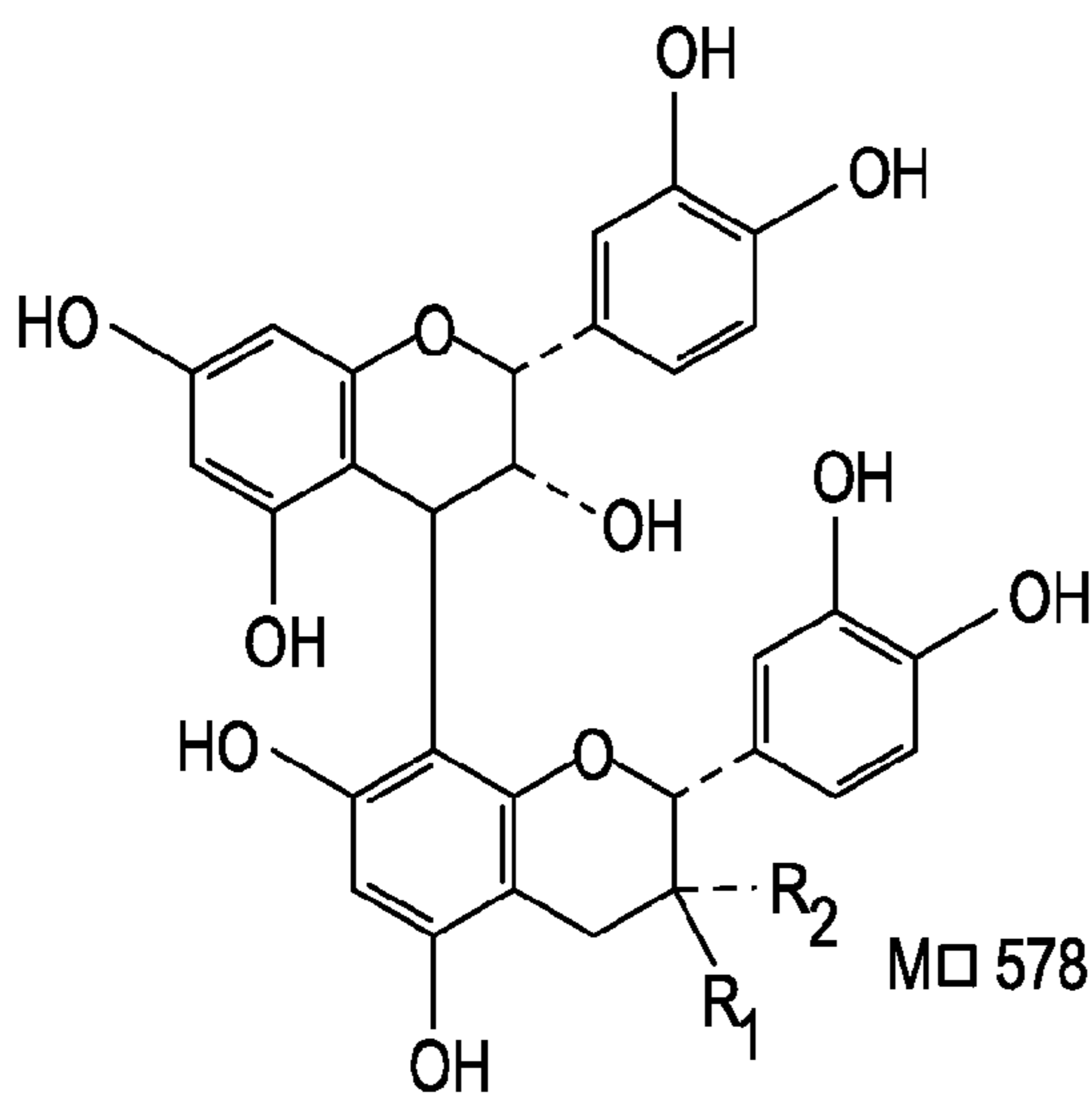
3. R1=OH, R2=H; B-TYPE DIMER 1 4. R1=H, R2=OH; B-TYPE DIMER 2
