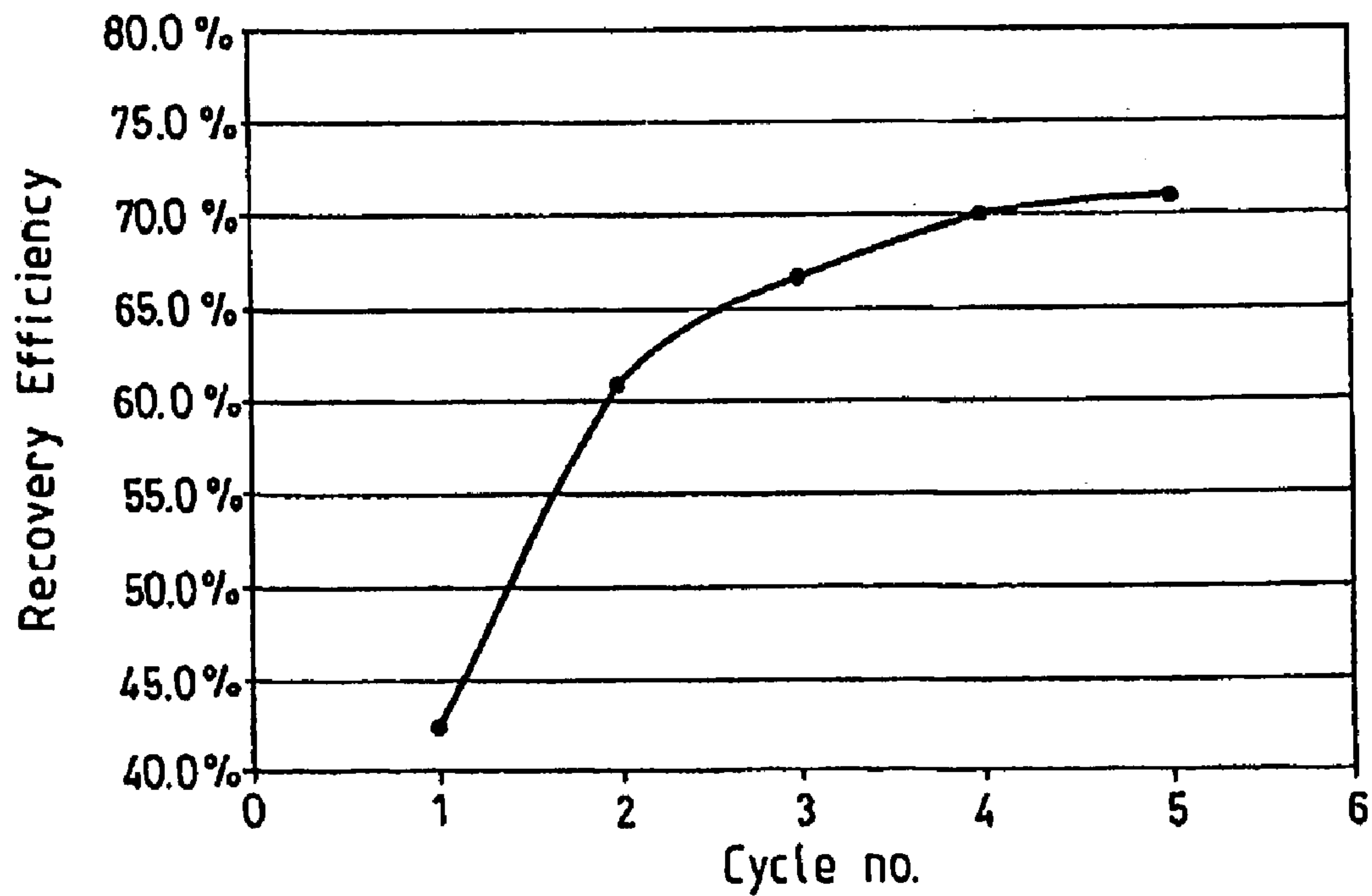
FIG.3 PRIOR ART
