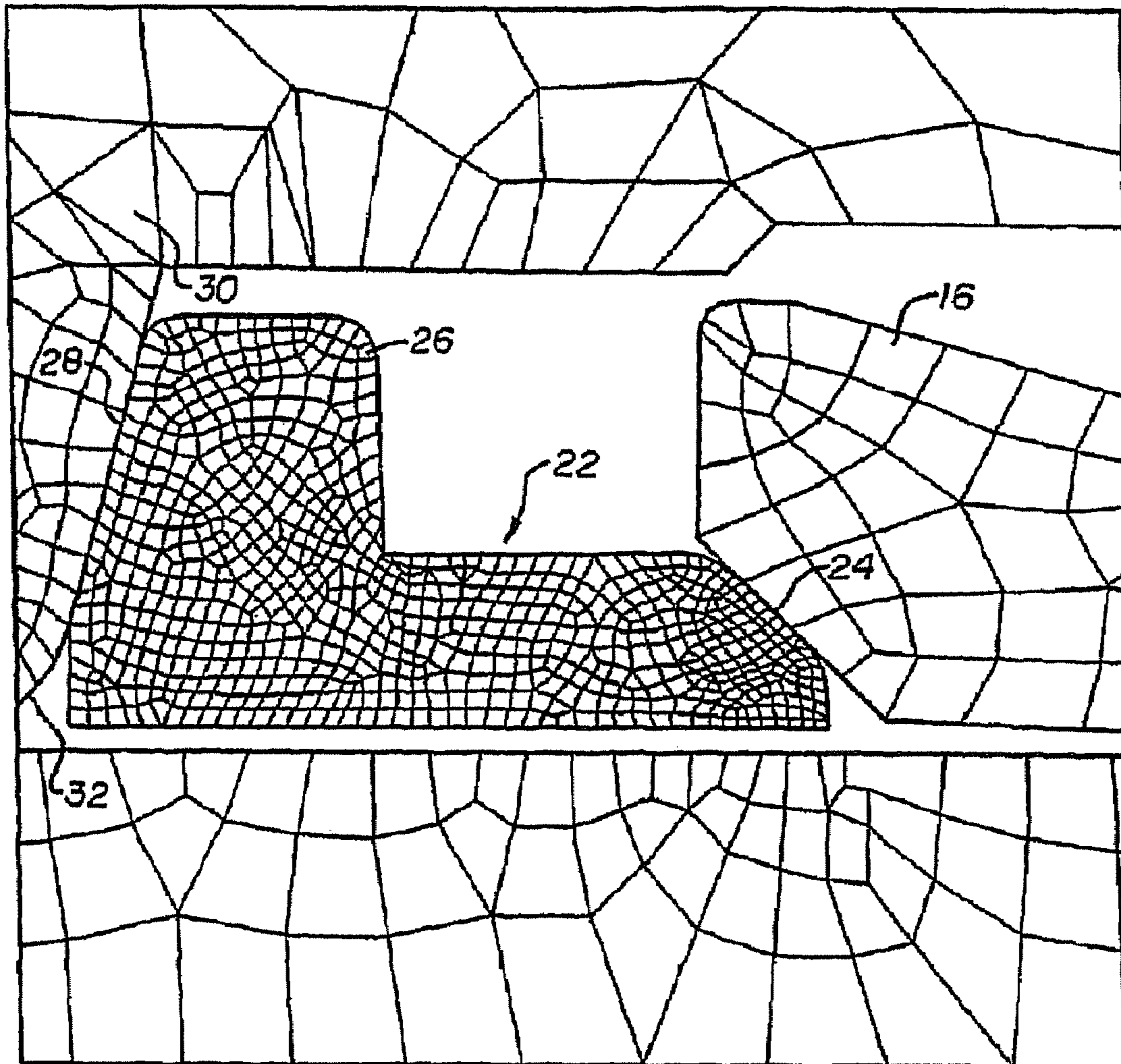
FIG. 6 (PRIOR ART)
